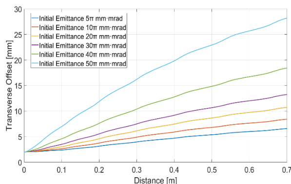
Figure 7: Evolution of transverse RMS bunch size along the longitudinal axis, for various initial emittance injected.
