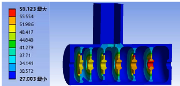
Figure 8: Steady-state temperature distribution in ANSYS simulation.
