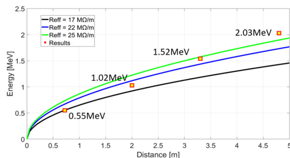
Figure 3: Predesign of different energy schemes.
