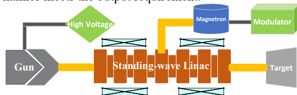
Figure 2: Layout of the designed linac system.
