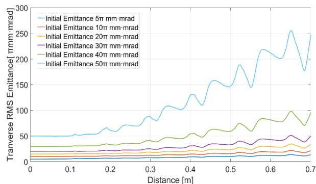
Figure 6: Evolution of transverse RMS emittance along the longitudinal axis, for various initial emittance injected.
