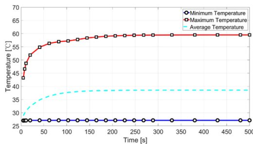
Figure 9: Temporal evolution of the steady-state temperature.
