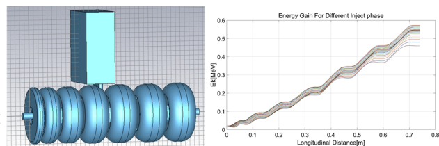
Figure 4: Vacuum model of the accelerating structure in CST (left) and kinetic energy evolution longitudinally(right).
