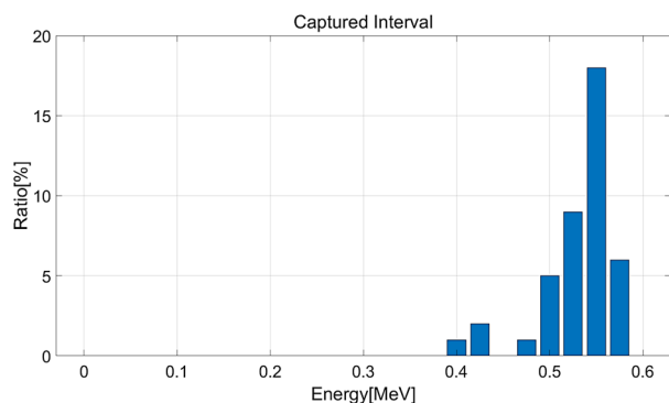
Figure 5: Energy distribution of the captured electrons.
