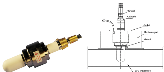
Figure 1: CW L-band (915 MHz) magnetron.
