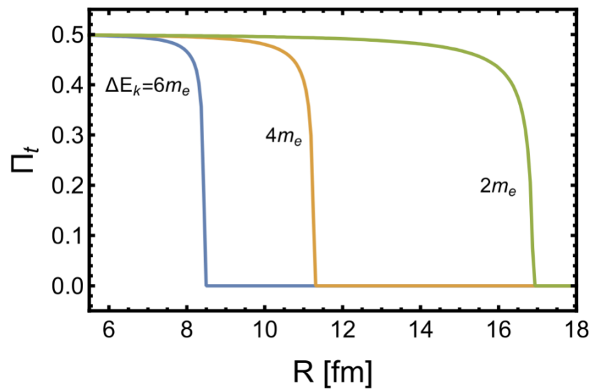
Figure 3. (Color online) Tunneling probability for the positron as a function of the relative distance of the two C ions and E_{c.m.} = 9.4 MeV and different values of \Delta E_k .
