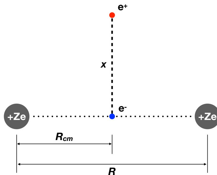
Figure 1. (Color online) Geometry of the pair production.
