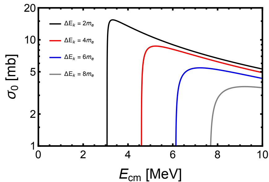
Figure 4. (Color online) Upper limit for the integrated cross-section for e^+e^- production in ^{12}\text{C}+^{12}\text{C} scattering below the Coulomb barrier for different values of \Delta E_k . We stress that \Delta E_k \geq 0 .
