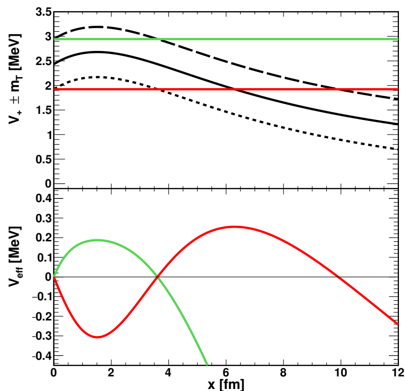
Figure 2. (Color online) An illustrative example when V_{eff}(R, 0) = 0 . In the bottom panel we plot V_{eff} vs. x and the corresponding potential with full line ( \pm m_T = m_e —top panel, dashed and dotted lines) seen by the positron. The calculations are performed for ^{12}\text{C}+^{12}\text{C} collisions.
