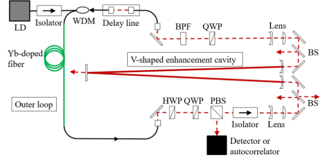
Figure 2: Schematic of the pulsed fiber laser oscillator with the self-resonating enhancement cavity.
