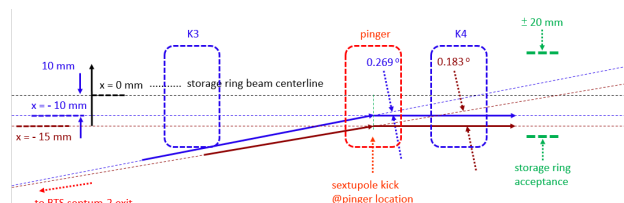
Figure 2: The proposed sextupole injection strength required at pinger location. The pinger will be re-installed at section-8 in September leaving the ceramic chamber for MIK and sextupole injection test-run.
