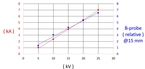
Figure 8: The measured pulsed drive-current and the response of \hat{B} -probe at kA region.
