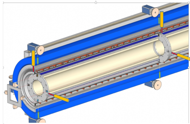
Figure 4: Isometric view of washer stack installed within bore of a 1 T superconducting solenoid.
