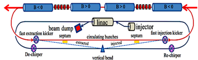
Figure 2: Configuration for bunched-beam electron cooling of ion bunches in JLEIC.
