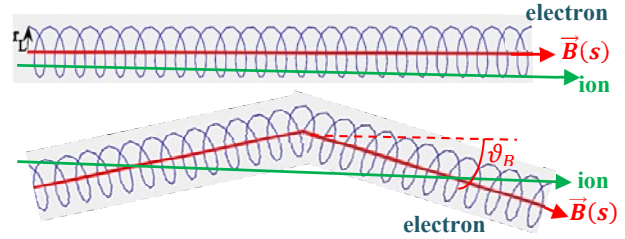
Figure 1: Schematic effect of magnetic field alignment on magnetized cooling: a) close alignment of \vec{B} with ion beam; b) \vec{B} misaligned so the spiraling electrons heat rather than cool the ion beam.
