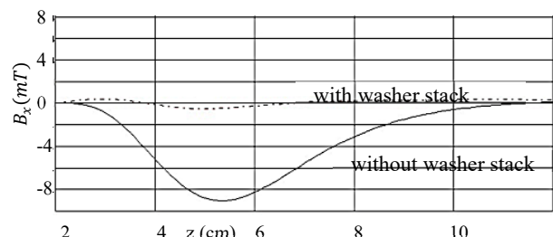
Figure 5: Transverse field B_x(z) along the solenoid axis when one turn of the solenoid is displaced in \hat{x} direction.
