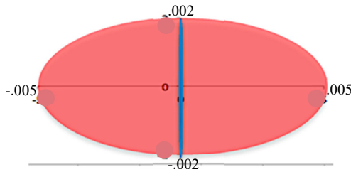
Figure 3: Rest-frame velocity distributions of the electrons (blue) and ions (red) in JLEIC. (from Ref. 5).
