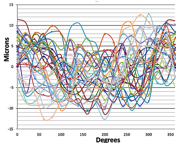
Figure 7: Metrology of the sequence of 30 washers in the compressed washer stack.
