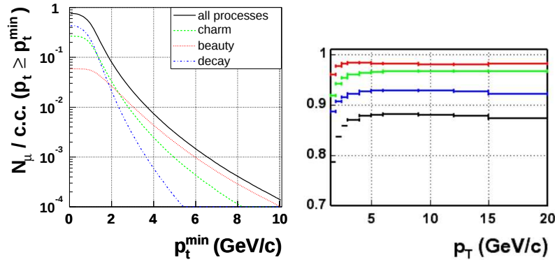
Fig. 3. Left: Number of muons above a threshold p_t^{\min} per central Pb–Pb collision (5% centrality) detected in the muon spectrometer including the trigger cut-off p > 1 GeV/ c . Right: Efficiency for the detection of single muons. Lines refer, from top to bottom, to: trigger, acceptance, tracking, total.
