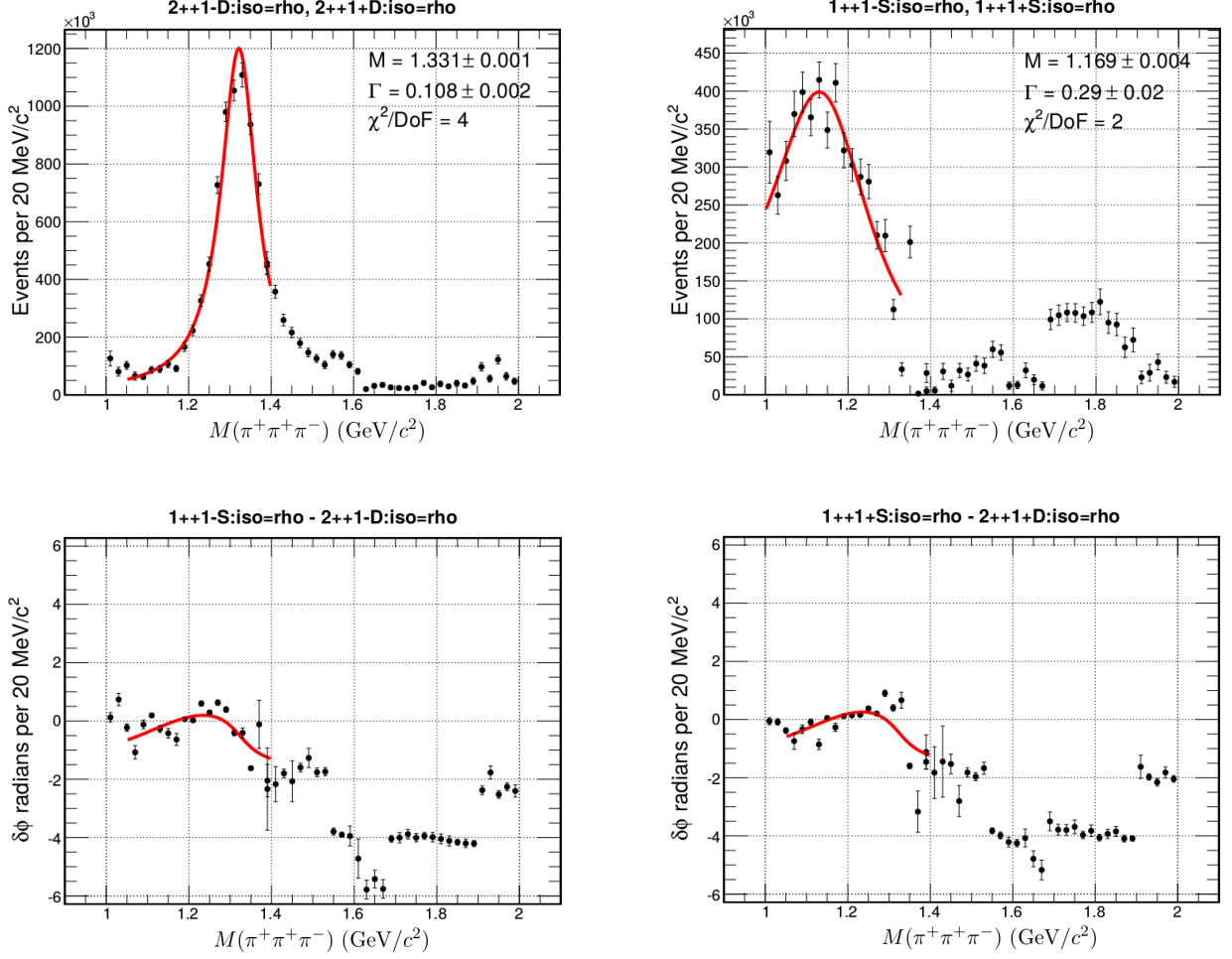
Figure 9.7: For the \gamma p \rightarrow n \pi^+ \pi^+ \pi^- reaction: on the top row is the combined intensity for the two reflectivities M^\epsilon = 1^\pm for the partial waves: 2^{++}1^\pm[\rho(770)\pi]_D and 1^{++}1^\pm[\rho(770)\pi]_S . The two intensities have been fitted with a mass dependent BW function. The bottom row shows the the phase difference of the 2^{++}[\rho(770)\pi]_D wave against 1^{++}[\rho(770)\pi]_S wave for the two different reflectivities. The red curve is a plot of BW phase difference with the parameters obtained by fitting the intensities.
