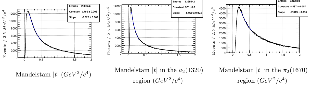
Figure 5.5: \gamma p \rightarrow n\pi^+\pi^+\pi^- : Exponential fits to the |t| distribution for the full 3 \pi mass range ( left plot ), for the low 3 \pi mass region ( center plot ) and for the high 3 \pi mass region ( right plot ). The events showed have the \theta_{lab} cut but not the low t' selection.
