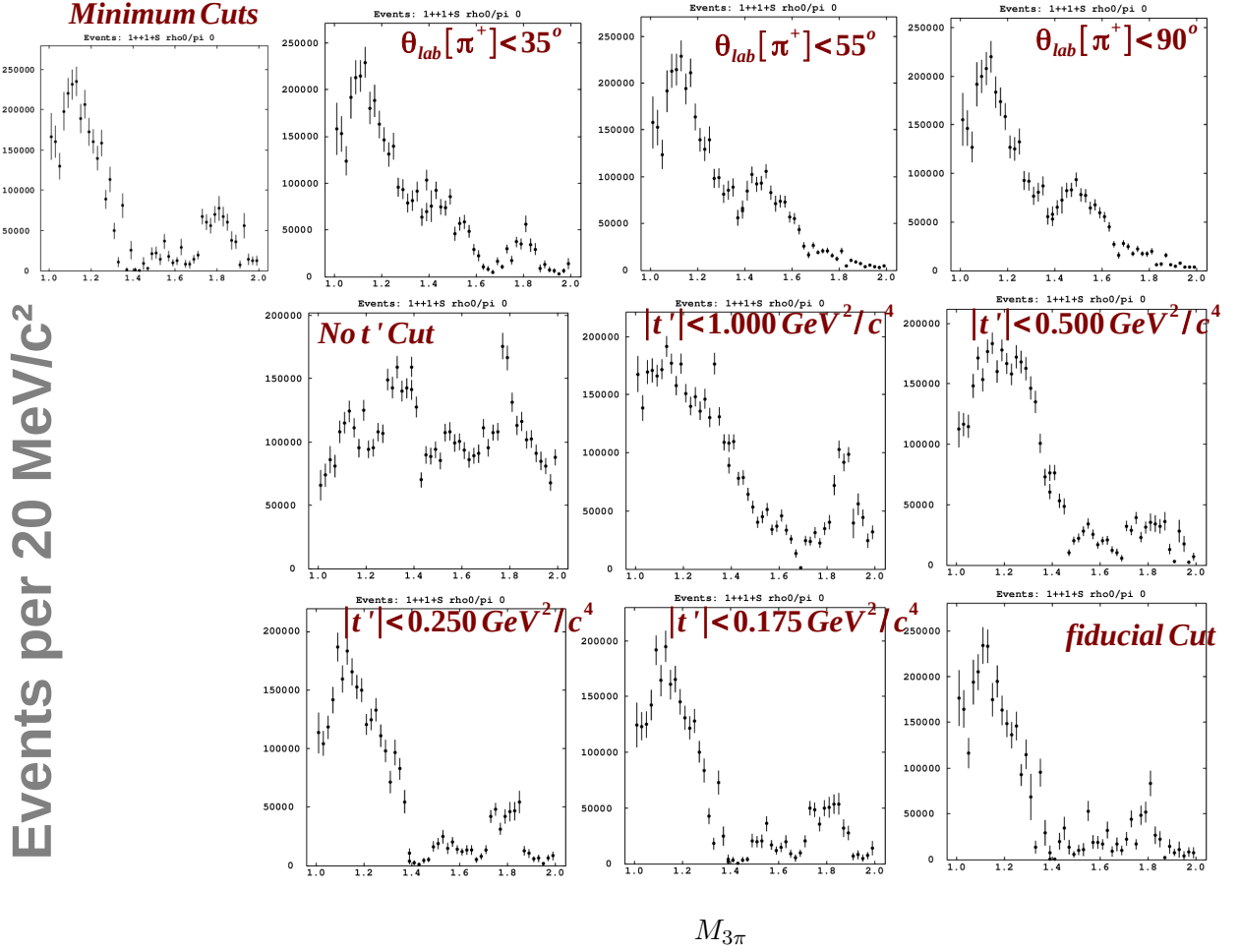
Figure D.8: \gamma p \rightarrow n \pi^+ \pi^+ \pi^- : 1^{++}1^+S intensities for various selection criteria. The specific selection that is applied is labeled in each plot separately. The minimum represents the cuts that are in the PWA results Chapter.
