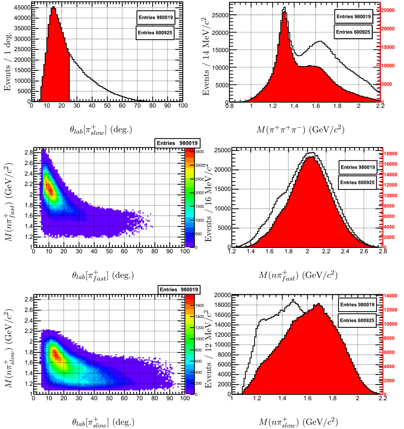
Figure 5.2: \gamma p \rightarrow n \pi^+ \pi^+ \pi^- : The first column shows the \theta_{lab}(\pi_{slow}^+) distribution and its correlation with the n \pi^+ invariant mass. The second column is the 3\pi and n \pi^+ invariant mass distributions. The red histograms have been plotted for events with \theta_{lab}(\pi_{slow}^+) < 25^\circ .
