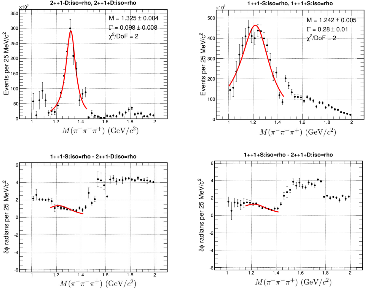
Figure 8.6: For the \gamma p \rightarrow \Delta^{++} \pi^+ \pi^- \pi^- reaction, the top row shows the intensity, combined over two reflectivities M^\epsilon = 1^\pm , for the 2^{++}1^\pm[\rho(770)\pi]_D and the 1^{++}1^\pm[\rho(770)\pi]_S partial waves. The two intensities have been fitted with a mass dependent BW function which is plotted with a red curve along with the obtained parameters. In the bottom row , the phase difference of the 2^{++}D wave against 1^{++}S wave for the two different reflectivities is shown. The red curve is a plot of BW phase difference with the parameters obtained by fitting the intensities.
