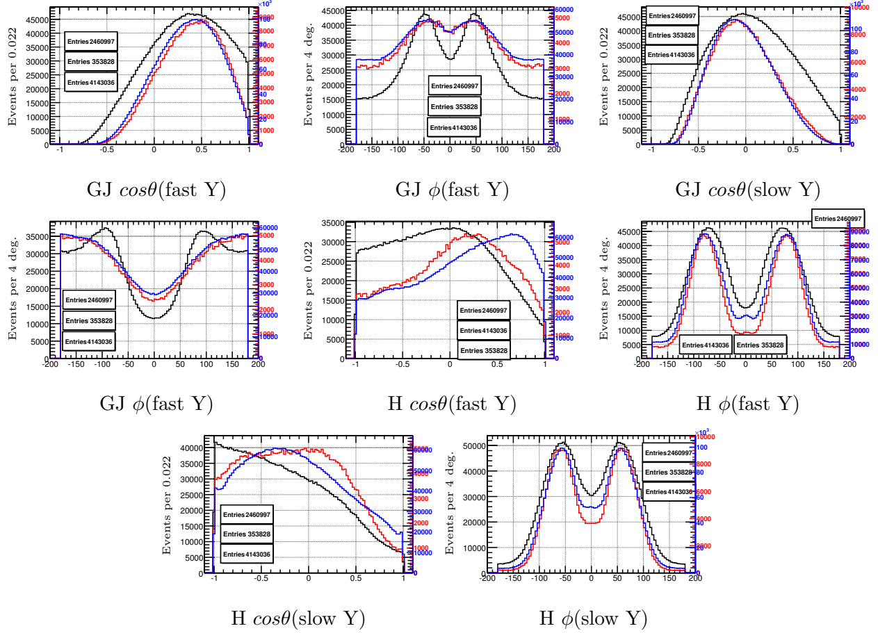
Figure A.3: \gamma p \rightarrow \pi^- \pi^- \pi^+ \Delta^{++} : Rest frame angles. Black line is for data without baryon reduction. Red line is for data with baryon reduction background cuts. Blue line is for Monte-Carlo with baryon reduction background cuts.
