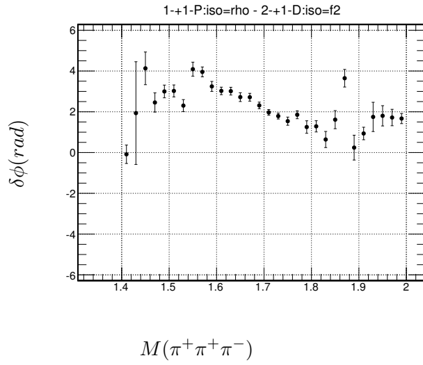
Figure C.9: \gamma p \rightarrow n\pi^+\pi^+\pi^- : Phase difference between the 1^-+1^-P[Y = \rho(770)] wave and the 2^-+1^-D[Y = f_2(1270)] wave for negative ( left ) and positive ( right ) reflectivity.
