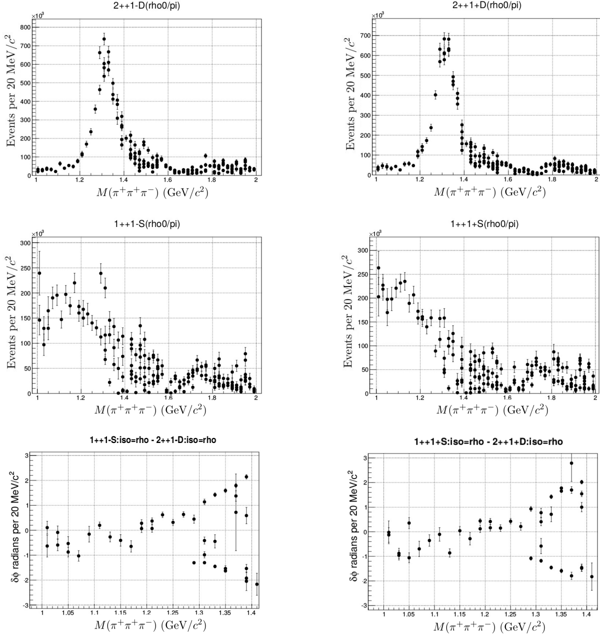
Figure 9.6: \gamma p \rightarrow n \pi^+ \pi^+ \pi^- : Results of multiple random fits after selection of only fits with final likelihood within 60 counts from the minimum value found. The top and middle plots show the intensities for the 1^{++}1^\pm[\rho(770)\pi]_S and 2^{++}1^\pm[\rho(770)\pi]_D waves. The bottom left plot shows the phase difference between the 1^{++}1^-[\rho(770)\pi]_S and 2^{++}1^-[\rho(770)\pi]_D wave. The bottom right plot shows the phase difference between the 1^{++}1^+[\rho(770)\pi]_S and 2^{++}1^+[\rho(770)\pi]_D wave.
