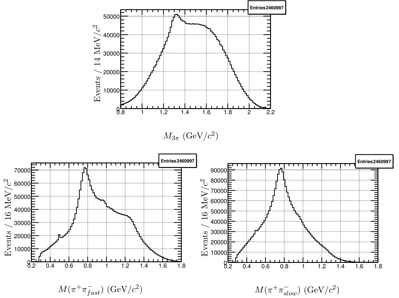
Figure 4.3: Plots of interest for the \gamma p \rightarrow \pi^- \pi^- \pi^+ \Delta^{++} reaction. Difference in momentum cut has been applied here. Top: invariant mass of the 3\pi system. Bottom Left: invariant mass of \pi^+ \pi_{fast}^- . Bottom Right: invariant mass of \pi^+ \pi_{slow}^- .
