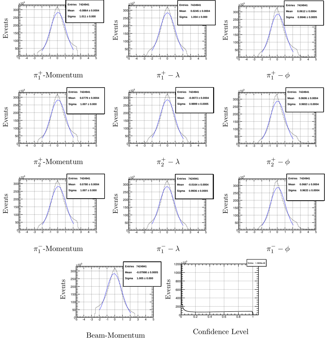
Figure 3.12: Kinematic fit results for high energy photons for the \gamma p \rightarrow \pi^+ \pi^- \pi^+[n] reaction. The events in the pull distributions are greater than 1% confidence level and they have been fitted with a Gaussian function. The bottom right plot is the confidence level distribution for a missing neutron hypothesis.
