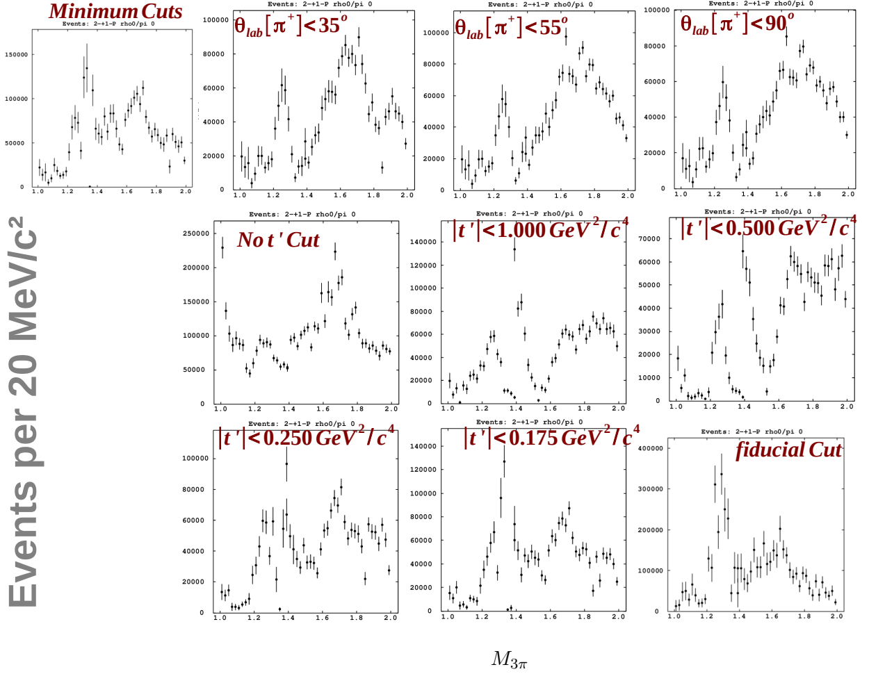
Figure D.11: \gamma p \rightarrow n \pi^+ \pi^+ \pi^- : 2^{-+}1^{-}P intensities for various selection criteria. The specific selection that is applied is labeled in each plot separately. The minimum represents the cuts that are in the PWA results Chapter.
