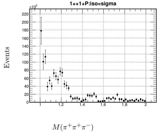
Figure C.4: \gamma p \rightarrow n\pi^+\pi^+\pi^- : The intensity spectrum of the 1^{++}1^{-}P[Y = \sigma] ( left ) and 1^{++}1^{+}P[Y = \sigma] ( right ) partial waves.
