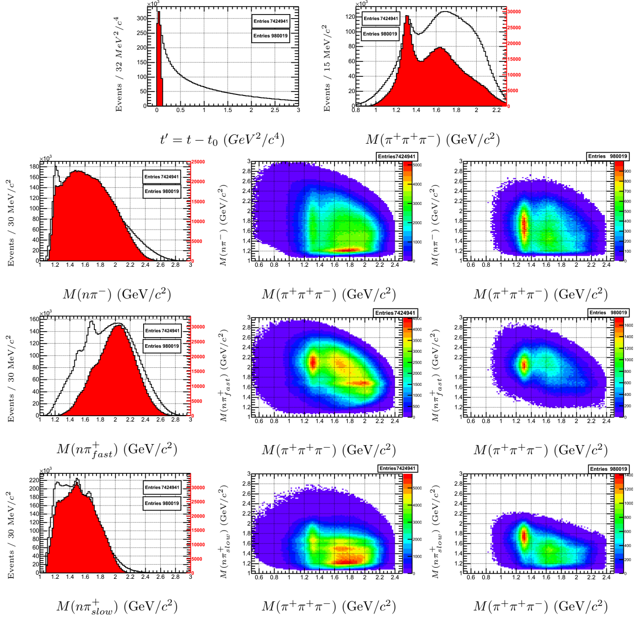
Figure 5.1: \gamma p \rightarrow n \pi^+ \pi^+ \pi^- : The top two plots show the t' and the 3\pi invariant mass distributions. The first column shows the n\pi invariant mass distributions. The second column shows the correlations between the n\pi and 3\pi invariant mass plots and the third column shows those correlations for events with t' < 0.1 \text{ GeV}^2/c^4 .
