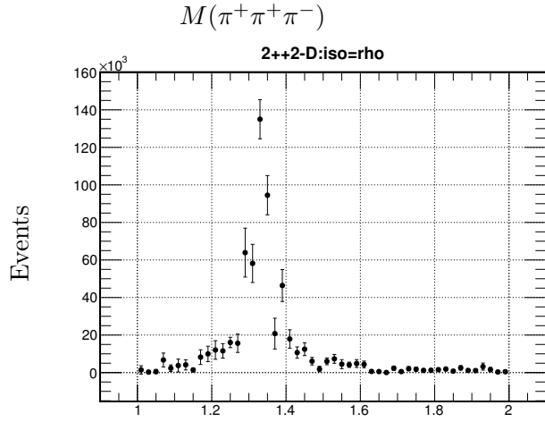
Figure C.1: \gamma p \rightarrow n\pi^+\pi^+\pi^- : The intensity spectrum of the 2^{++}1^-D[Y = \rho(770)] (top left), 2^{++}1^+D[Y = \rho(770)] (top right), 2^{++}2^-D[Y = \rho(770)] (bottom left) and 2^{++}2^+D[Y = \rho(770)] (bottom right) partial waves.
