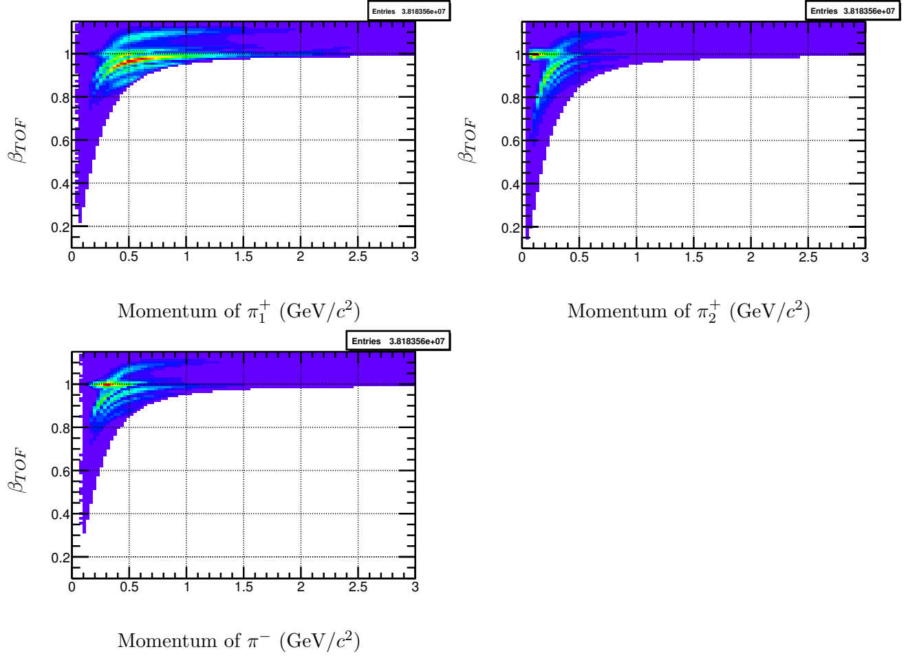
Figure 3.10: \gamma p \rightarrow n\pi^+\pi^+\pi^- : The Figure shows for each pion the \beta as measured from the Time of Flight detector against the momentum of the particle. The events showed have at least two charged tracks with \delta\beta > 0.03 .
