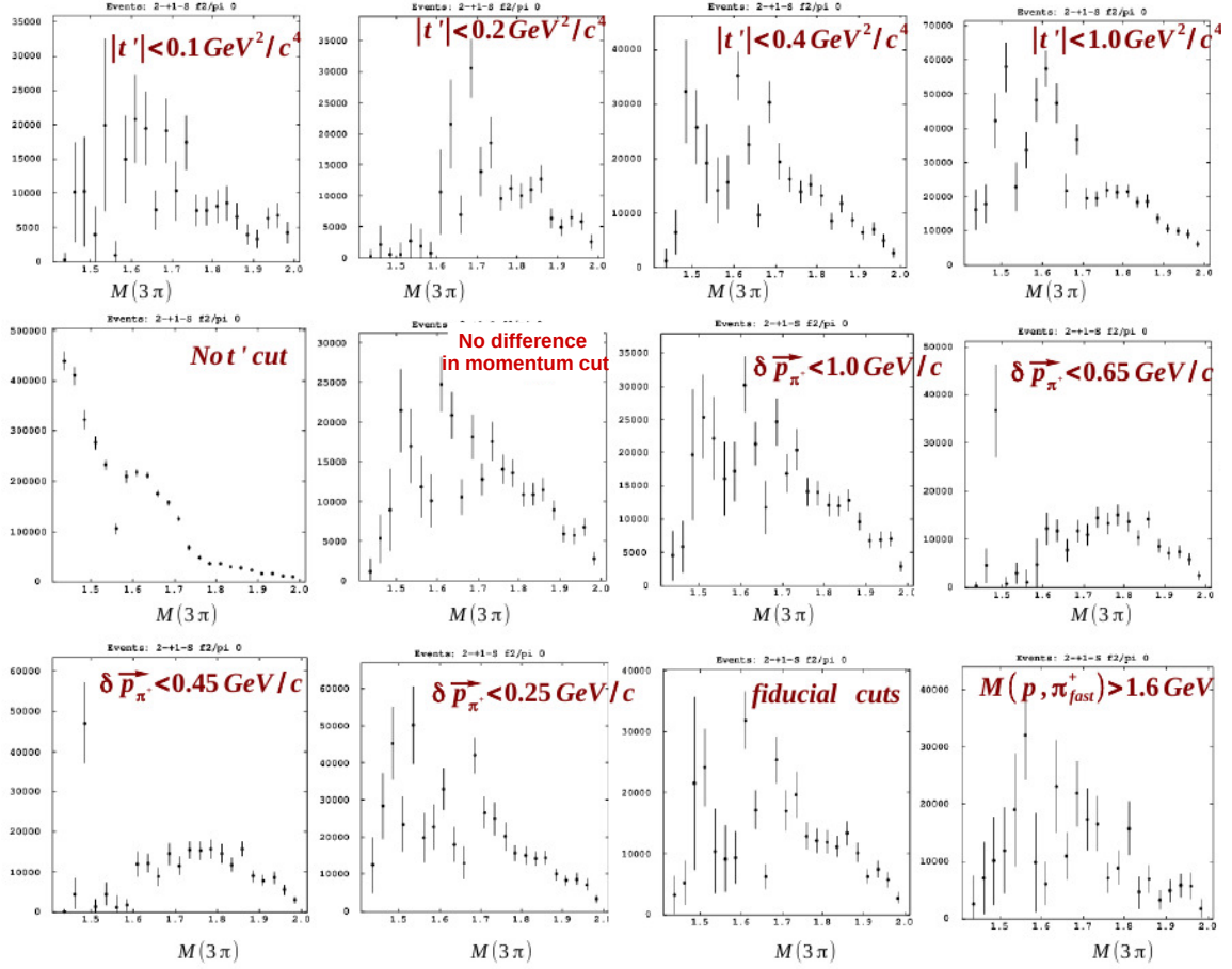
Figure F.2: \gamma p \rightarrow \pi^- \pi^- \pi^+ \Delta^{++} : 2^{-+}1^+S intensities for various selection criteria. The specific selection that is applied is labeled in each plot separately. The fit-results with |t'| < 0.4 \text{ GeV}^2/c^4 represents the cuts that were used in the PWA results Chapter
