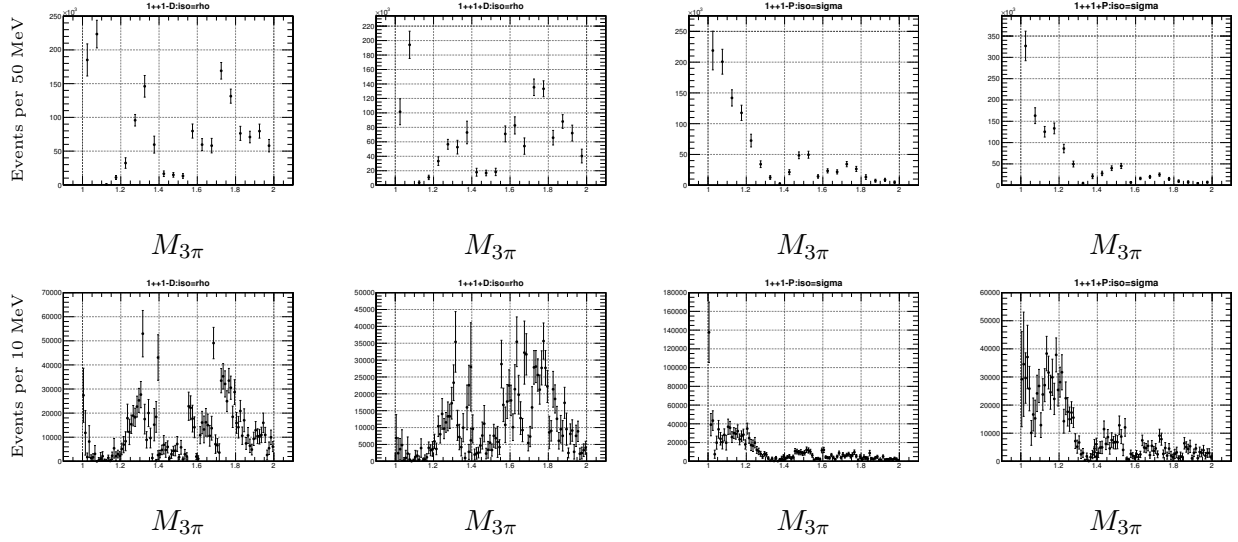
Figure B.2: \gamma p \rightarrow n\pi^+\pi^+\pi^- : 50 MeV mass bin size was used for the top plots and 10 MeV mass bin size for the bottom plots. The first two plots show the intensity of the 1^{++}D waves and the last two plots show the intensity of the 1^{++}P waves.
