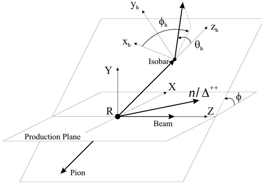
Figure G.2: The Gottfried-Jackson and helicity frames used to describe the sequential decay of the 3\pi meson resonance. The recoil particle lies in the XZ of the production plane and it is a neutron for the \gamma p \rightarrow n\pi^+\pi^+\pi^- reaction and a \Delta^{++} for the \gamma p \rightarrow \pi^-\pi^-\pi^+\Delta^{++} reaction.
