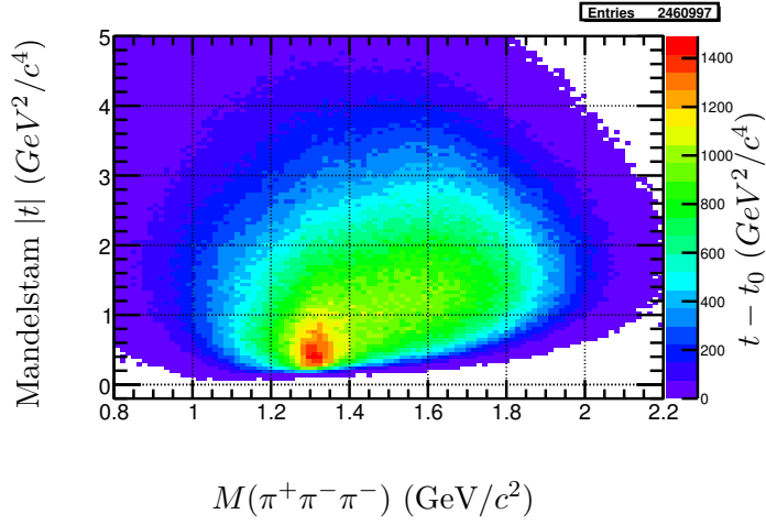
Figure 4.4: \gamma p \rightarrow \pi^-\pi^-\pi^+\Delta^{++} : The top plot shows an exponential fit of the Mandelstam t distribution. The bottom left plot shows the t against the 3\pi invariant mass and the bottom right plot shows the normalized t , t' , against the 3\pi invariant mass.
