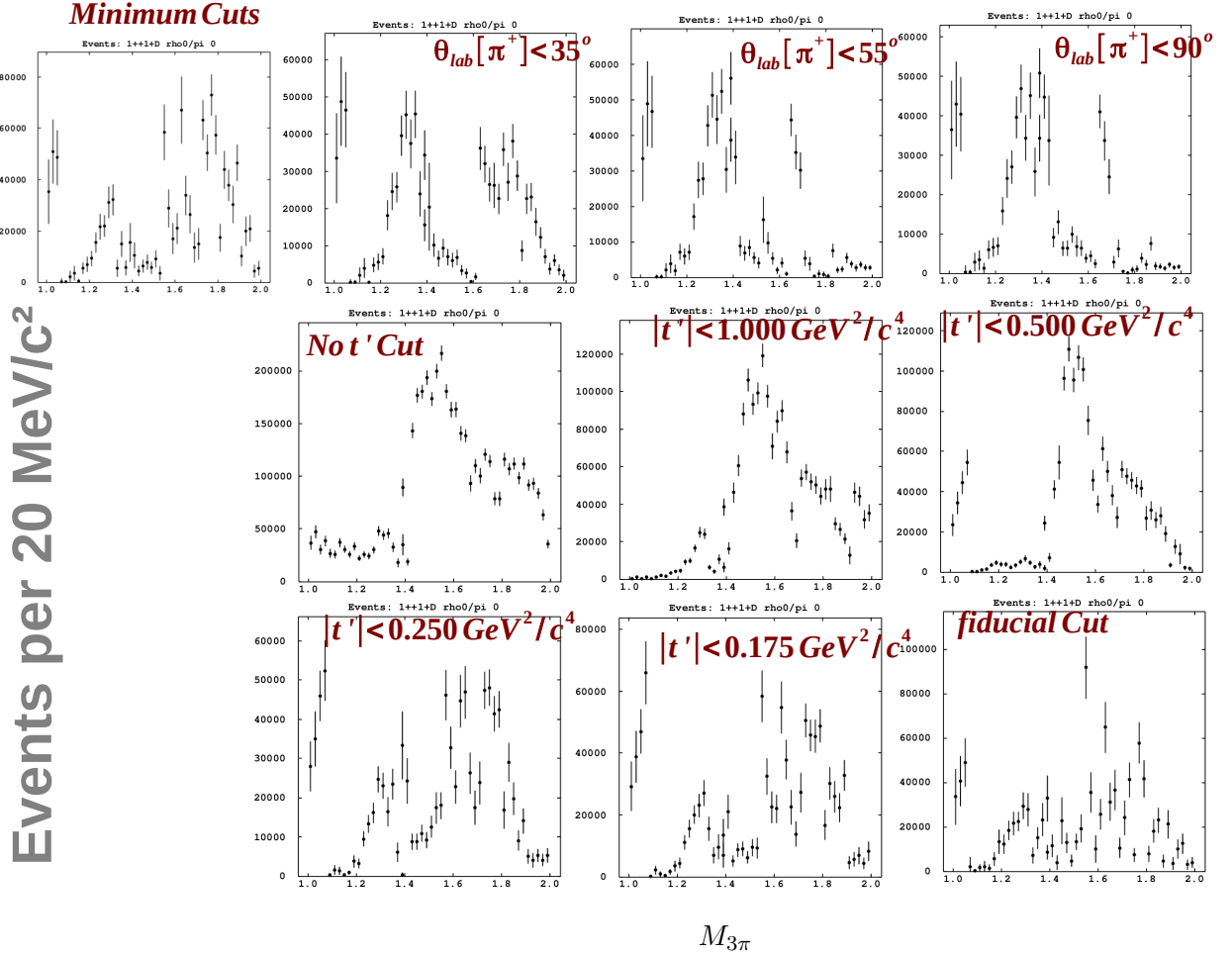
Figure D.4: \gamma p \rightarrow n \pi^+ \pi^+ \pi^- : 1^{++}1^+D intensities for various selection criteria. The specific selection that is applied is labeled in each plot separately. The minimum represents the cuts that are in the PWA results Chapter.
