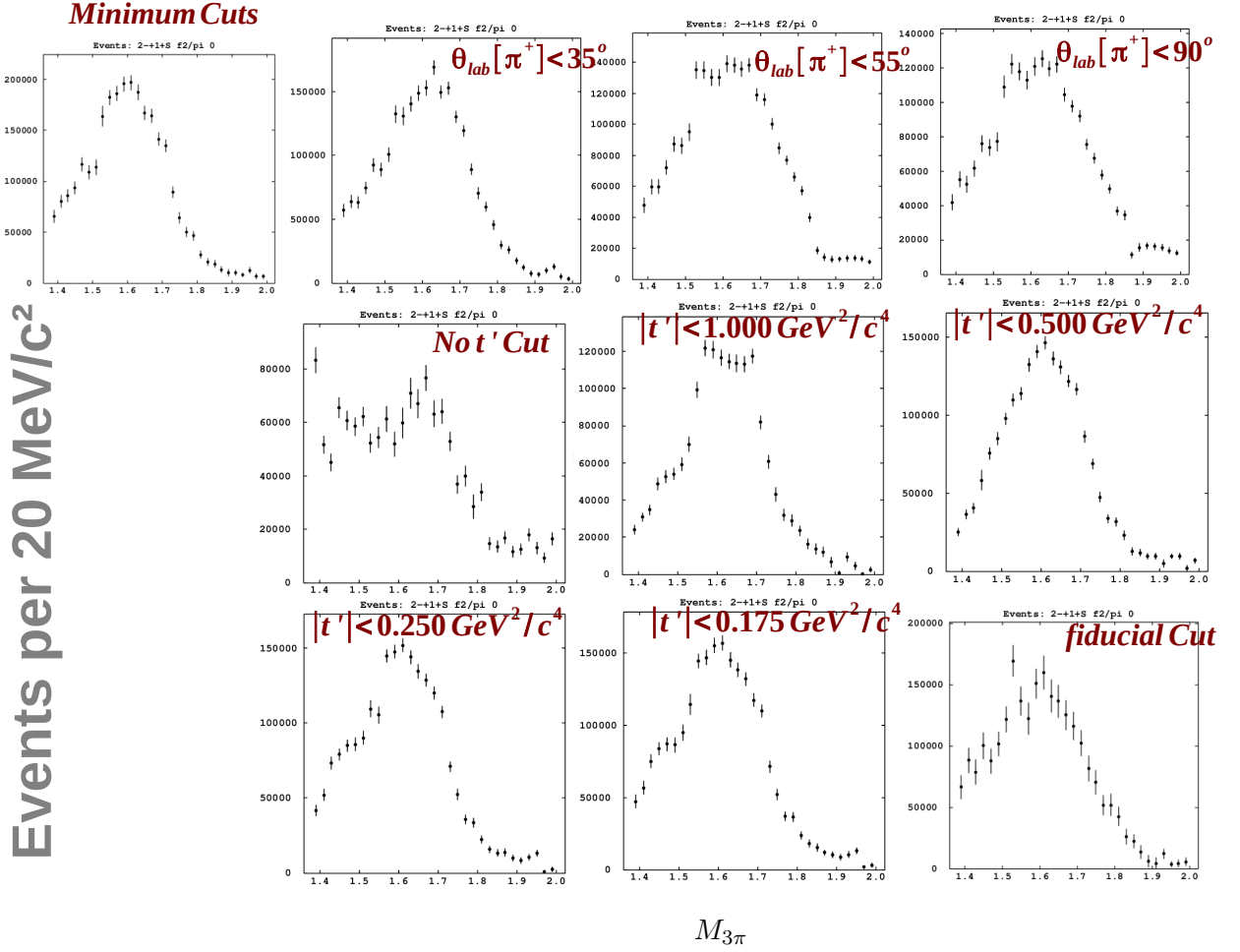
Figure D.14: \gamma p \rightarrow n \pi^+ \pi^+ \pi^- : 2^- 1^+ S intensities for various selection criteria. The specific selection that is applied is labeled in each plot separately. The minimum represents the cuts that are in the PWA results Chapter.
