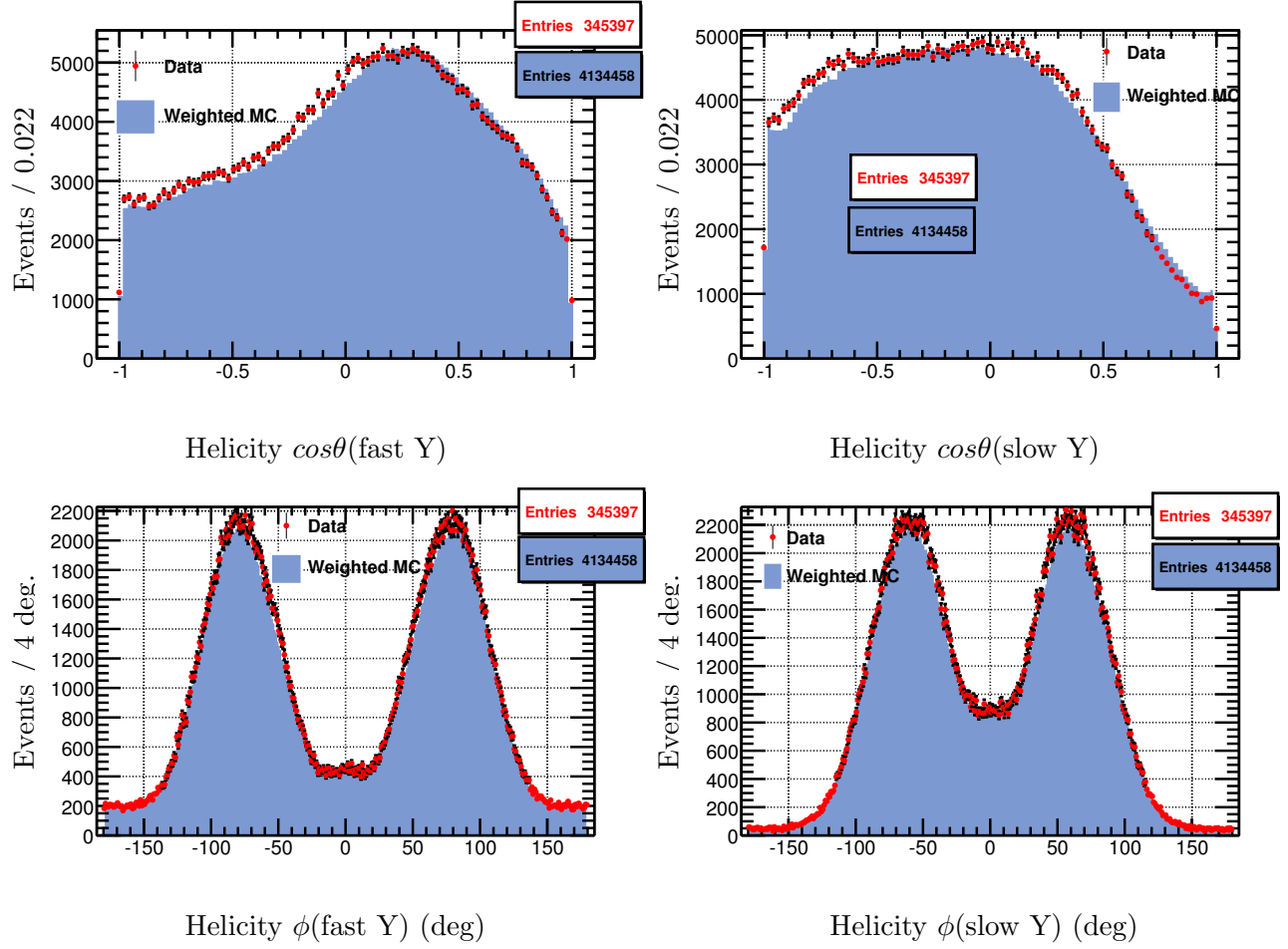
Figure 8.11: \gamma p \rightarrow \pi^- \pi^- \pi^+ \Delta^{++} : Angular distributions in the Helicity rest frame for data (points) and predicted (blue histograms) four-vectors.
