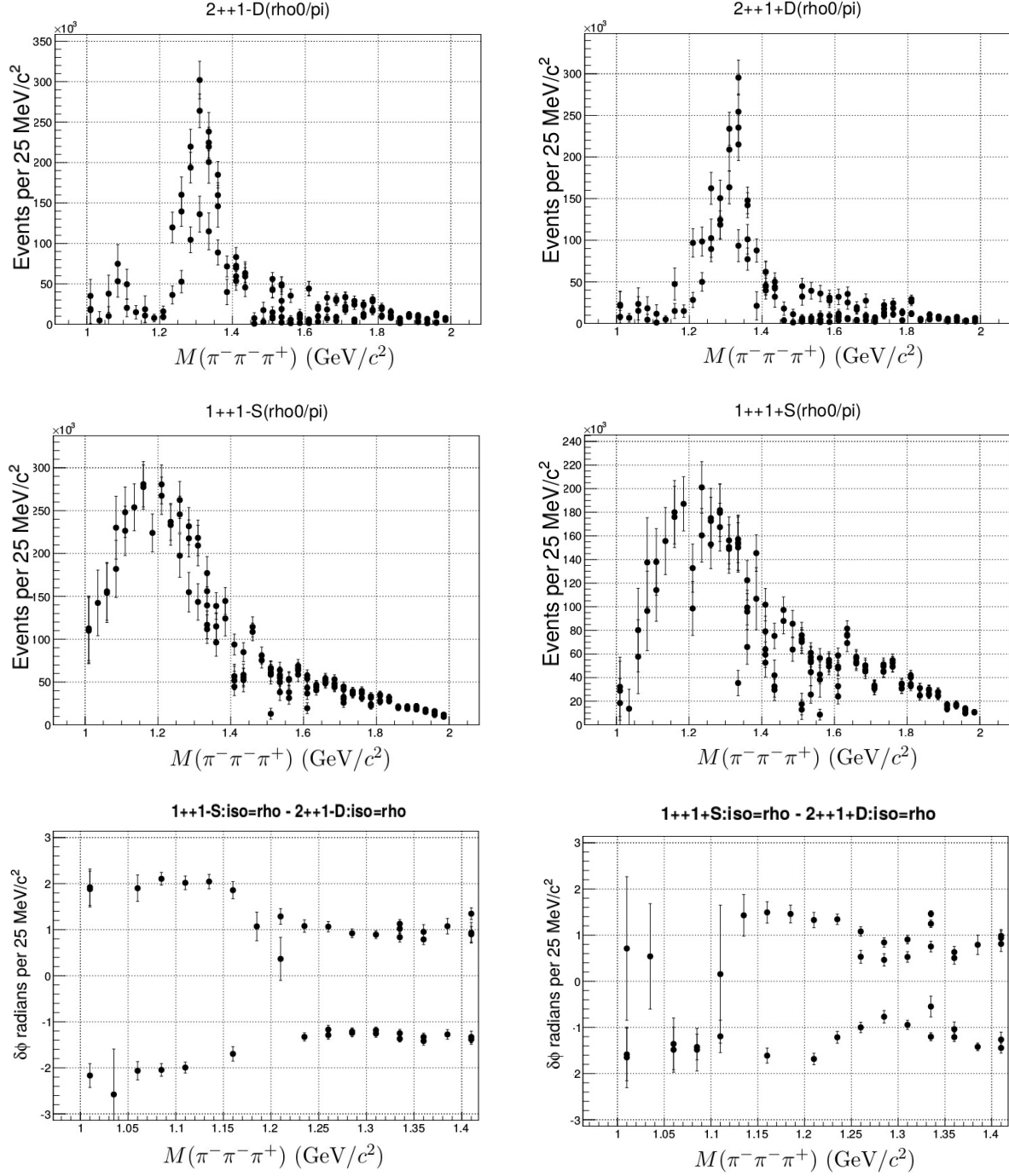
Figure 8.5: \gamma p \rightarrow \pi^- \pi^- \pi^+ \Delta^{++} : Results of multiple random fits after selection of only fits with final likelihood within 60 counts from the minimum value found. The top and middle plots show the intensities for the 1^{++}1^{\pm}[\rho(770)\pi]_S and 2^{++}1^{\pm}[\rho(770)\pi]_D waves. The bottom left plot shows the phase difference between the 1^{++}1^{-}[\rho(770)\pi]_S and 2^{++}1^{-}[\rho(770)\pi]_D wave. The bottom right plot shows the phase difference between the 1^{++}1^{+}[\rho(770)\pi]_S and 2^{++}1^{+}[\rho(770)\pi]_D wave.
