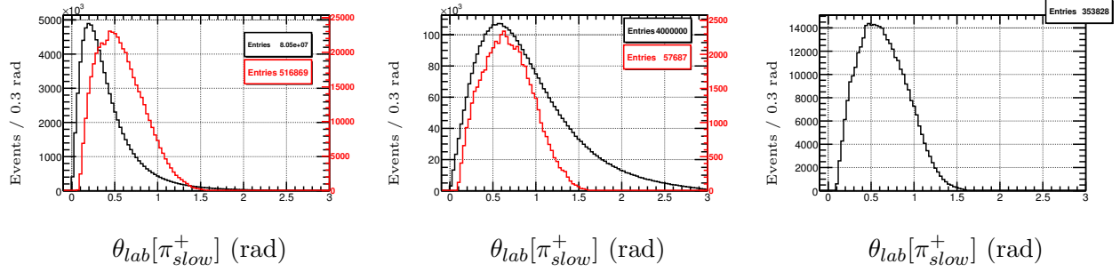
Figure 8.15: Left: \theta_{lab}[\pi_{slow}^+] for generated (black line) and accepted (red line) \gamma p \rightarrow p 4\pi events. Middle: \theta_{lab}[\pi_{slow}^+] for generated (black line) and accepted (red line) \gamma p \rightarrow \pi^- \pi^- \pi^+ \Delta^{++} events. Right: \theta_{lab}[\pi_{slow}^+] for \gamma p \rightarrow \pi^- \pi^- \pi^+ \Delta^{++} data events.
