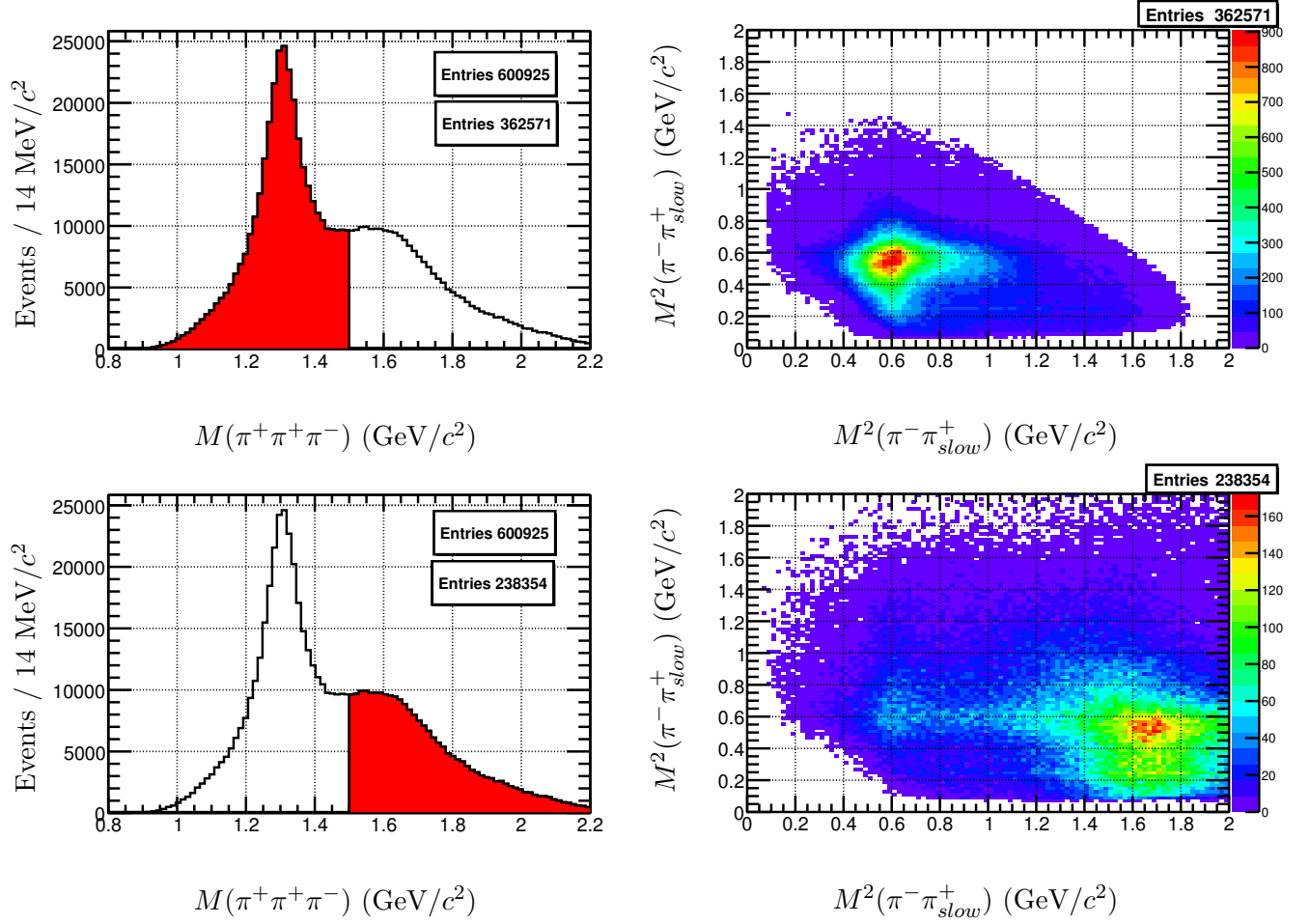
Figure 5.4: \gamma p \rightarrow n \pi^+ \pi^+ \pi^- : The top right plot shows the Dalitz plot for M_{3\pi} < 1.5 \text{ GeV}/c (low mass region). The bottom right plot shows the Dalitz plot for M_{3\pi} > 1.5 \text{ GeV}/c (high mass region).
