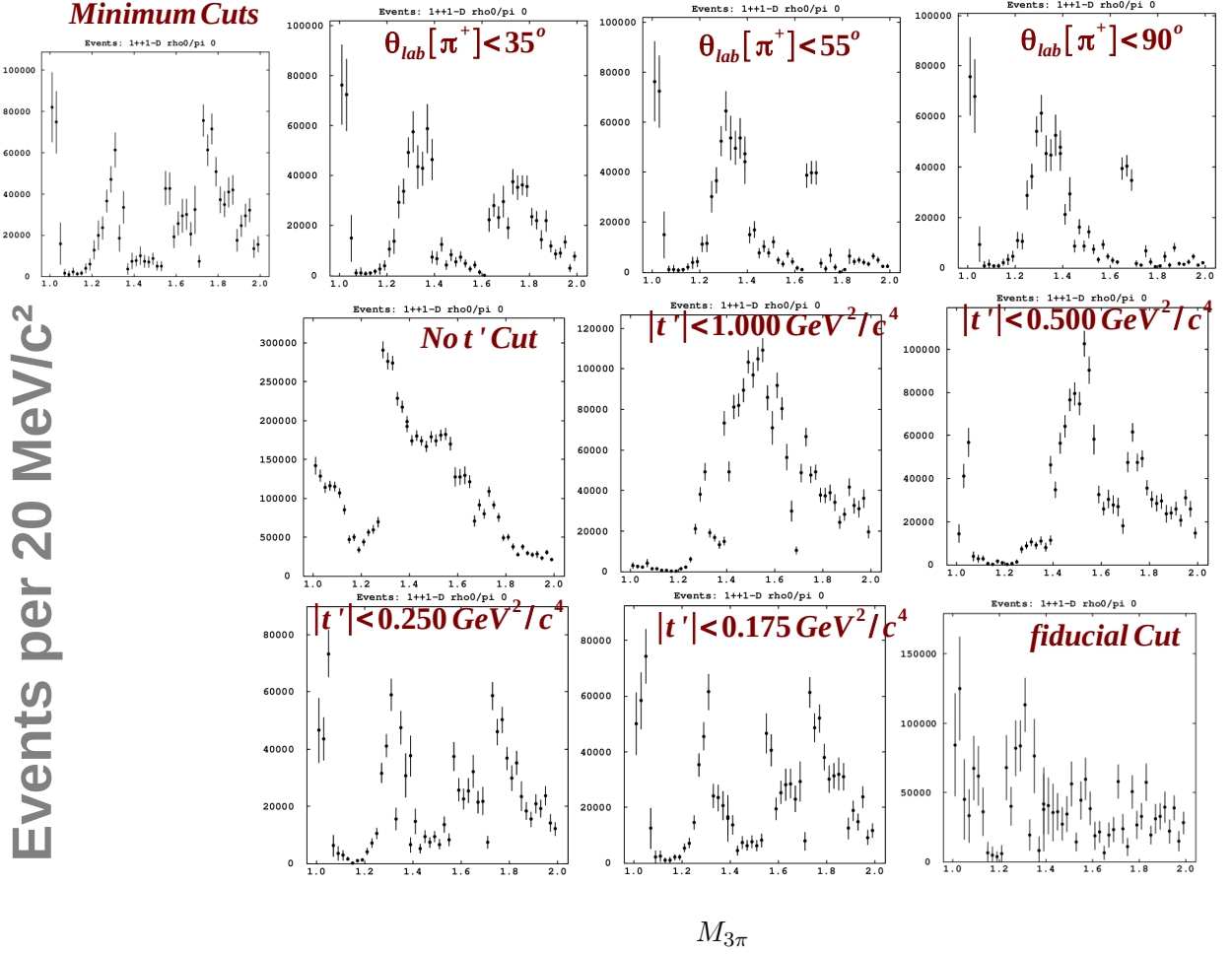
Figure D.3: \gamma p \rightarrow n \pi^+ \pi^+ \pi^- : 1^{++}1^-D intensities for various selection criteria. The specific selection that is applied is labeled in each plot separately. The minimum represents the cuts that are in the PWA results Chapter.
