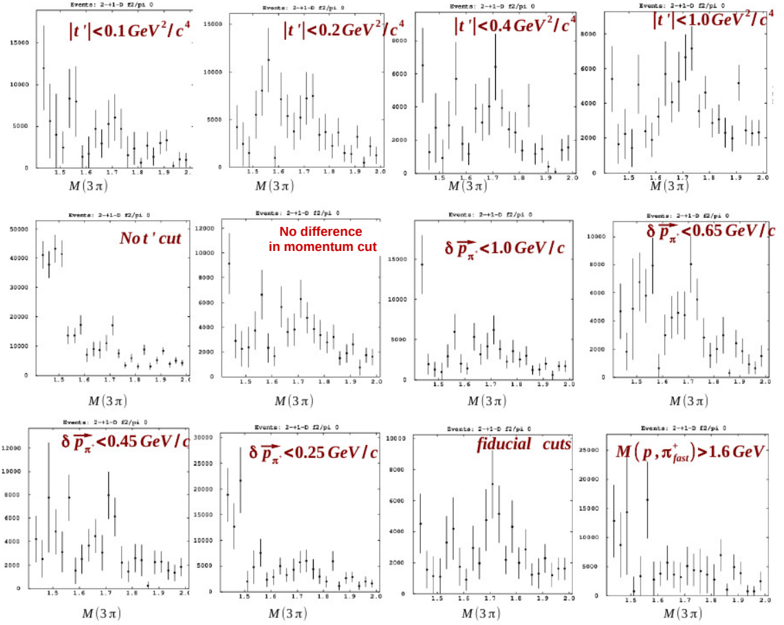
Figure F.6: \gamma p \rightarrow \pi^- \pi^- \pi^+ \Delta^{++} : 2^{-+}1^+D intensities for various selection criteria. The specific selection that is applied is labeled in each plot separately. The fit-results with |t'| < 0.4 \text{ GeV}^2/c^4 represents the cuts that were used in the PWA results Chapter
