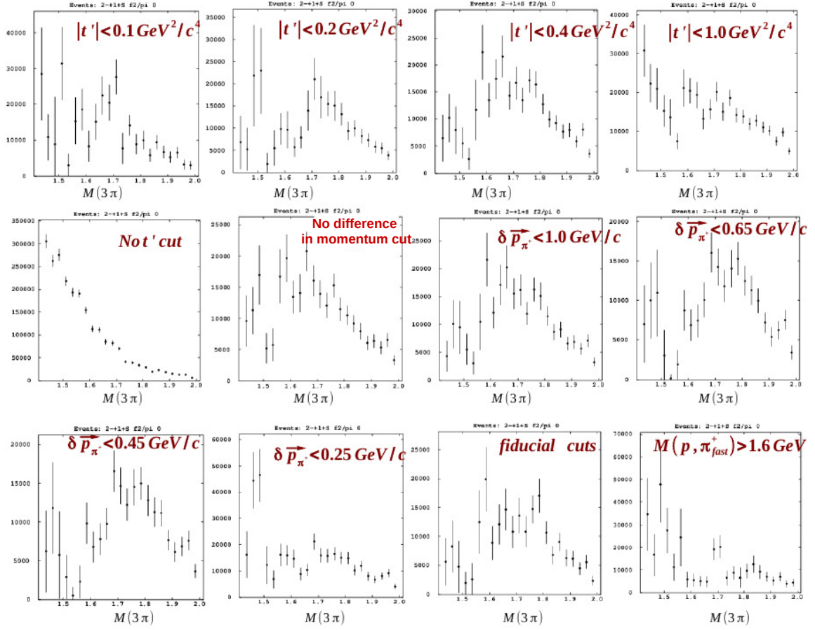
Figure F.1: \gamma p \rightarrow \pi^- \pi^- \pi^+ \Delta^{++} : 2^{-+}1^{-}S intensities for various selection criteria. The specific selection that is applied is labeled in each plot separately. The fit-results with |t'| < 0.4 \text{ GeV}^2/c^4 represents the cuts that were used in the PWA results Chapter
