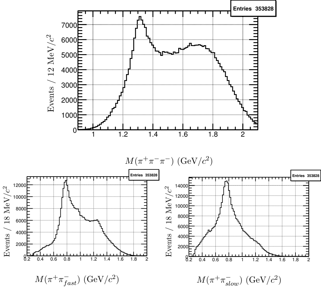
Figure 4.14: \gamma p \rightarrow \pi^-\pi^-\pi^+\Delta^{++} : The top plot shows the invariant 3\pi mass distribution for the final number of events that were used in the PWA. The bottom plots are the \pi\pi invariant mass distributions.
