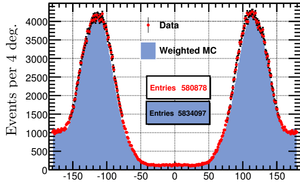
Helicity \phi (fast Y) (deg)
