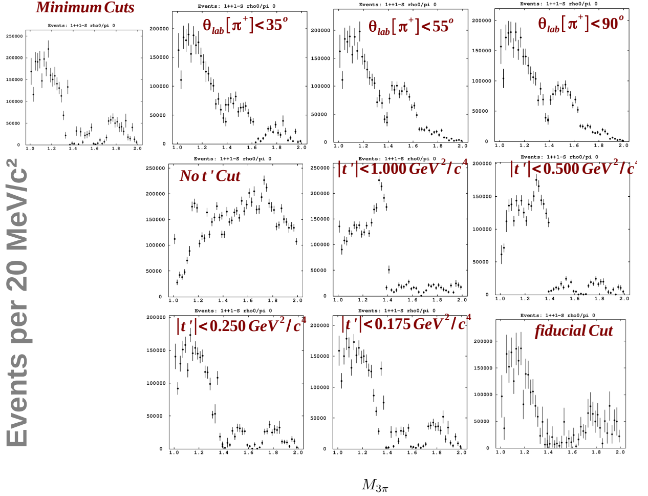
Figure D.7: \gamma p \rightarrow n \pi^+ \pi^+ \pi^- : 1^{++}1^{-}S intensities for various selection criteria. The specific selection that is applied is labeled in each plot separately. The minimum represents the cuts that are in the PWA results Chapter.
