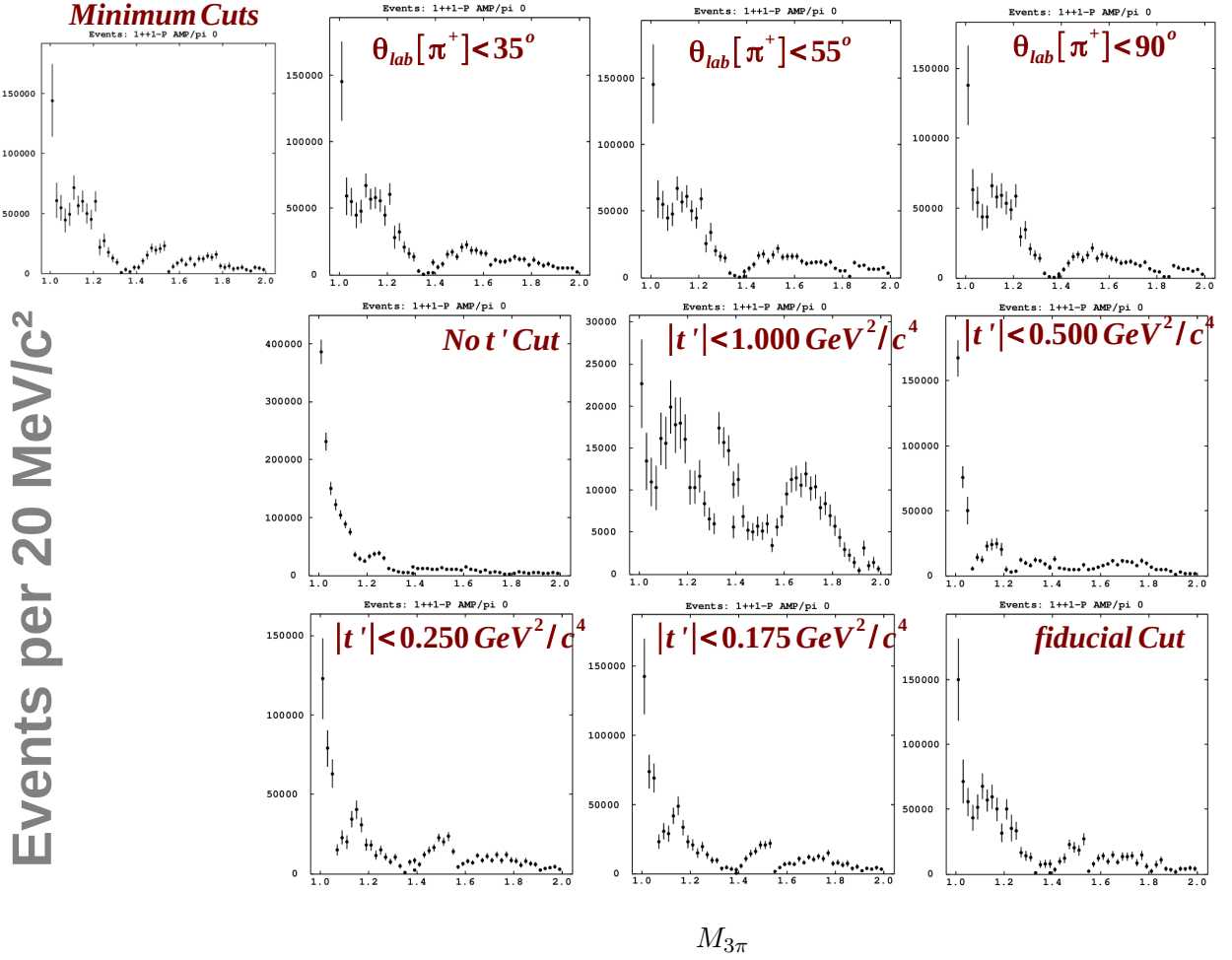
Figure D.5: \gamma p \rightarrow n\pi^+\pi^+\pi^- : 1^{++}1^-P intensities for various selection criteria. The specific selection that is applied is labeled in each plot separately. The minimum represents the cuts that are in the PWA results Chapter.
