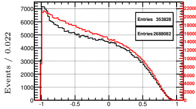
\cos\theta in the \Delta^{++} rest frame for data and summing the helicities for M=1/2
