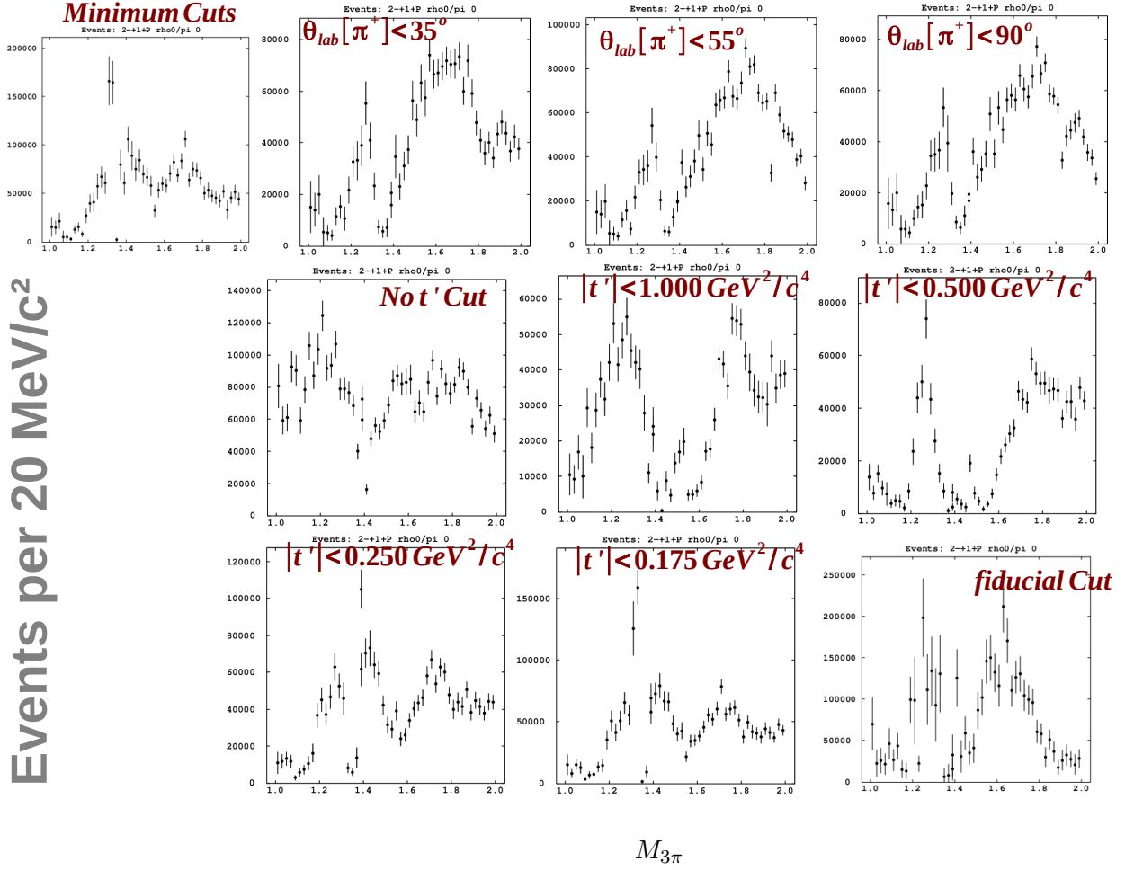
Figure D.12: \gamma p \rightarrow n\pi^+\pi^+\pi^- : 2^-1^+P intensities for various selection criteria. The specific selection that is applied is labeled in each plot separately. The minimum represents the cuts that are in the PWA results Chapter.
