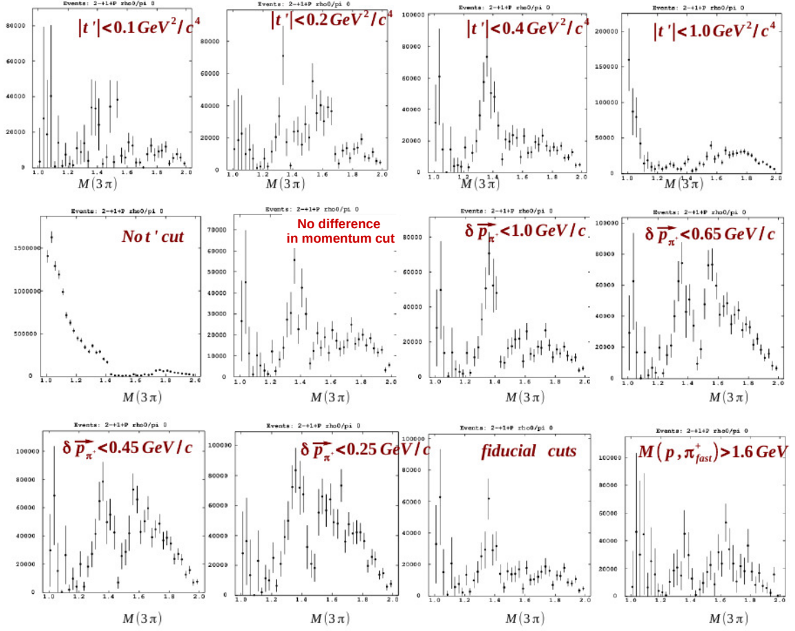
Figure F.3: \gamma p \rightarrow \pi^- \pi^- \pi^+ \Delta^{++} : 2^{+}1^{-}P intensities for various selection criteria. The specific selection that is applied is labeled in each plot separately. The fit-results with |t'| < 0.4 \text{ GeV}^2/c^4 represents the cuts that were used in the PWA results Chapter
