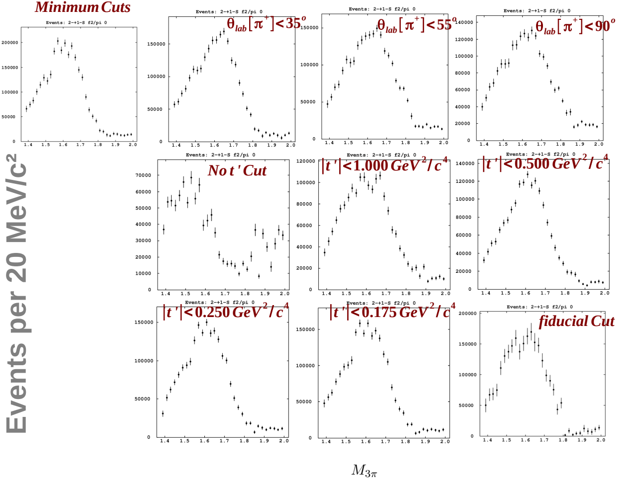
Figure D.13: \gamma p \rightarrow n\pi^+\pi^+\pi^- : 2^{-+}1^{-}S intensities for various selection criteria. The specific selection that is applied is labeled in each plot separately. The minimum represents the cuts that are in the PWA results Chapter.
