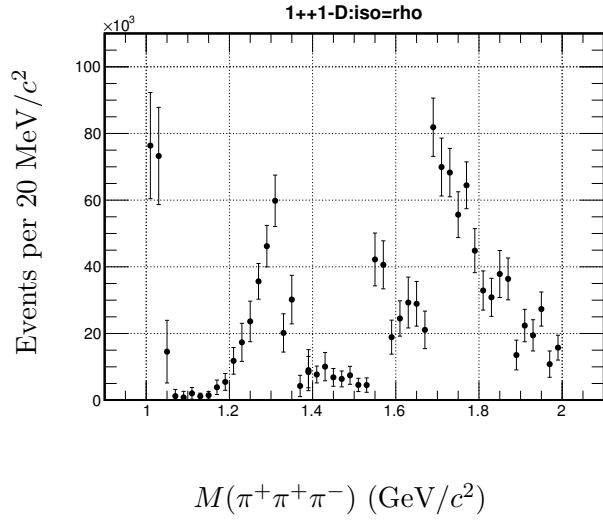
Figure 9.2: \gamma p \rightarrow n\pi^+\pi^+\pi^- : The partial wave intensity spectra of the 1^{++}1^{-}[\rho(770)\pi]_S ( top left ), 1^{++}1^{+}[\rho(770)\pi]_S ( top right ), 1^{++}1^{-}[\rho(770)\pi]_D ( bottom left ) and 1^{++}1^{+}[\rho(770)\pi]_D ( bottom right ) partial waves.
