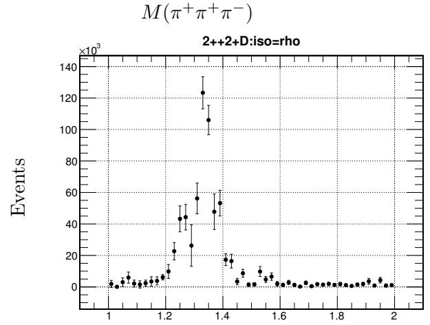
Figure C.1: \gamma p \rightarrow n\pi^+\pi^+\pi^- : The intensity spectrum of the 2^{++}1^-D[Y = \rho(770)] (top left), 2^{++}1^+D[Y = \rho(770)] (top right), 2^{++}2^-D[Y = \rho(770)] (bottom left) and 2^{++}2^+D[Y = \rho(770)] (bottom right) partial waves.
