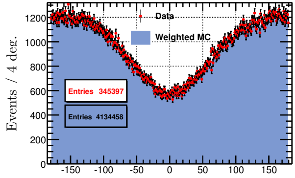
GJ \phi(\text{slow Y}) (deg)
