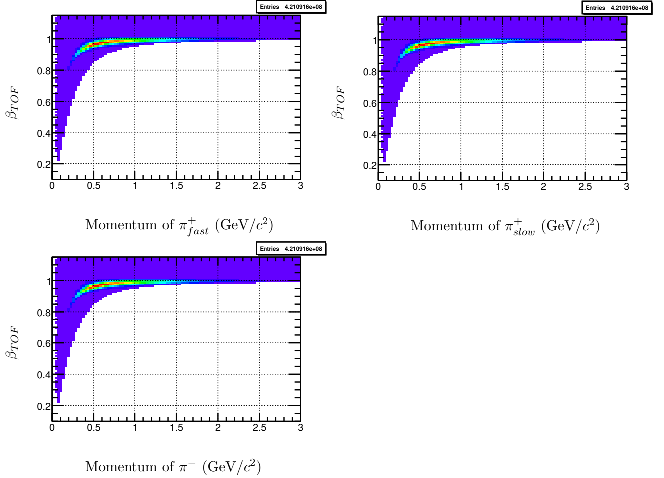
Figure 3.9: \gamma p \rightarrow n\pi^+\pi^+\pi^- : The Figure shows for each pion the \beta as measured from the Time of Flight detector against the momentum of the particle. The events showed have at least two charged tracks with \delta\beta < 0.03 .
