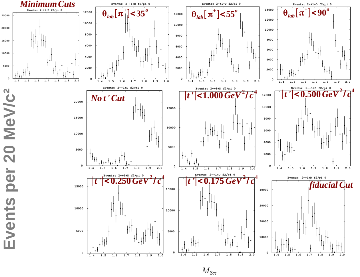
Figure D.10: \gamma p \rightarrow n\pi^+\pi^+\pi^- : 2^-1^+D intensities for various selection criteria. The specific selection that is applied is labeled in each plot separately. The minimum represents the cuts that are in the PWA results Chapter.
