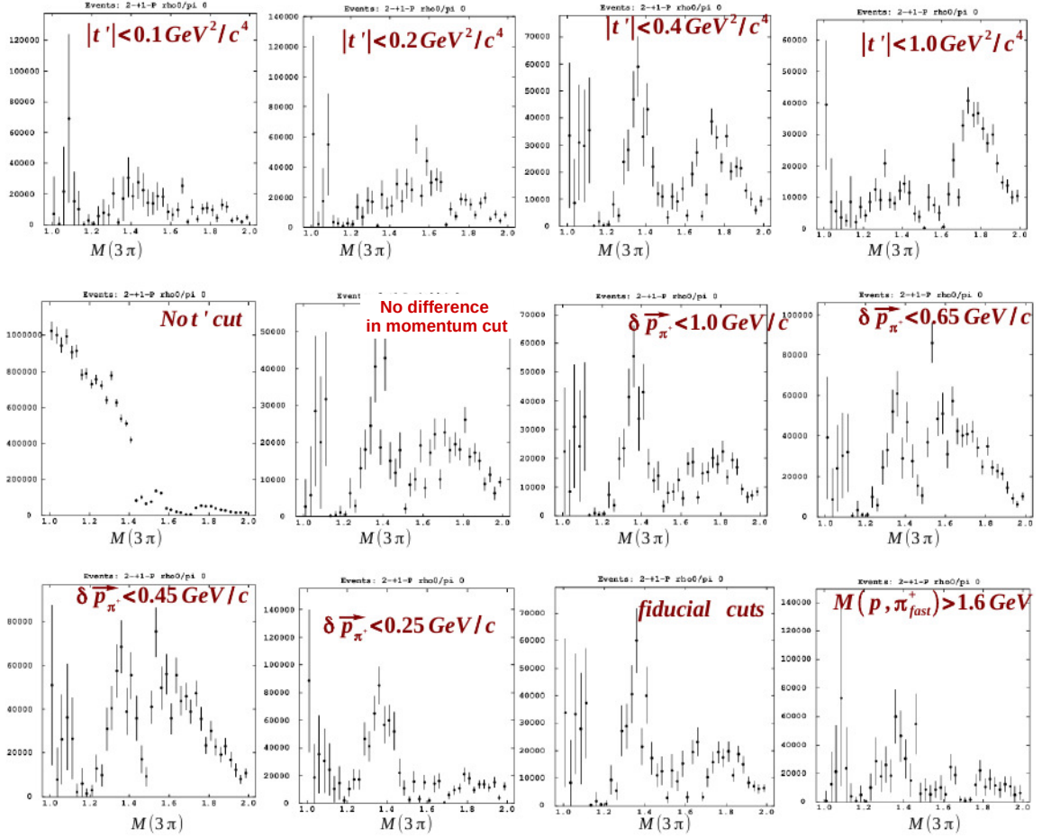
Figure F.4: \gamma p \rightarrow \pi^- \pi^- \pi^+ \Delta^{++} : 2^{-+}1^+P intensities for various selection criteria. The specific selection that is applied is labeled in each plot separately. The fit-results with |t'| < 0.4 \text{ GeV}^2/c^4 represents the cuts that were used in the PWA results Chapter
