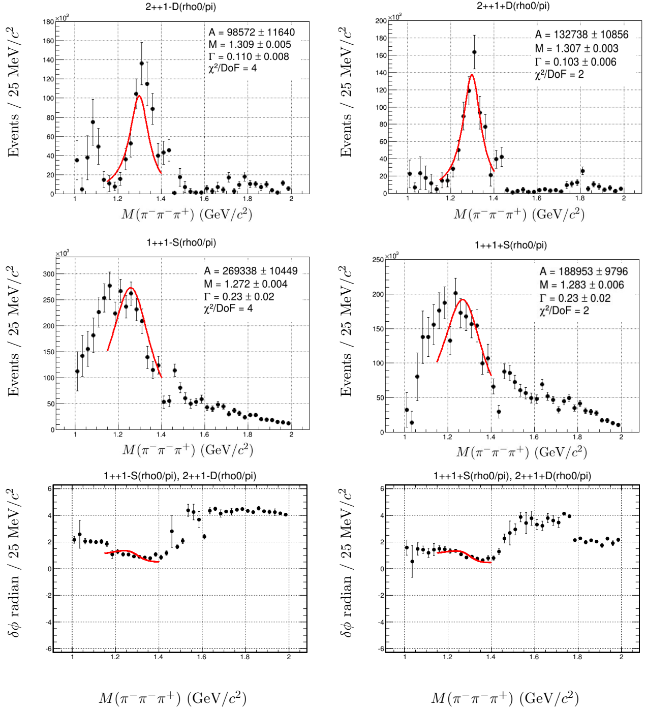
Figure 8.3: \gamma p \rightarrow \pi^- \pi^- \pi^+ \Delta^{++} : A mass dependent fit of the 1^{++}[\rho(770)\pi]_S and 2^{++}[\rho(770)\pi]_D intensity distributions and their phase difference was performed for each reflectivity separately. The first column shows the fit results for M^\epsilon = 1^- and the second column for M^\epsilon = 1^+ .
