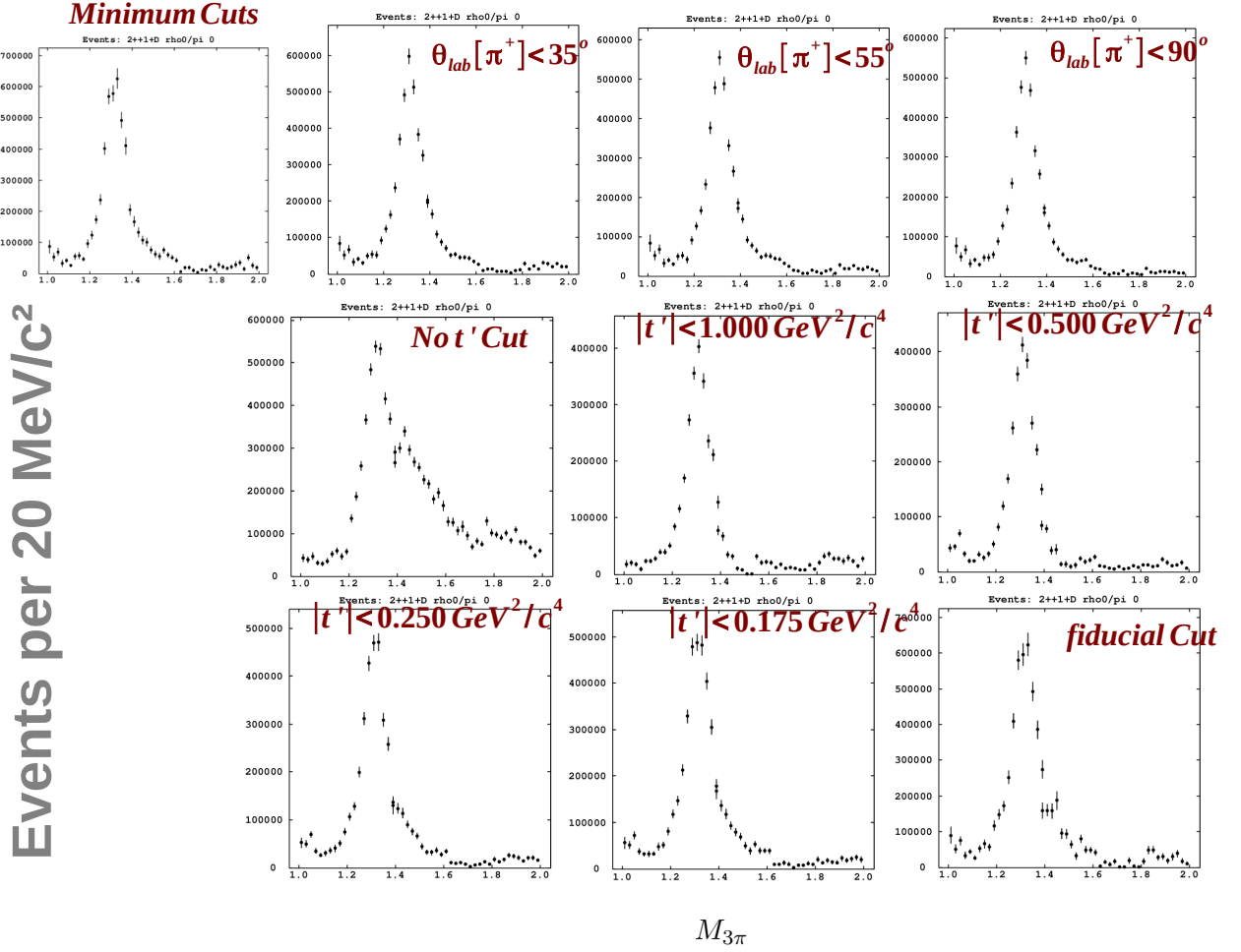
Figure D.16: \gamma p \rightarrow n \pi^+ \pi^+ \pi^- : 2^{++}1^+D intensities for various selection criteria. The specific selection that is applied is labeled in each plot separately. The minimum represents the cuts that are in the PWA results Chapter.
