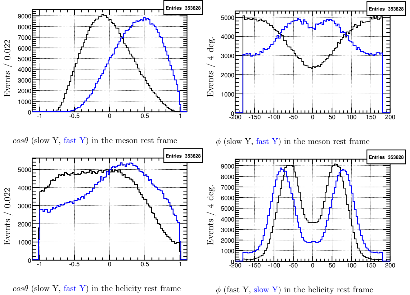
Figure 4.16: \gamma p \rightarrow \pi^- \pi^- \pi^+ \Delta^{++} : \cos\theta and \phi distributions in the meson rest frame ( top ) and in the helicity rest frame ( bottom ) for the final data sample. Top left: for the blue curve the \pi_{fast}^- was used to form the \rho – isobar and for the black curve the \pi_{slow}^- was used to form the \rho – isobar . Top right: \phi distribution for fast and slow isobar. Bottom left: for the blue curve the \pi_{fast}^- was used as the analyzer and for the black curve the \pi_{slow}^- was used as the analyzer. Bottom right: \phi distribution for fast and slow analyzer.
