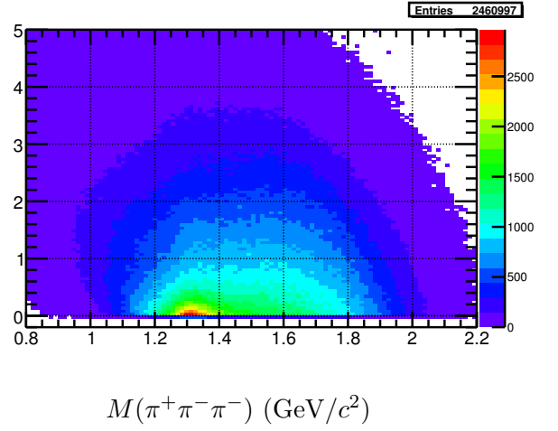
Figure 4.4: \gamma p \rightarrow \pi^-\pi^-\pi^+\Delta^{++} : The top plot shows an exponential fit of the Mandelstam t distribution. The bottom left plot shows the t against the 3\pi invariant mass and the bottom right plot shows the normalized t , t' , against the 3\pi invariant mass.
