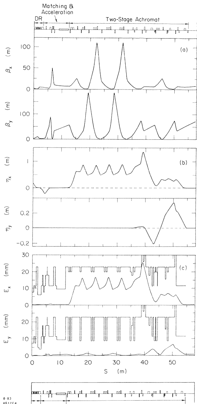
Fig. 4. (a) Beta vs. s (m); (b) Eta vs. s (m); (c) Envelope vs. s (m); where E = \sqrt{\epsilon\beta + (\eta\delta)^2} , for \epsilon_x = \epsilon_y = 0.01 mm-mrad and \delta = 2\% .
