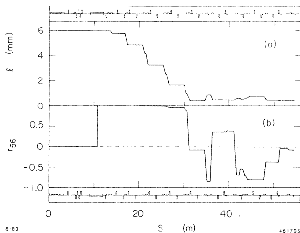
Fig. 5. (a) Bunch length vs. s (m) for \hat{V}_{RF} = 33 MeV; final rms length is 0.5 mm. (b) r_{56}(\ell - \delta correlation) vs. s (m).
