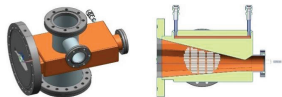
Figure 7: OFHC distributed absorber and cross section.
