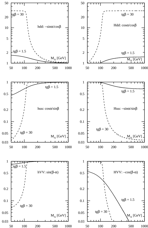
Fig. 10. The coupling parameters of the neutral MSSM Higgs bosons as a function of the pseudoscalar mass M_A for two values of \tan\beta = 1.5, 30 and vanishing mixing. The couplings are defined in Table II.
