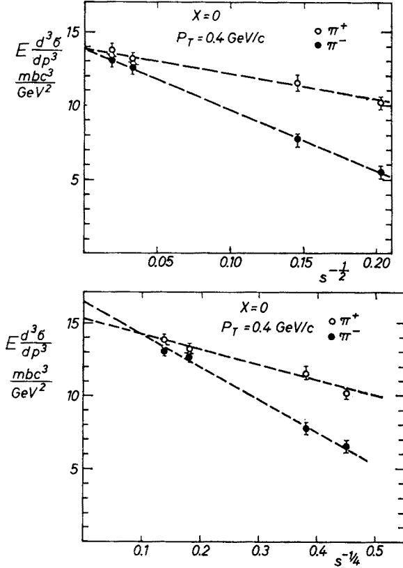
Fig. 11. The cross-sections for pp \rightarrow \pi^\pm X on the s^{-\frac{1}{2}} and s^{-\frac{1}{4}} plots. The two cross-sections should be equal asymptotically, which disfavors the s^{-\frac{1}{2}} behaviour
