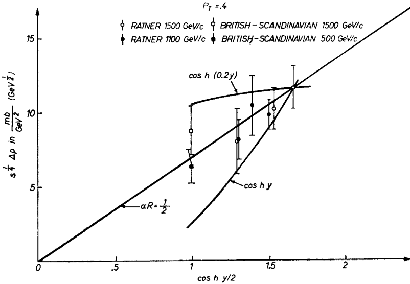
Fig. 9. The quantity s^{-1/4} \Delta_p on a cosh Y/2 plot. The straight line corresponds to Eq. (22). The behaviours cosh (0.2Y) and cosh (Y) , corresponding to \alpha_R(0) = 0.8 and 0 are also shown for comparison
