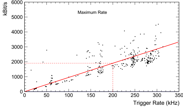
Figure 4.15: Maximum data flow as a function of the trigger rate for all the pp runs. The values are fitted with a linear function to evaluate the value at 200kHz.
