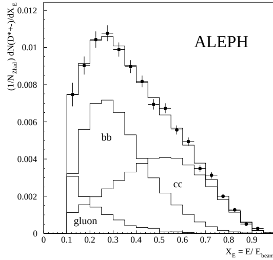
Fig. 1. Energy spectrum of charmed hadrons in Z^0 decays.
