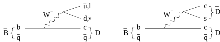
Fig. 2. Charm production in weak decays of b -hadrons.
