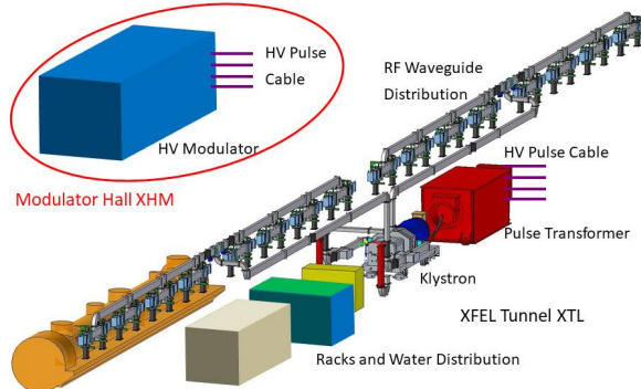
Figure 2: RF station layout.
