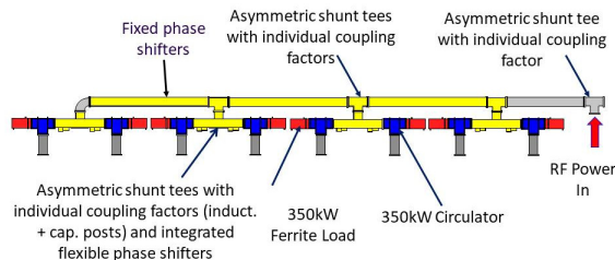
Figure 9: Module waveguide distribution.
