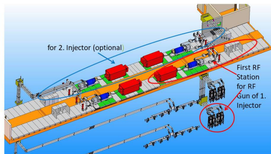
Figure 4: RF stations for injector.
