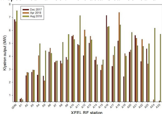
Figure 6: Klystron RF output power for different RF stations at different dates.
