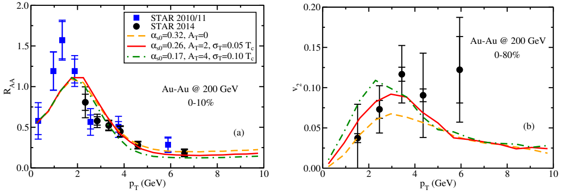
Figure 3. (Color online) Effects of the temperature dependence of the transport coefficient on (a) R_{AA} vs. (b) v_2 of D mesons.
