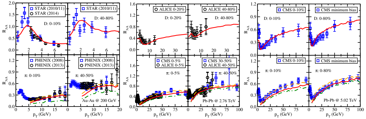
Figure 2. (Color online) R_{AA} of D and \pi from RHIC to the LHC energies. Data are taken from Refs. [2, 35, 36, 37, 38, 39, 40, 41].
