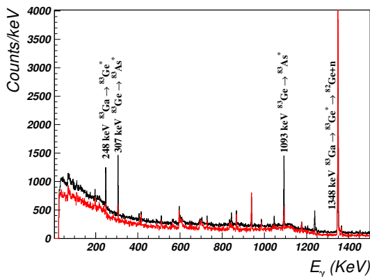
Fig. 4. Beta-gamma (black) and beta-neutron-gamma (grey/red) spectra for decays of A = 83 isobars.
