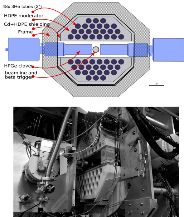
Fig. 2. Neutron detector Hybrid-3Hen at LeRIBSS.
