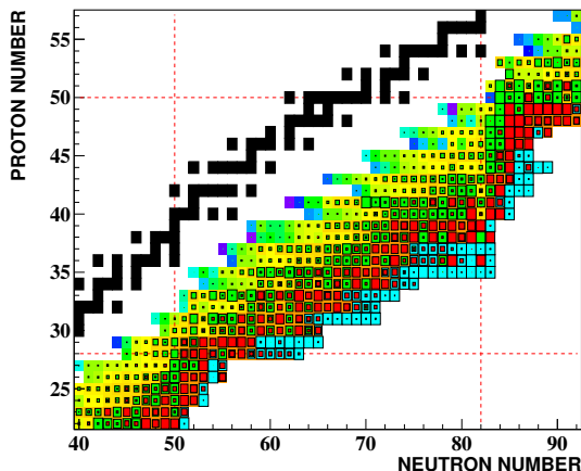
Fig. 1. Beta-delayed neutron emission predicted by Möller et al. [2]. The squares with solid borders indicate beta-delayed \beta 1n , \beta 2n and \beta 3n channels.
