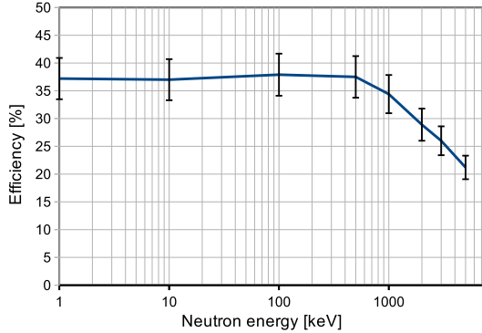
Fig. 3. Neutron detection efficiency for Hybrid-3Hen as modelled by Geant4. The 10% relative error bars are estimated due to Geant4 model uncertainties. Line is to guide the eye.
