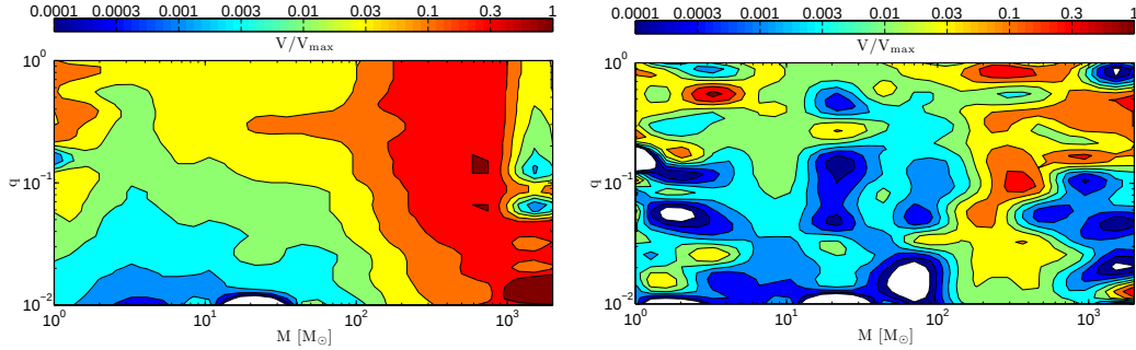
Figure 6.14: Contours of detection probability p := V/V_{\max} as a function of rest mass M and mass ratio q for Advanced LIGO for a source inside the optimal filtering distance horizon, using sine-Gaussian (left panel) and ringdown (right panel) templates for an initial pericenter separation of r_p = 6M .
