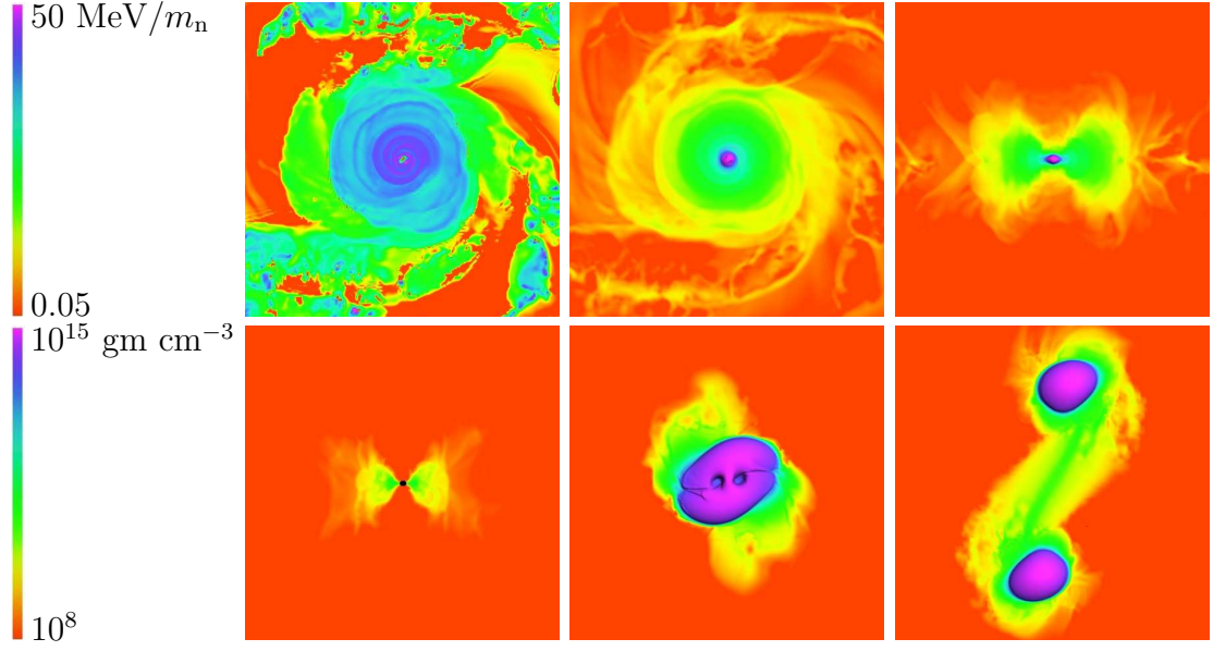
Figure 5.3: Snapshots of thermal specific energy (top left panel) with a logarithmic color scale from 0.05 to 50 MeV/ m_n and rest-mass density (other five panels) from 10^8 to 10^{15} gm cm ^{-3} . The top left and top middle, and bottom middle and bottom right panels show the equatorial plane, while the other two show a perpendicular plane through the center of mass. The top panels show an HMNS with surrounding disk and unbound material from the r_p = 8.75 , HB EOS case at t = 13.3 ms. The bottom panels show, from left to right, a BH and a surrounding disk for the r_p = 7.5 B EOS case at t = 10.2 ms; a merger from the r_p = 7.5 , HB EOS case at t = 3.2 ms; NSs with excited f -mode perturbations post close encounter from the r_p = 10 , HB EOS case at t = 4.1 ms. The first four panels have the same distance scale, where the coordinate radius of the HMNS and BH are \approx 13 and \approx 6 km, respectively. The last two panels share a second distance scale; the coordinate separation between the NSs in the last panel is \approx 73 km.
