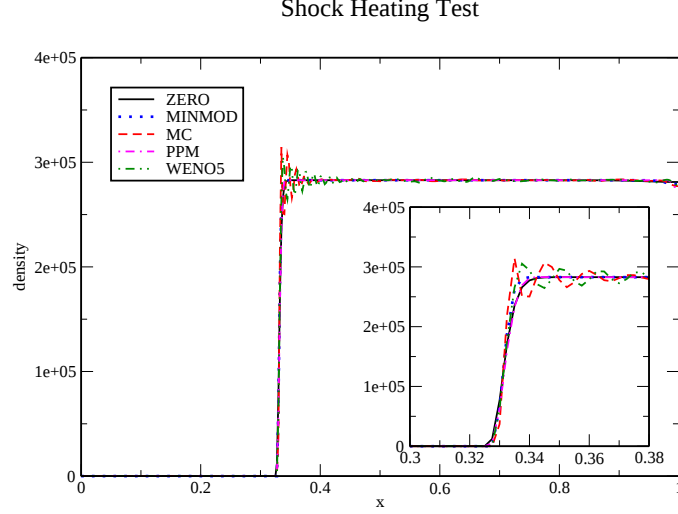
Figure 2.8: Density at t = 2.0 for the shock-heating test with different reconstruction methods and the HLL flux scheme. The inset focuses on the shock front.
