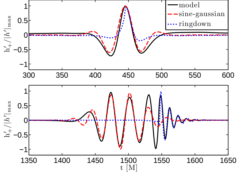
Figure 6.9: Whitened waveforms for a 10 \text{ M}_\odot (top panel) and a 100 \text{ M}_\odot (bottom panel) binary with initial e = 1 and r_p = 5M , along with the (whitened) best-fit template among sine-Gaussian and ringdown templates.
