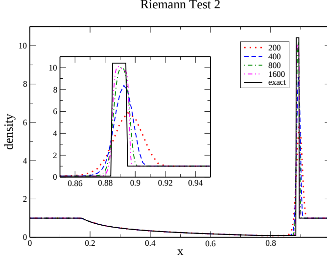
Figure 2.5: Density at t = 0.4 for Riemann Test 2 (RT2) at different resolutions for HLL-WENO5. The average convergence rate in this case is 0.76. The thin shell of material between the shock and the contact is particularly difficult to resolve.
