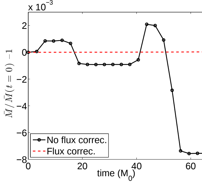
Figure 2.14: The relative variation of the fluid rest-mass ( \bar{M}/\bar{M}(t=0) - 1 ) for a boosted NS test with (dotted, red line) and without (solid black line) flux corrections at mesh refinement boundaries. For this test, the mesh hierarchy is fixed so that at t \approx 20 M_0 the NS has moved from being contained entirely on the finest resolution to being contained entirely on the second finest resolution. At t \approx 60 M_0 the NS has moved from the second to the third finest resolution.
