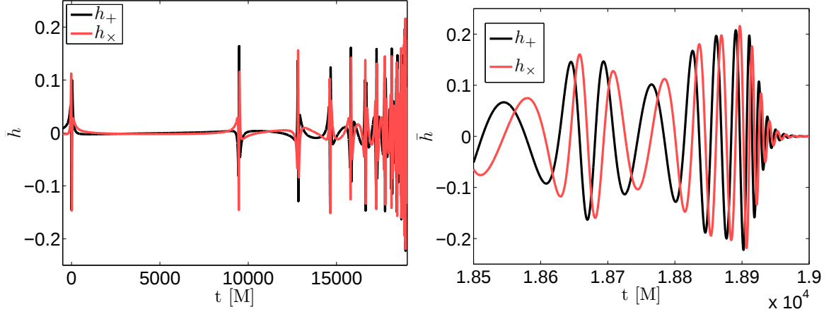
Figure 6.5: GW strain generated with our model and initial conditions r_p = 8 M and e = 1 . The left panel shows the entire waveform, while the right panel shows a zoomed-in view of the end of the waveform.
