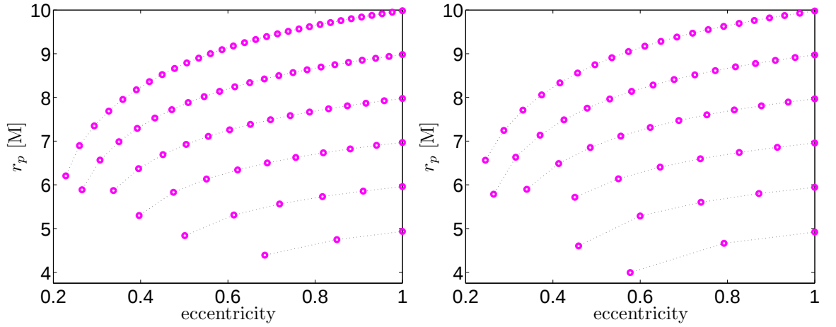
Figure 6.6: Evolution of orbital parameters for a 4:1 (left panel) and an equal mass ratio (right panel) binary. The effective eccentricity is calculated from successive apoapse and periapse distances as e = (r_a - r_p)/(r_a + r_p) .
