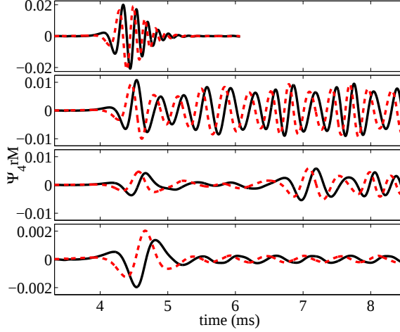
Figure 5.2: Real (solid black) and imaginary (dotted red) components of the Newman–Penrose scalar \Psi_4 on the axis orthogonal to the orbit measured at r = 100M for the r_p = 5, 7.5, 8.75 , and 10 cases with HB EOS.
