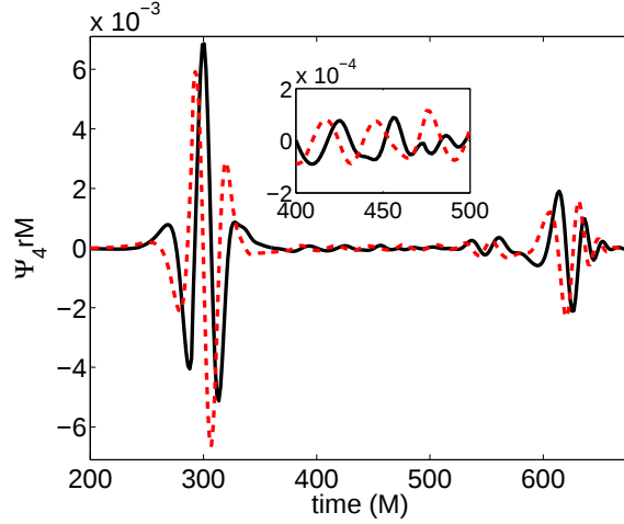
Figure 4.10: The real and imaginary components (solid black lines and red dotted lines) of \Psi_4 on the z-axis (perpendicular to the orbital plane) at r = 70 M for the r_p = 7.0 2H simulation. The large burst at t \approx 300 M comes from the initial fly-by, where the NS becomes extremely distorted (Fig. 4.3) and loses a significant portion of its mass (Fig. 4.7). The smaller pulse at t = 600 M comes from the merger. In between, there is a smaller component of the signal coming from the tidally induced oscillation of the NS.
