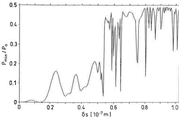
Figure 9. Power loss due to thermal effects: interference minimum as a function of local mirror deformation.
