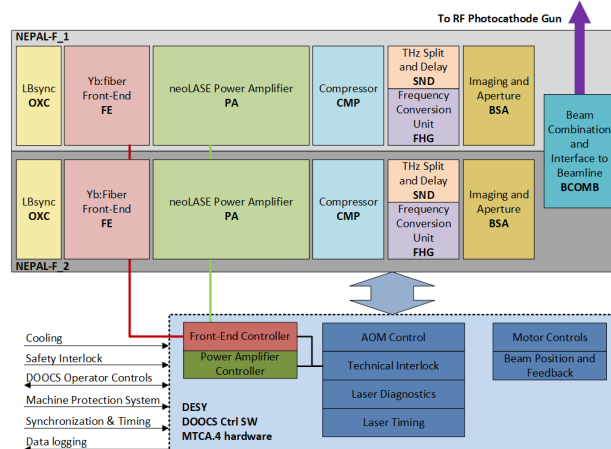
Figure 1: System diagram of the NEPAL-F laser system. The system is composed of two identical laser lines NEPAL-F_1 and NEPAL-F_2 comprising the sub-components Optical Cross Correlator (OXC), Front-End (FE), Power Amplifier (PA), Compressor (CMP), Split and Delay unit (S/D), Frequency conversion (FHG), Beam Shaping Aperture (BSA) and Beam Combination (BCOMB). The laser parameters such as pulse duration, delay, spectrum and phase, burst length and intra-burst repetition rate are remotely controllable via Distribute Object-oriented Control System (DOOCS) [5].
