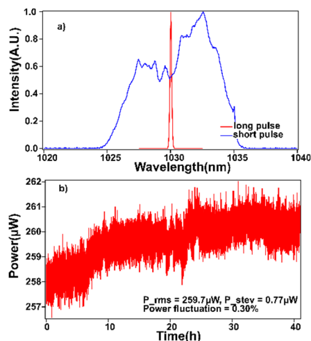
Figure 3: spectrum of the front-end output and power fluctuation (sampling rate: 3.3 Hz).
