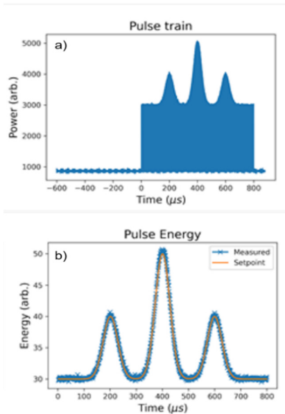
Figure 5: a): The arbitrary generation of pulse train. b): the comparison between the set burst and the measured burst.
