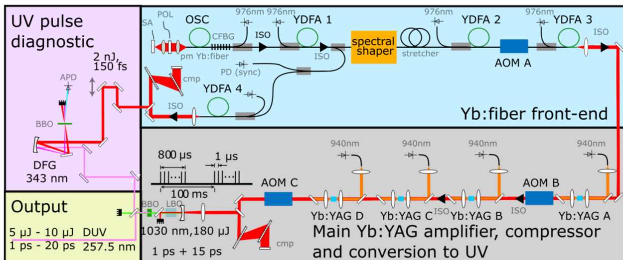
Figure 2: Schematic of one laser branch NEPAL-Fx: SA: Saturable absorber, POL: polarizer, CFBG: Chirp Fiber Bragg Grating, YDFA: Ytterbium doped fiber amplifier ISO: Isolator, AOM: Acoustic Optic Modulator, cmp: compressor, APD: avalanche photodiode.
