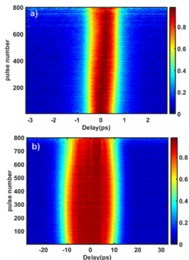
Figure 4: DUV pulse duration characterization by cross-correlation measurement for short pulse operation (a) and long pulse operation (b). Colour bar: Intensity of cross-correlation (normalized).
