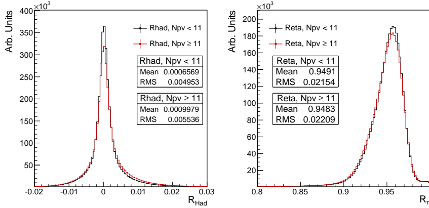
Figure 4.5: Electron hadronic leakage fraction ( R_{Had} ) and transverse shower profile ( R_\eta ) in layer 2 for high and low pile-up conditions. Pile-up is measured here as the number of primary vertices in the event.
