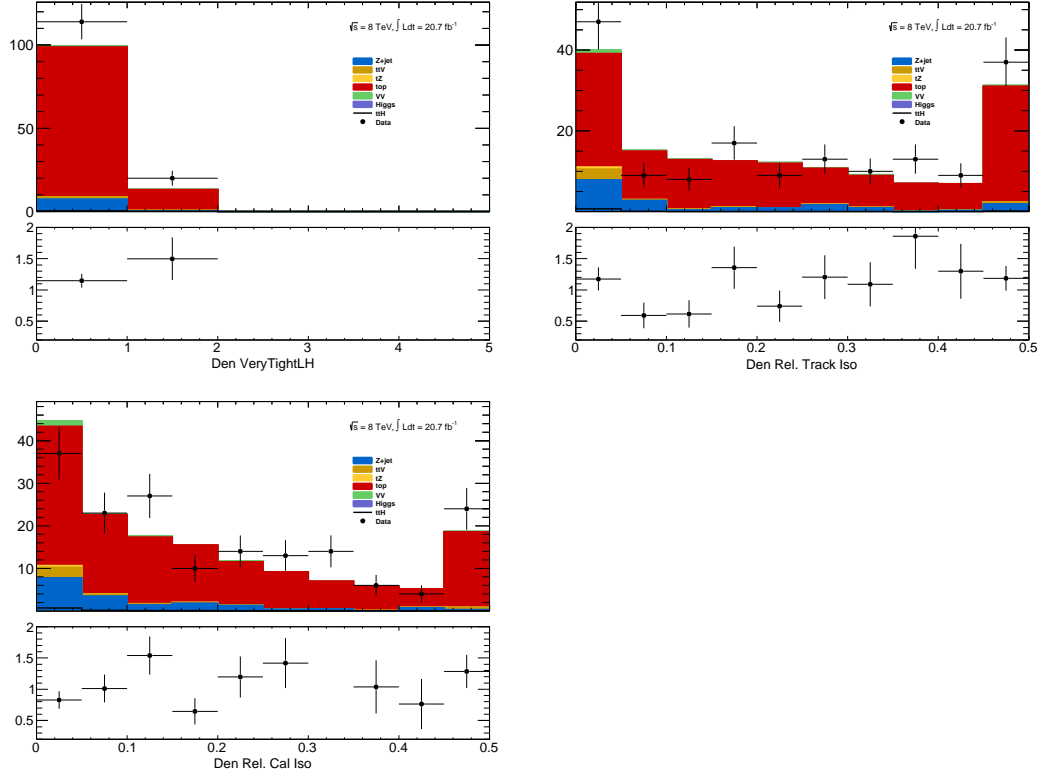
Figure 8.13: Distributions of anti-tight electron variables. The variables presented are, from top left to bottom right, p_T , \eta , VERYTIGHT Likelihood value, ptcone20/p_T , Etcone20/p_T . The plotted regions have the same cuts as the signal region, except the anti-tight electron must fail isolation for the plot of the VERYTIGHT identification word or fail the VERYTIGHT identification word for the plots of the isolation. Data (dots) are compared with a stacked histogram of the various simulated samples: top in red, V +jets (blue), VV (purple) and t\bar{t}V (yellow). The uncertainty on the data distribution is statistical.
