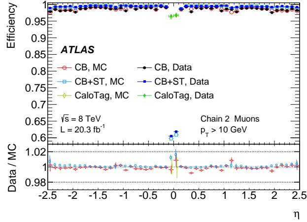
Figure 9.2: Muon identification efficiency in Data and MC as a function of \eta . The CB+ST (combined+segment tagged) operating point is used
