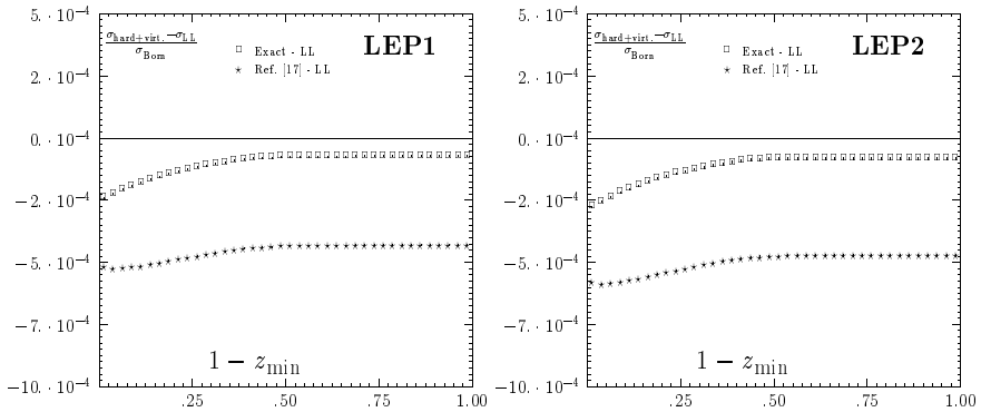
Fig. 1. Monte Carlo results ( 10^6 events) for the \mathcal{O}(\alpha^2) cross section for single photon emission from the electron line. Differences between three matrix elements are shown for the SICAL Wide-Narrow trigger, divided by the Narrow-Narrow Born cross section, with z_{\min} defined as in Fig. 2 of Ref. [9]. The two graphs display results for LEP1 and LEP2 parameters, respectively.
