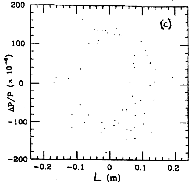
Fig. 7. Longitudinal phase space distributions for beam perturbed by filtered phase noise. L is the distance along the beam from the center of the bucket. (a) Original distribution before noise is introduced. (b) Distribution of circulating beam after 10^6 turns with filtered noise of amplitude \sigma_\phi = 0.015 rads. (c) Original distribution of those particles which hit the crystal after 10^7 turns.
