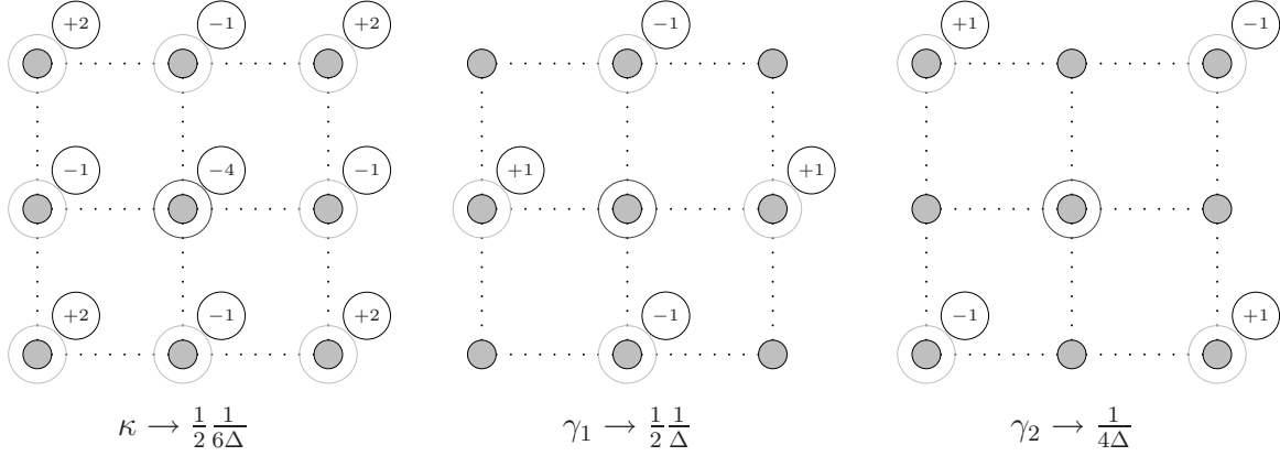
Fig. 2. The finite differencing coefficients for \kappa (left), \gamma_1 (middle) and \gamma_2 (right). E.g. for \kappa we use a formula including 9 points, the multiplicative factor is given at the bottom, the individual coefficients in the circle. Thus for the middle point (0, 0) we get \kappa(0, 0) = \frac{1}{2} \frac{1}{6\Delta} [2[\psi(-1, 1) + \psi(1, 1) + \psi(-1, -1) + \psi(1, -1)] - [\psi(0, 1) + \psi(-1, 0) + \psi(1, 0) + \psi(0, -1)] - 4\psi(0, 0)] .
