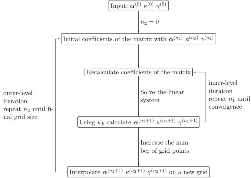
Fig. 1. The outline of the two-level iteration process.
