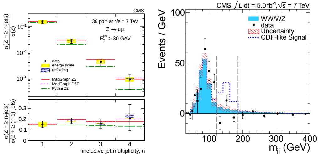
Figure 2: Left: Ratio \sigma(Z + n - jets)/\sigma(Z) in the muon channel compared to expectations from MADGRAPH and PYTHIA. Right: Distribution of the invariant mass spectrum of the leading two jets after subtraction of all SM components except the electroweak diboson WW/WZ. Error bars correspond to the statistical uncertainty. The band represents the systematic uncertainty in the sum of the SM components.
