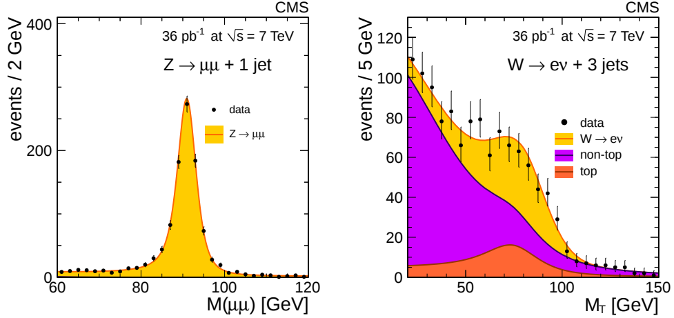
Figure 1: Left: di-lepton mass fit for the Z + 1 jet sample, in the muon channel. Right: fit results for the W(e\nu) + n -jet sample with n=3 in the M_T projection
