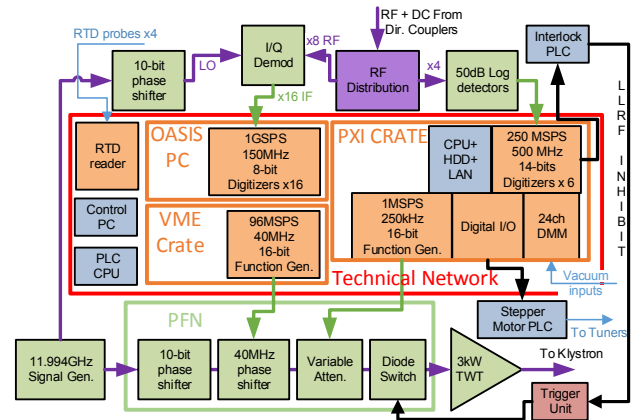
Figure 4: The LLRF network, acquisition and control.
