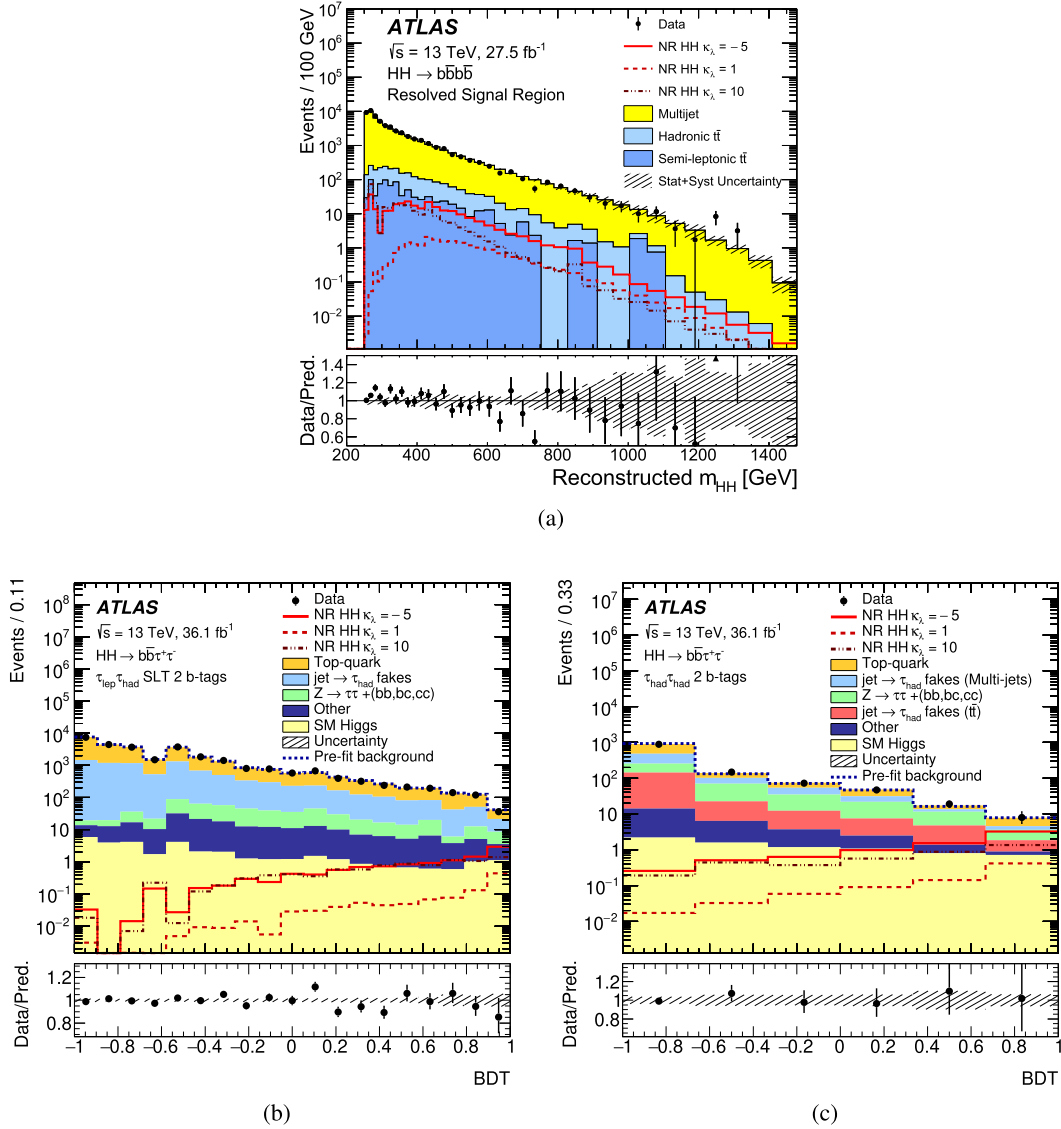
Fig. 3. Final discriminants used in the \kappa_\lambda -scan analysis for the b\bar{b}b\bar{b} and the b\bar{b}t\tau^+\tau^- final states. (a) shows the reconstructed m_{HH} distribution in the b\bar{b}b\bar{b} analysis; backgrounds include data-driven multi-jet processes (Multijet), t\bar{t} \rightarrow W^+W^-b\bar{b} with both W bosons decaying hadronically (Hadronic t\bar{t} ) and t\bar{t} \rightarrow W^+W^-b\bar{b} with at least one of the W bosons decaying leptonically (Semileptonic t\bar{t} ). (b) and (c) show the BDT distributions in the b\bar{b}t\tau^+\tau^- analysis for the \tau_{lep}\tau_{had} and the \tau_{had}\tau_{had} channels, respectively. The main backgrounds are t\bar{t} and single-top-quark production (Top-quark), the background arising from jets faking hadronic \tau -lepton decays (jet \rightarrow \tau_{had} fakes), Z \rightarrow \tau^+\tau^- plus two heavy-flavour jets [ Z \rightarrow \tau\tau + (bb, bc, cc) ], SM single Higgs boson production (SM Higgs) and other minor backgrounds (Other). The shaded area includes the systematic uncertainty of the total background expectation due to the statistics of simulated events and all experimental and theoretical systematic uncertainties. In figures (b) and (c) the uncertainty band is not shown in the upper panes because it is too small to be seen. The signal distribution is overlaid for \kappa_\lambda = -5, 1, 10 and is normalised to its expected yield.
