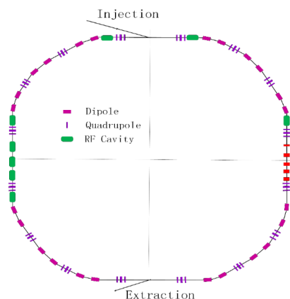
Figure 1: The layout of the cavity in the RCS.
