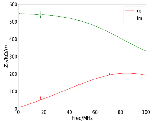
Figure 5: The RCS transverse impedance mode.
