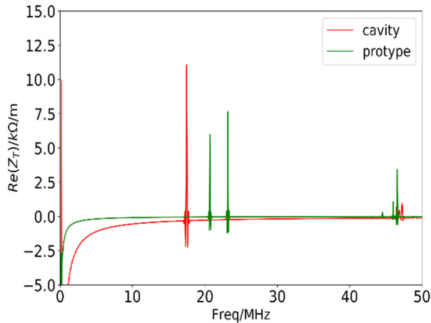
Figure 4: The transverse impedance of the ferrite cavity.
