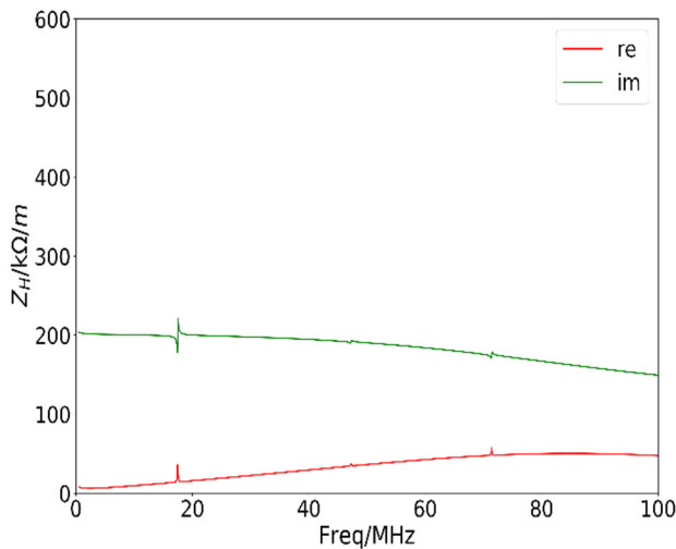
Figure 5: The RCS transverse impedance mode.
