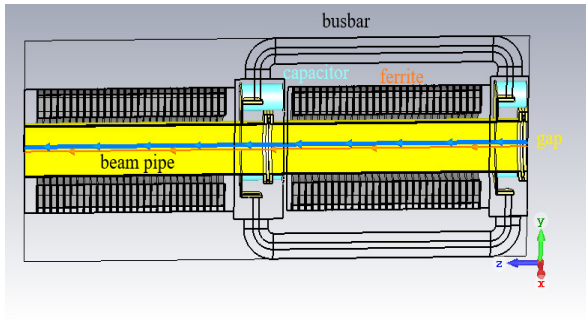
Figure 2: The CST simulation mode of the cavity prototype.
