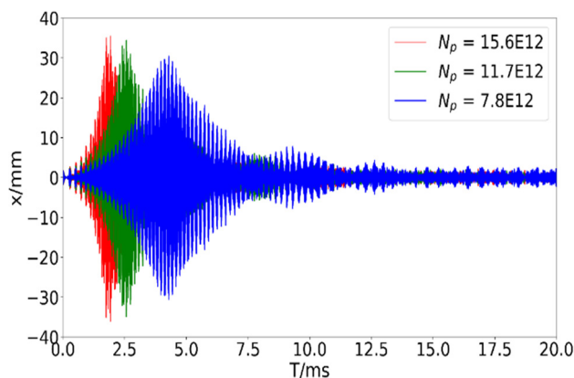
Figure 6: The cavity horizontal impedance drives the beam position with different beam intensity. The two buckets are perfectly filled with two bunches and the number of the legend is protons of two bunches.
