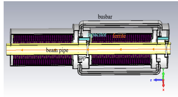
Figure 3: The CST simulation mode of the cavity.
