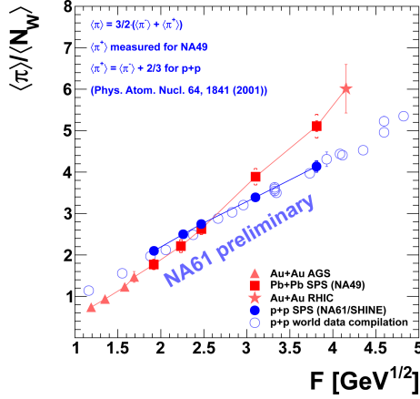
Fig. 5. Mean pion multiplicity per wounded nucleon in central Pb+Pb and p + p collisions. The NA61/SHINE points (full/blue) agree very well with the world data (empty/blue). The NA61/SHINE data will provide reference to the rest of the NA61/SHINE ion programme. The data is plotted in function of the Fermi's energy measure F = \left[ \frac{(\sqrt{s_{NN}} - 2m_N)^3}{\sqrt{s_{NN}}} \right]^{1/4} .
