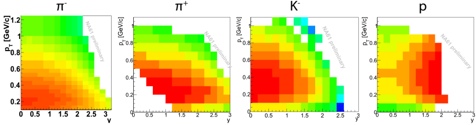
Fig. 3. h^- ( \pi^- ) and dE/dx ( \pi^+ , K^- , p ) identified particle spectra at 158 A GeV/ c .
