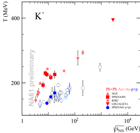
Fig. 4. Inverse slope parameter of m_T spectra in Pb+Pb and p + p collisions. The NA61/SHINE data provide reference to the data from heavy ion collisions.
