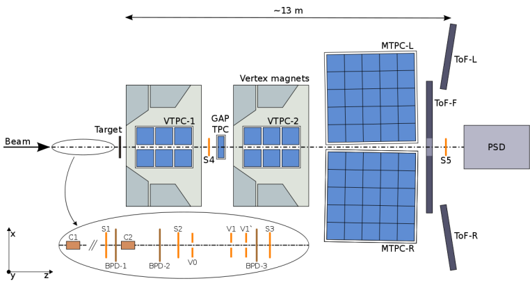
Fig. 2. The NA61/SHINE detector set-up.
