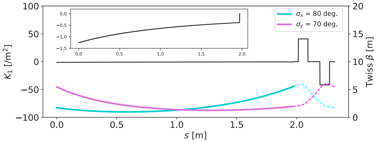
Figure 3. The lattice function of the first DLS section and two quadrupole magnets and the Twiss-beta function under periodic boundary conditions.
