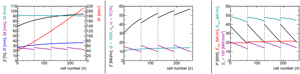
Figure 1. The S-band DLS cell parameters; first DLS ( n=1-64 ), second DLS ( n=65-128 ), third DLS ( n=129-189 ) and fourth DLS ( n=190-250 ).
