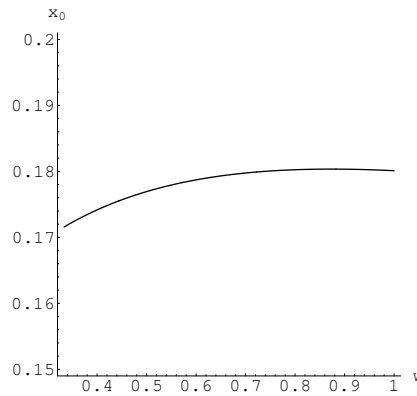
Fig. 1. The root x_0 as function of parameter w .
