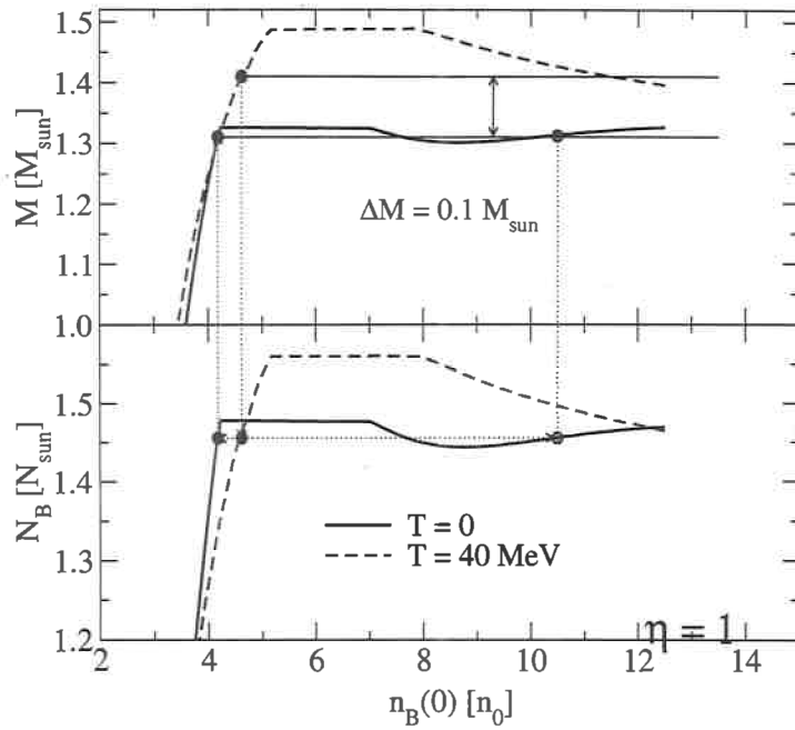
FIG. 9: Cooling an isothermal quark star configuration with initial mass M = 1.41 M_{\odot} at temperature T = 40 \text{ MeV} under conservation of the given baryon number N = 1.46 N_{\odot} down to T = 0 leads to a mass defect \Delta M = 0.1 M_{\odot} for the strong coupling case ( \eta = 1.0 ). Due to the twin structure at T = 0 , two alternatives for the final state can be attained, a homogeneous 2SC quark star or a dense 2SC-CFL quark hybrid star.
