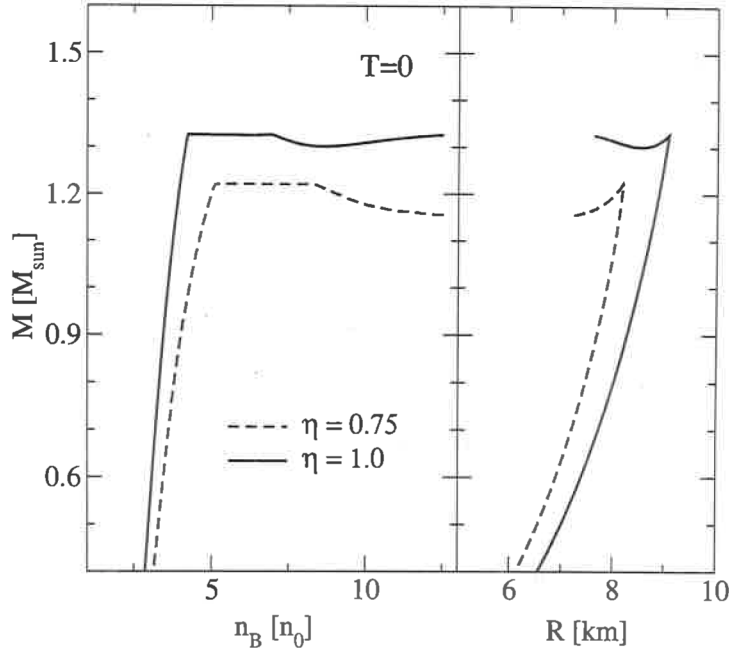
FIG. 8: Sequences of cold quark stars for the three-flavor quark matter equation of state described in the text. The rising branches in the mass-central density relation (left panel) indicate stable compact object configurations. The mass-radius relations (right panel) show that the three-flavor quark matter described in this paper leads to very compact selfbound objects. For intermediate diquark coupling, \eta = 0.75 , stable stars consist of a mixed phase of NQ-2SC matter with a maximum mass of 1.21 M_{\odot} (dashed line). At higher densities a phase transition to CFL quark matter occurs, which entails a collapse of the star. For strong coupling, \eta = 1 , the low density quark matter is in the 2SC phase and corresponding quark stars are stable up to a maximum mass of 1.326 M_{\odot} (solid line). The phase transition to CFL quark matter entails an instability, which at T = 0 leads to a third family of stable stars for central densities above 9n_0 and a mass twin window of 1.301 - 1.326 M_{\odot} .
