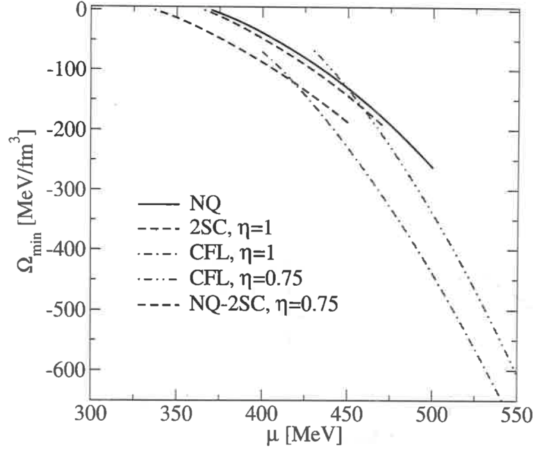
FIG. 6: Minima of the thermodynamical potential for neutral three-flavor quark matter at T = 0 as a function of the quark chemical potential. Note that at a given coupling \eta the state with the lowest \Omega_{\min} is attained and the physical pressure is P = -\Omega_{\min} .
