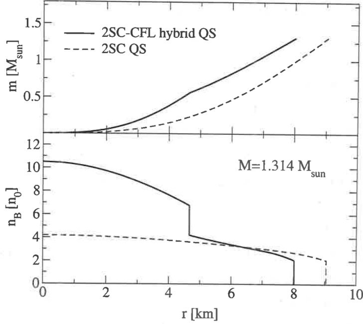
FIG. 10: Structure of two quark star (QS) configurations with M = 1.314 M_{\odot} (mass twins) for the three-flavor quark matter equation of state described in the text in the case of strong coupling ( \eta = 1 ). The low-density twin has a radius of 9 km and is a homogeneous 2SC quark star, the high-density twin is more compact with a radius of 8 km and consists of a CFL quark matter core with 4.65 km radius and a 2SC quark matter shell.
