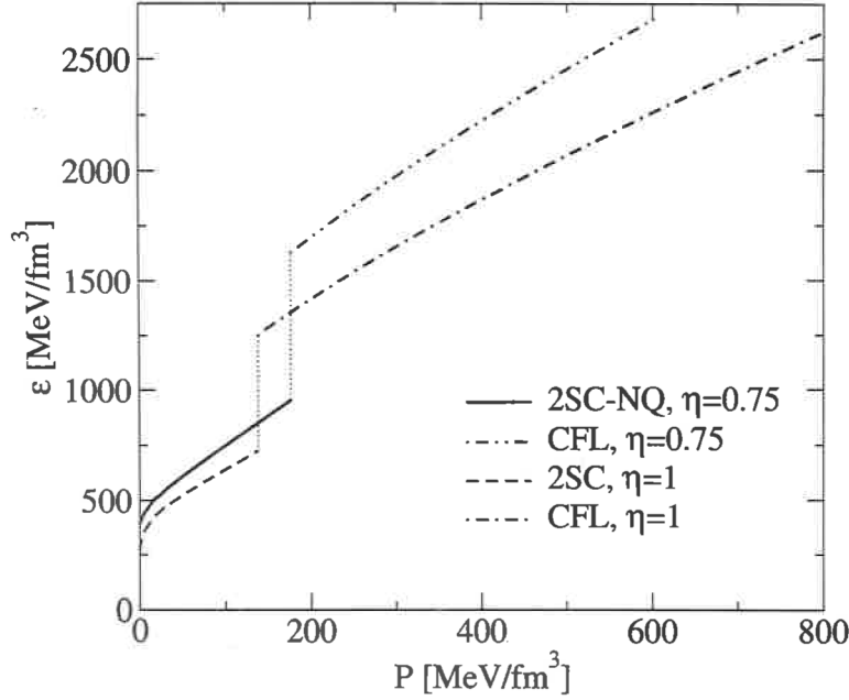
FIG. 7: Equation of state for three-flavor quark matter at T = 0 with first order phase transitions. For intermediate diquark coupling ( \eta = 0.75 ): from the mixed NQ-2SC phase to the CFL phase. For strong diquark coupling ( \eta = 1 ): from the 2SC phase to the CFL phase.
