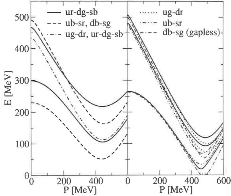
FIG. 3: Quark-quark quasiparticle dispersion relations. For \eta = 0.75 , T = 0 , and \mu = 465 MeV (left panel) there is a forbidden energy band above the Fermi surface. All dispersion relations are gapped at this point in the \mu - T plane, see Fig. 5. There is no forbidden energy band for the ub - sr , db - sg , and ur - dg - sb quasiparticles for \eta = 1 , T = 59 MeV, and \mu = 500 MeV (right panel). This point in the \mu - T plane constitutes a part of the gapless CFL phase of Fig. 6.
