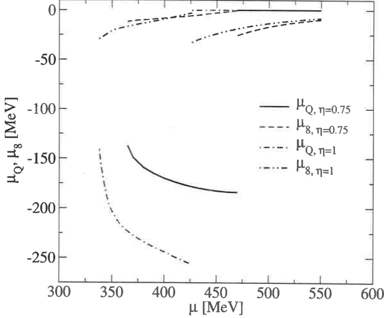
FIG. 2: Chemical potentials \mu_Q and \mu_8 at T = 0 for both values of the diquark coupling, \eta = 0.75 and \eta = 1 . All phases considered in this work have zero n_3 color charge for \mu_3 = 0 . Hence \mu_3 is omitted in the plot.
