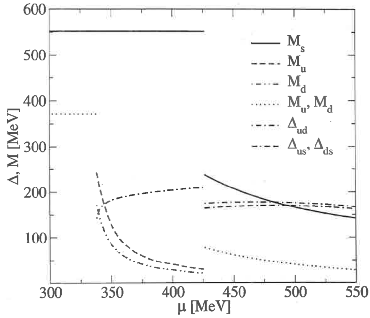
FIG. 1: Gaps and dynamical quark masses as functions of \mu at T = 0 for intermediate diquark coupling, \eta = 0.75 (upper panel) and for strong diquark coupling, \eta = 1 (lower panel).
