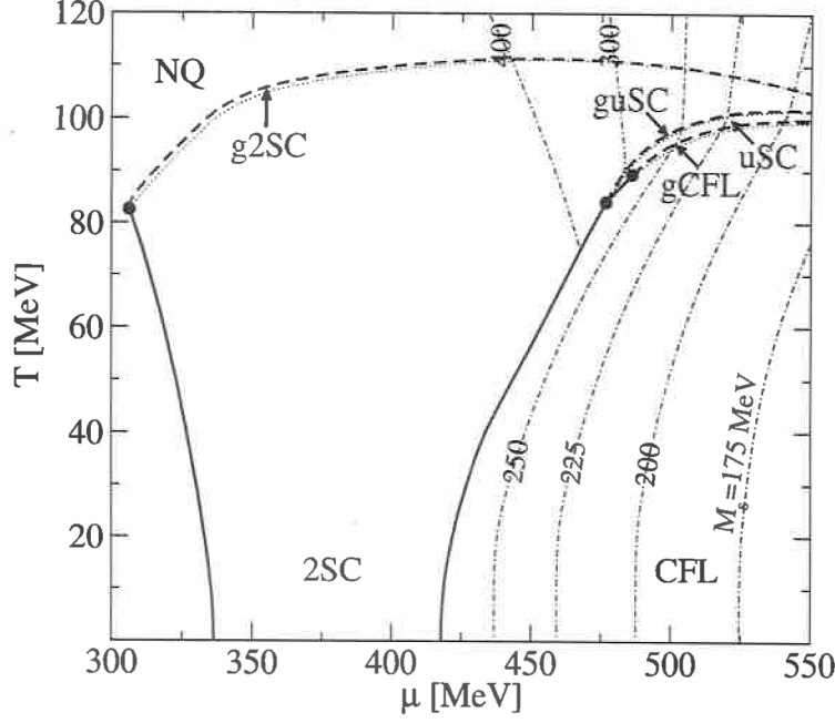
FIG. 5: Phase diagram of neutral three-flavor quark matter for strong diquark coupling, \eta = 1 . Line styles as in Fig. 5.
