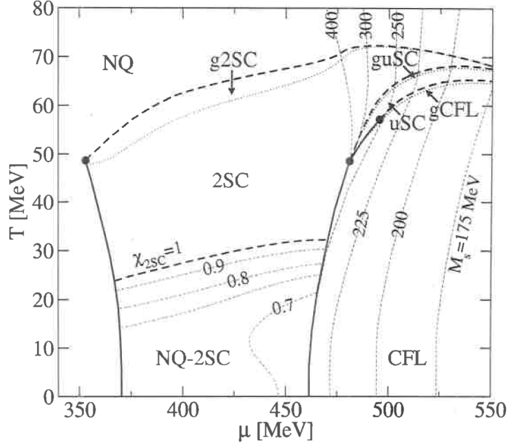
FIG. 4: Phase diagram of neutral three-flavor quark matter for intermediate diquark coupling, \eta = 0.75 . First-order phase transition boundaries are indicated by bold solid lines, while thin solid lines correspond to second-order phase boundaries. The dashed lines indicate gapless phase boundaries. The volume fraction, \chi_{2SC} , of the 2SC component of the mixed NQ-2SC phase is denoted with thin dotted lines, while the constituent strange quark mass is denoted with bold dotted lines.
