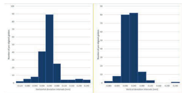
Figure 3: Histograms of the deviations for the Booster.
