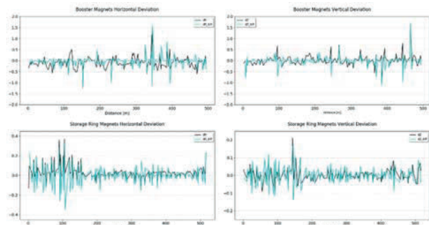
Figure 5: Derivatives of the magnets and girders deviations for the Booster (top) and Storage Ring (bottom).
