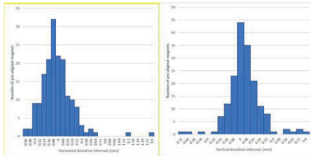
Figure 1: Histograms of the deviations for the Booster.
