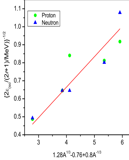
FIG. 1: Mass dependence of the reduced spin-orbit splitting.
