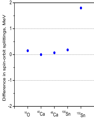
FIG. 2: Difference between spin-orbit splitting of proton and neutron for N = Z and N \neq Z nuclei.
