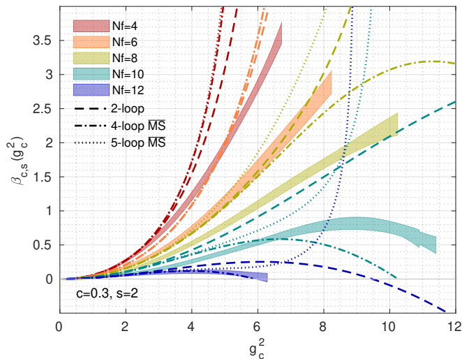
FIG. 1. Comparison of the step-scaling functions for N_f = 4, 6, 8, 10 and 12 using the c = 0.300 scheme and scale change s = 2 .
