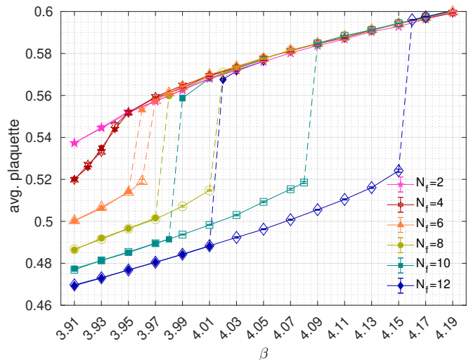
FIG. 7. Comparison of the plaquette on 8^4 volumes as the function of the bare coupling for N_f = 2 - 12 flavors. By performing starts from weak and strong coupling we are resolving a hysteresis for N_f \geq 6 . Both the discontinuity and the hysteresis width grows with increasing flavor number.
