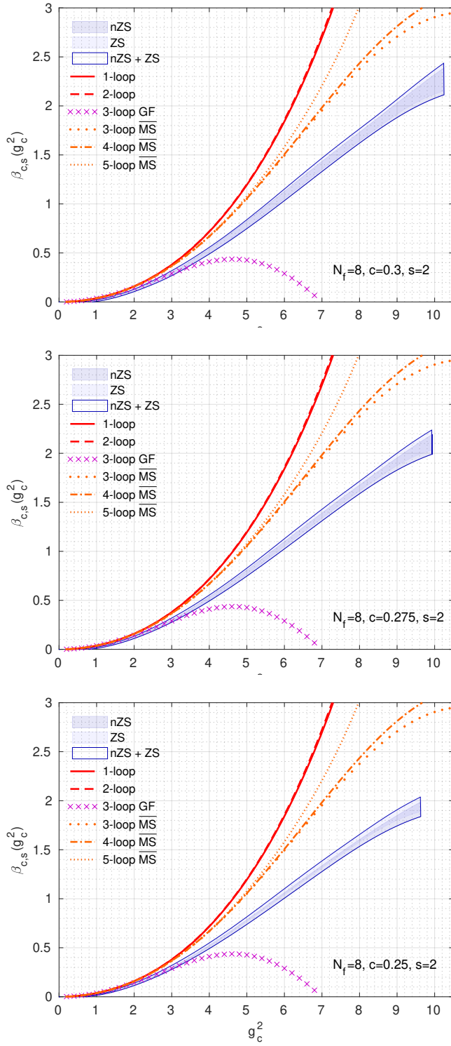
FIG. 6. Comparison of our final N_f = 8 continuum results obtained from our preferred (n)ZS data set for c = 0.300 (top), 0.275 (middle), and 0.250 (bottom) to universal 1- and 2-loop perturbative predictions (red), 3-loop perturbative predictions in the gradient flow scheme (purple) and 3-, 4-, and 5-loop \overline{\text{MS}} scheme predictions (orange).
