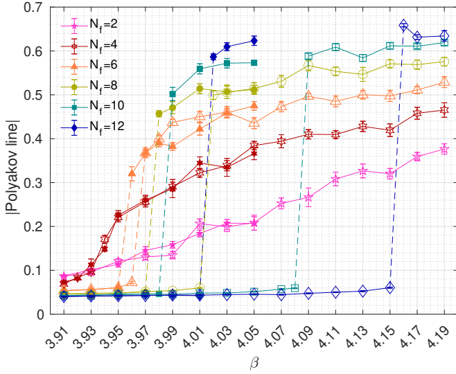
FIG. 8. Comparison of the absolute value of the Polyakov line on 8^4 volumes as the function of the bare coupling for N_f = 2 - 12 flavors. By performing starts from weak and strong coupling we are resolving a hysteresis for N_f \geq 6 . Both the discontinuity and the hysteresis width grows with increasing flavor number.
