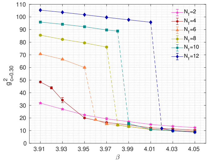
FIG. 2. The renormalized gauge coupling determined using Symanzik gauge action, Zeuthen flow, and Symanzik operator in the c = 0.30 scheme on 8^4 volumes as the function of the bare coupling for N_f = 2 - 12 flavors.
