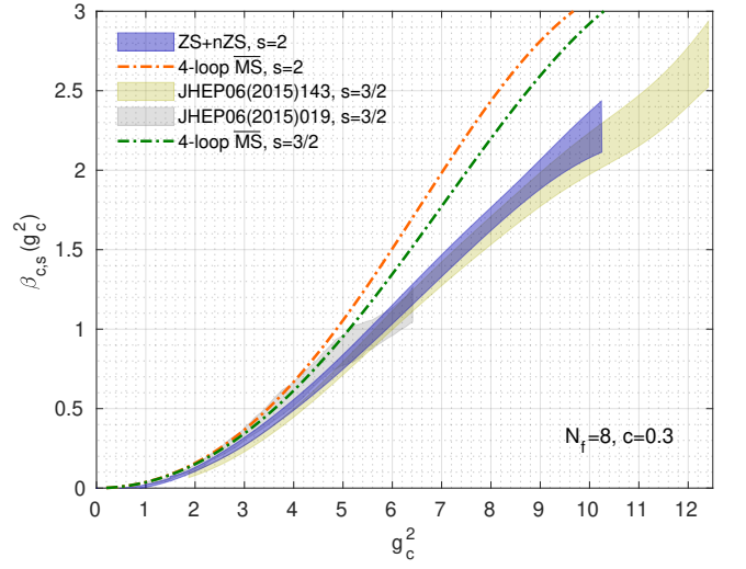
FIG. 10. Comparison of our N_f = 8 continuum results obtained from our preferred (n)ZS data set for c = 0.300 to the nonperturbative results obtained by Hasenfratz et al. [4] and the Lattice Higgs Collaboration (LatHC) [5]. While our results are based on the scale change s = 2 , both prior studies used s = 3/2 .
