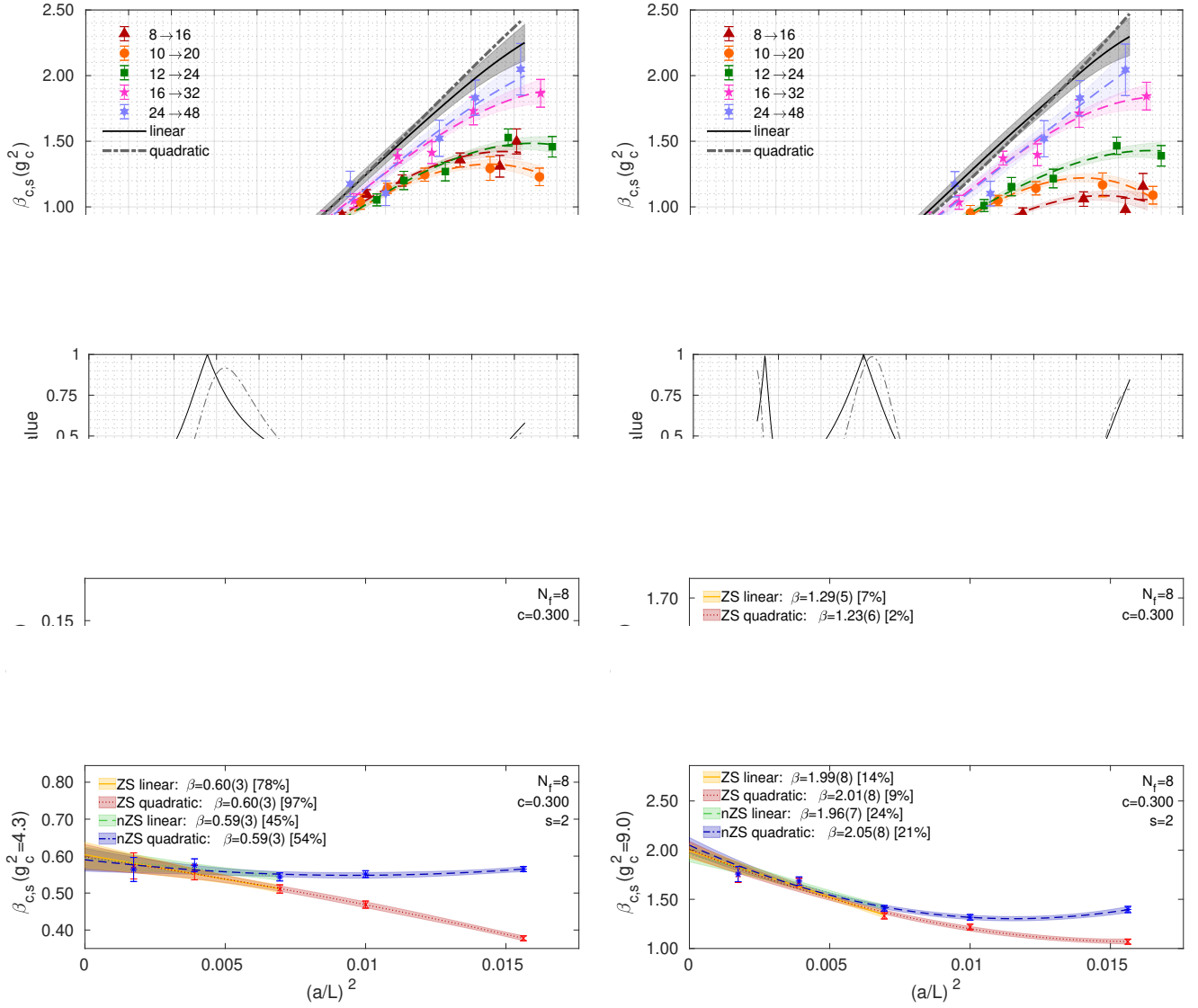
FIG. 4. Discrete step-scaling \beta -function for N_f = 8 in the c = 0.300 gradient flow scheme for our preferred nZS (left) and ZS (right) data sets. The symbols in the top row show our results for the finite volume discrete \beta function with scale change s = 2 . The dashed lines with shaded error bands in the same color of the data points show the interpolating fits. We consider two continuum limits: a linear fit (black line with gray error band) in a^2/L^2 to the three largest volume pairs and a quadratic fit to all volume pairs (black dash-dotted line). The p -values of the continuum extrapolation fits are shown in the plots in the second row. Further details of the continuum extrapolation at selected g_c^2 values are presented in the small panels at the bottom where the legend lists the extrapolated values in the continuum limit with p -values in brackets. Only statistical errors are shown.
