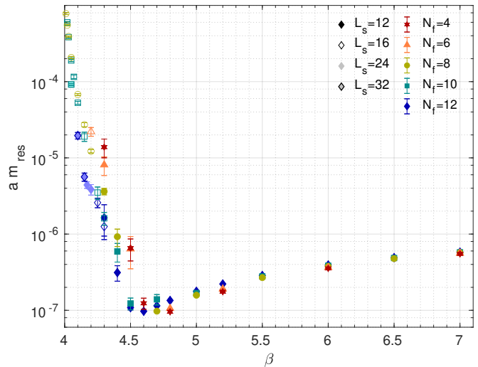
FIG. 3. Residual mass am_{\text{res}} as a function of the bare coupling \beta determined on (L/a)^4 volumes with L/a = 32 for SU(3) gauge systems with N_f = 4, 6, 8, 10 , or 12 flavors. Different colors and symbols distinguish the number of flavors; filled, open, shaded, or framed markers denote the extent L_s of the fifth dimension for MDWF.
