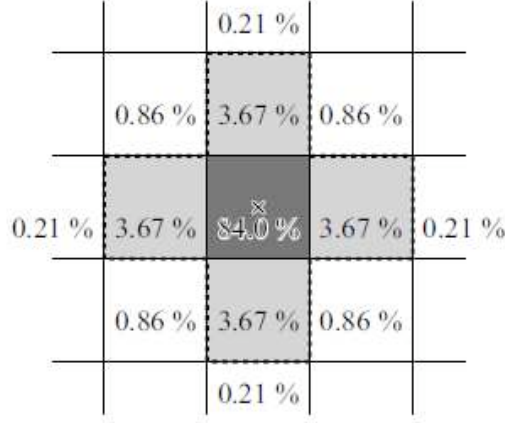
Figure 3.6: An example of expected shower energy fraction in towers in the case of perpendicular hit of photon on the center of a tower. Surrounded five towers by dotted lines are used for E_{core} calculation.
