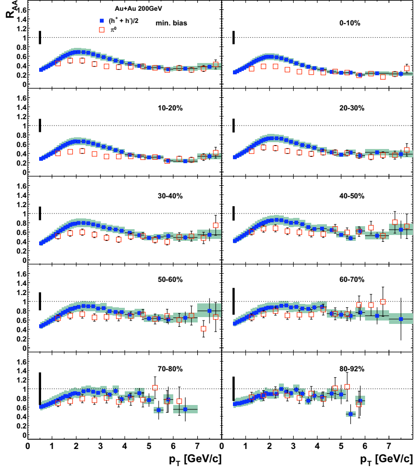
Figure 5.11: \pi^0 R_{AA}(p_T) compared to inclusive charged hadron R_{AA}(p_T) in several centrality selections [86].
