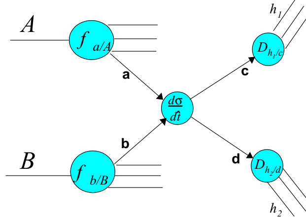
Figure 1.8: Schematic representation of a high- p_T reaction factorized into parton distribution functions ( f ), parton fragmentation functions ( D ), and a hard-scattering subprocess.
