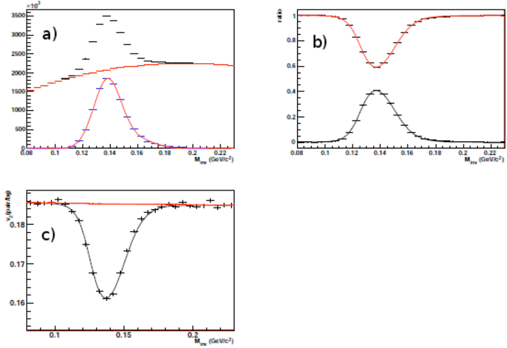
Figure 4.6: An example showing the procedures of invariant mass method in centrality 20-30% and p_T \in 2.0 -2.5 GeV/c. a) shows the invariant mass distributions for total pairs (black), background (red) and signal (blue fitted with pink Gaussian curve). b) shows the ratios N_{BG}/N_{pair} (red) and N_{sig}/N_{pair} (black). c) shows the fit to v_2^{pair} (black) and the red curve is the background v_2(M_{inv}) .
