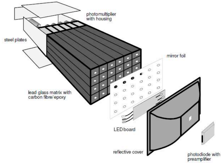
Figure 2.6: Interior view of a PbGl module.
