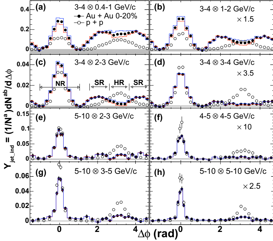
Figure 1.13: Two particle azimuthal angular correlations in Au+Au 0-20% collisions [59]. The away side is suppressed when partner p_T > 3 GeV/c. Below double peak structures at away side imply medium response to the fast moving parton.
