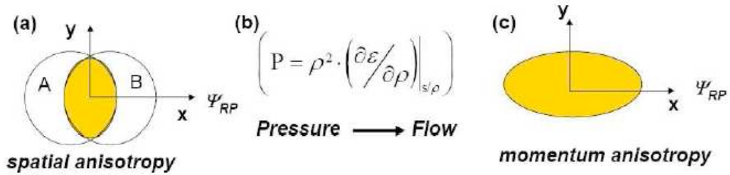
Figure 1.5: Schematic illustration of how pressure gradient converts initial spatial asymmetry to final state momentum anisotropy (elliptic flow).
