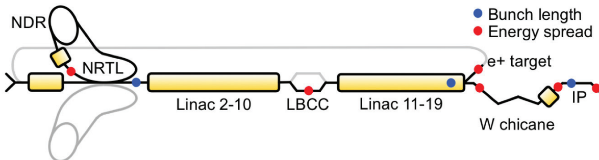
Figure 1: The FACET accelerator complex. Yellow boxes represent accelerator sections, including those in the injector, the NRTL compressor, Sectors 2-10, Sectors 11-19, and the eventual location of the X-band transverse cavity to be installed in the W chicane. Blue dots show the location of bunch length diagnostics in Sectors 2, 18, and 20, and red dots show the locations of energy spectrometers.
