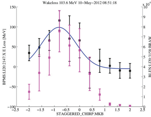
Figure 5: Chirp scan showing 103 MeV of energy loss to longitudinal linac wakefields. The purple signal is the amplitude of the THz table foil pyro detector.
