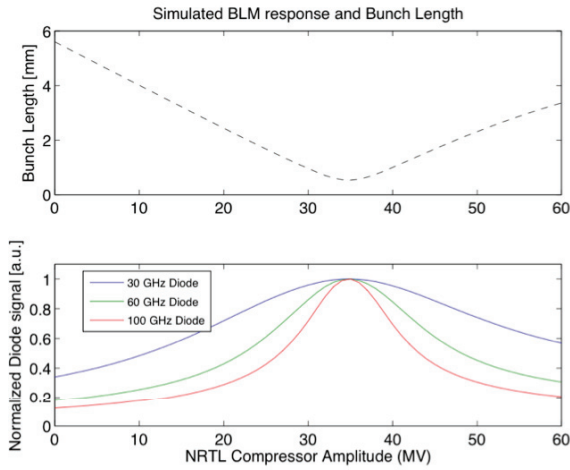
Figure 2: Simulated gap monitor response vs. compressor klystron RF voltage.
