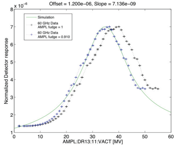
Figure 3: Simulated 60 GHz diode response and measured data from compressor voltage scan.
