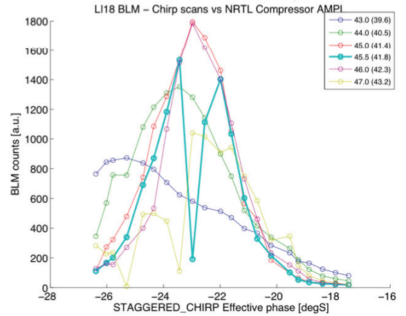
Figure 4: Data from the Sector 18 BLM. Here the phase of Sectors 2-11 is scanned at various NRTL compressor settings (fudged voltage in parentheses). The light blue curve appears to be the optimum – at the central point, saturation of the GADC causes the apparent signal to drop.
