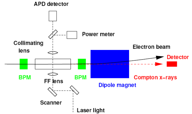
Figure 1: Schematic of the LW IP region.
