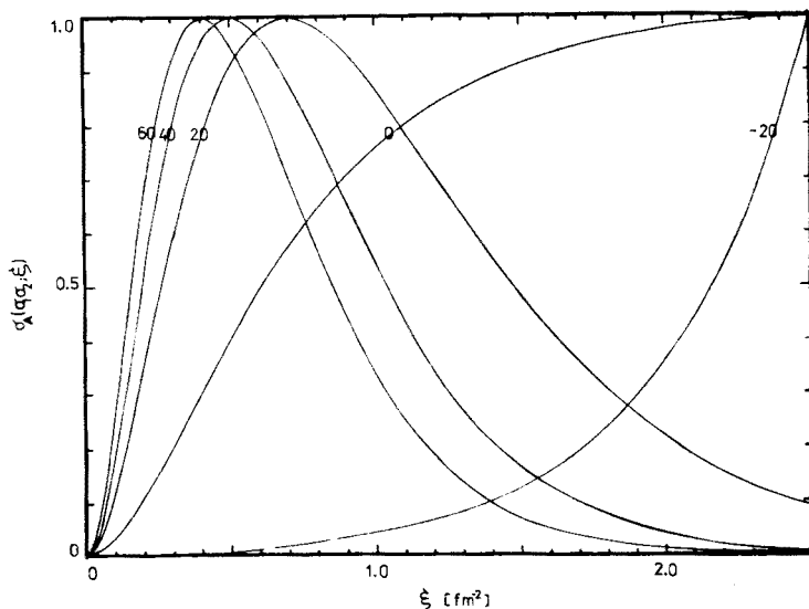
Fig. 1. The differential K lbig-Margolis (KM) cross-sections \sigma_A(\sigma_1 \sigma_2, \xi) for \sigma_1 = 40 mb and different values of the parameter \sigma_2 (60, 40, 20, 0, -20 mb) which labels the curves. Each curve is normalized to 1 at its maximum
