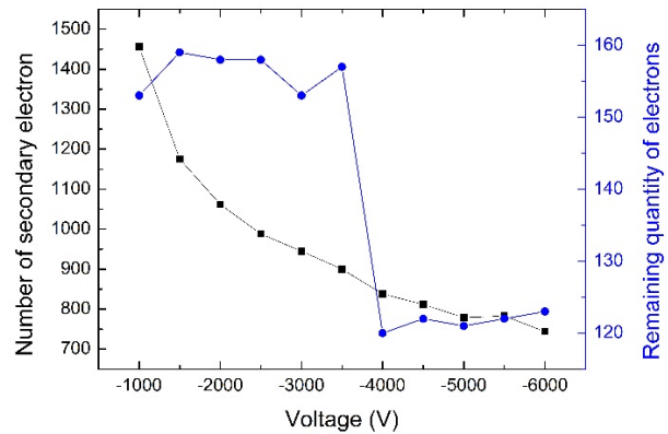
Figure 5: The results of secondary electron simulation.
