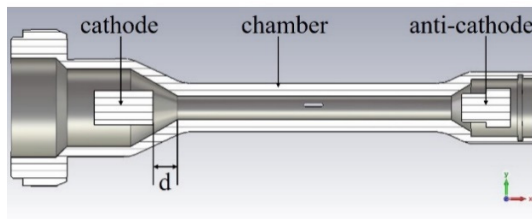
Figure 3: Cold cathode ion source model for simulation.
