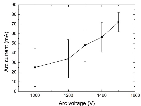
Figure 6: Arc current vs. arc voltage.
