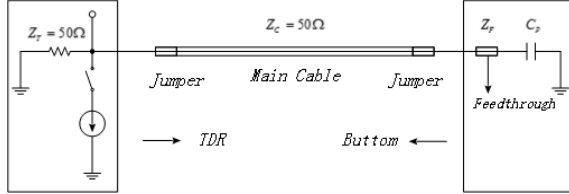
Figure 3: The schematic of the TDR of a signal channel.
