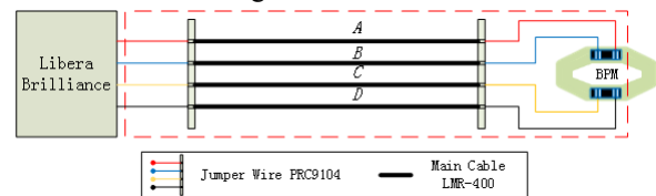
Figure 2: The schematic of the BPM signal channels.
