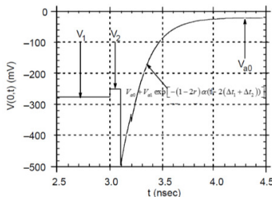
Figure 4: The theoretical waveform of BPM signal channel with button.
