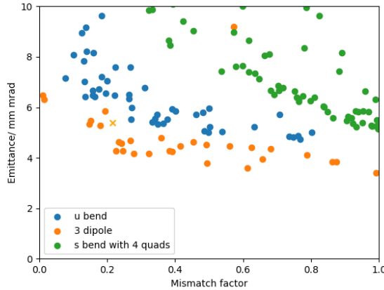
Figure 3: The Pareto fronts resulting from the optimisations. An example solution has been marked with an x. This is a 2D projection of the 3D Pareto front to show two of the variables. The bunch length is not shown. The front has been zoomed into the region of interest but extends beyond the bounds of the plot.
