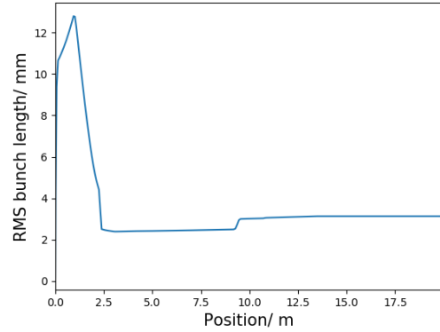
Figure 5: The RMS bunch length along the example injection line.
