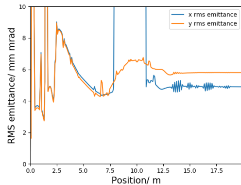
Figure 6: The transverse emittances along the the example injector.
