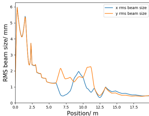
Figure 4: The rms transverse beam sizes along the example injection line.
