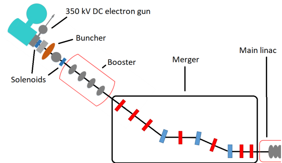
Figure 1: The layout of the injector with an example of a possible merger scheme.
