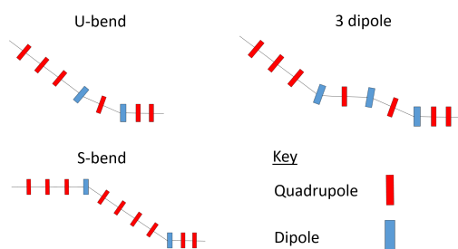
Figure 2: The merger schemes investigated in this proceeding.
