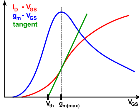
Figure 2.8: Threshold voltage extraction using the linear extrapolation method.
