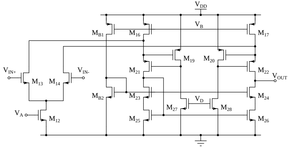
Figure 4.23: Schematic diagram of the first amplifying stage using a high-swing cascode current sink.
