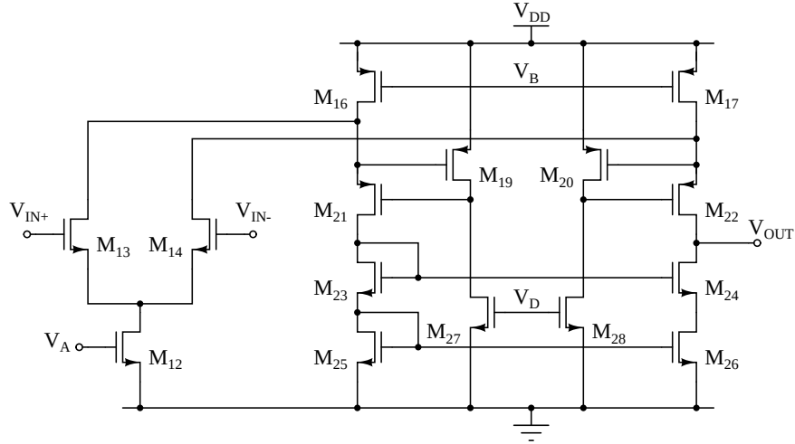
Figure 4.9: Schematic diagram of the first amplifying stage using a cascode current sink.
