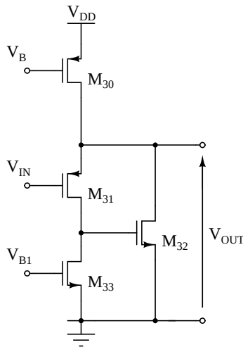
Figure 4.24: Schematic diagram of the super source follower circuit.
