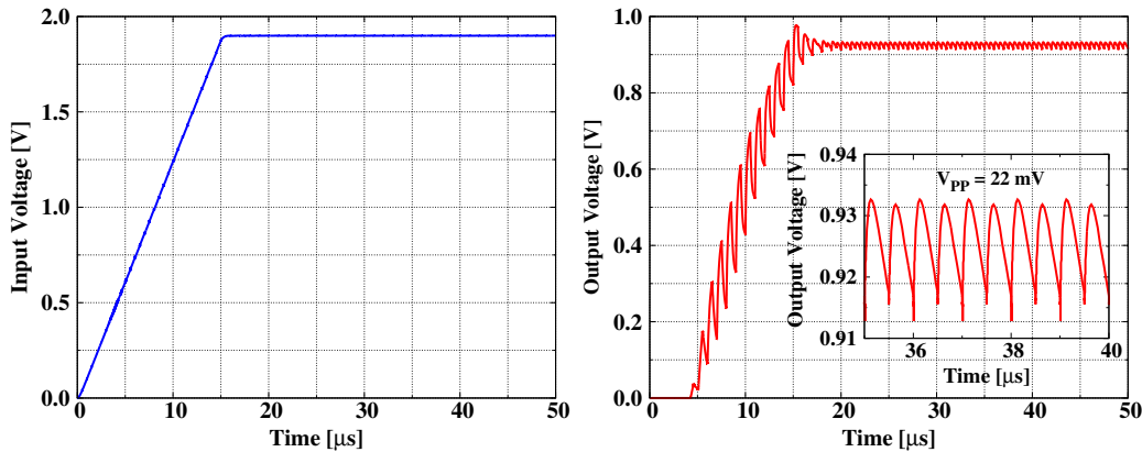
Figure 3.26: Simulated time response of the switched capacitor DC-DC step-down converter.
