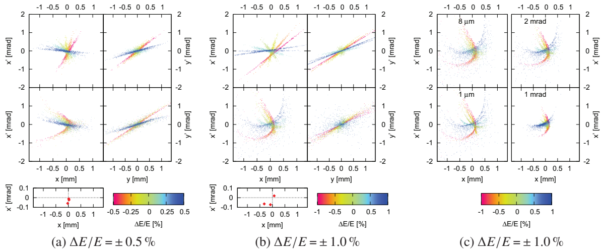
Figure 3: Phase space distributions at the end of the beam transport line for seven monoenergetic beamlets and the average x and x' with \Delta E/E (a) \pm 0.5\% and (b) \pm 1.0\% , at the top is the uncorrected, at the bottom the corrected phase space distribution. (c) Variation of the source size and the divergence for an energy spread of \pm 1\% . left : The source size is set to 1\mu\text{m} , and 8\mu\text{m} with \sigma_{x'} = 2.5\text{ mrad} . right : The divergence is set to 2.0\text{ mrad} and 1.0\text{ mrad} with \sigma_x = 4\mu\text{m} .
