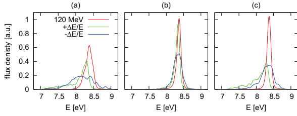
Figure 4: Undulator radiation spectra for monoenergetic beamlets with the different energy spread and initial divergence: \Delta E/E = 0.5\% , (a) \sigma_{x'} = 2.5\text{ mrad} and (b) \sigma_{x'} = 1.0\text{ mrad} , respectively; (c) \Delta E/E = 1.0\% , \sigma_{x'} = 1.0\text{ mrad} . Displayed is the central, the minimum and the maximum energy. The entrance position in x is not optimized in this case.
