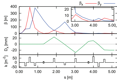
Figure 2: Layout of the dispersive transport system. The inset shows a zoom on the beta functions.
