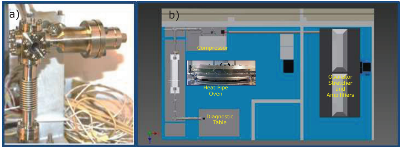
Figure 1: Layout of scaled laser pulse propagation study. a) Photograph of the 3.5 cm rubidium cell used for the quasilinear pulse elongation study. b) CAD layout of the MPP laser / plasma room for phase B of the laser pulse propagation investigation.
