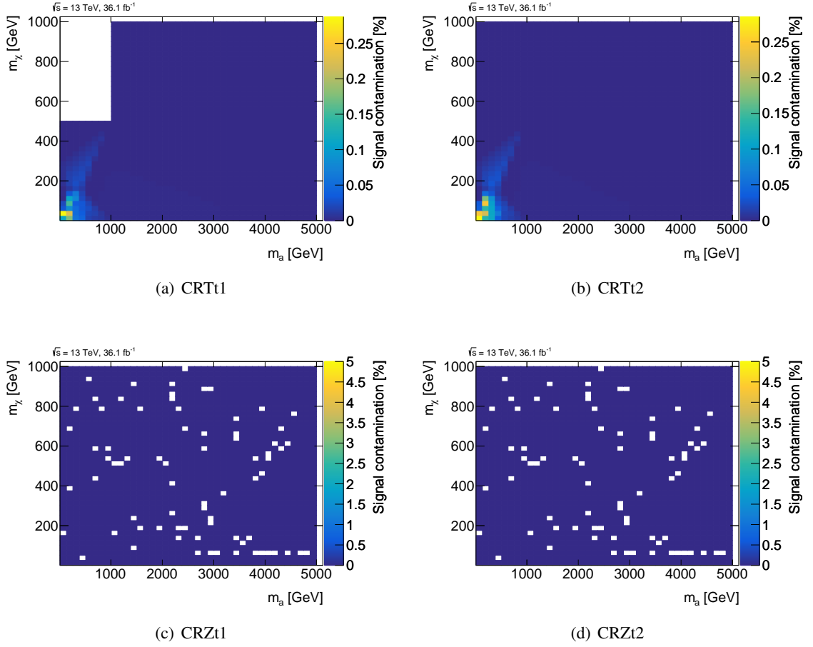
Figure C.7: Expected signal contamination for WIMP pair production via a pseudoscalar mediator in the t\bar{t} and Z +jets CRs.
