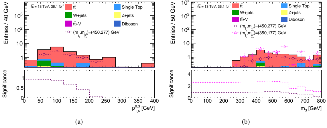
Figure 11.22: Simulated distributions of p_{T,b}^{0,S} (a) and m_S (b) after applying the basic requirements summarised in Table 11.1 as well as p_T^{ISR} > 400 GeV, p_T^{4,S} > 50 GeV and |\Delta\phi_{ISR,E_T^{miss}}| > 3 .
