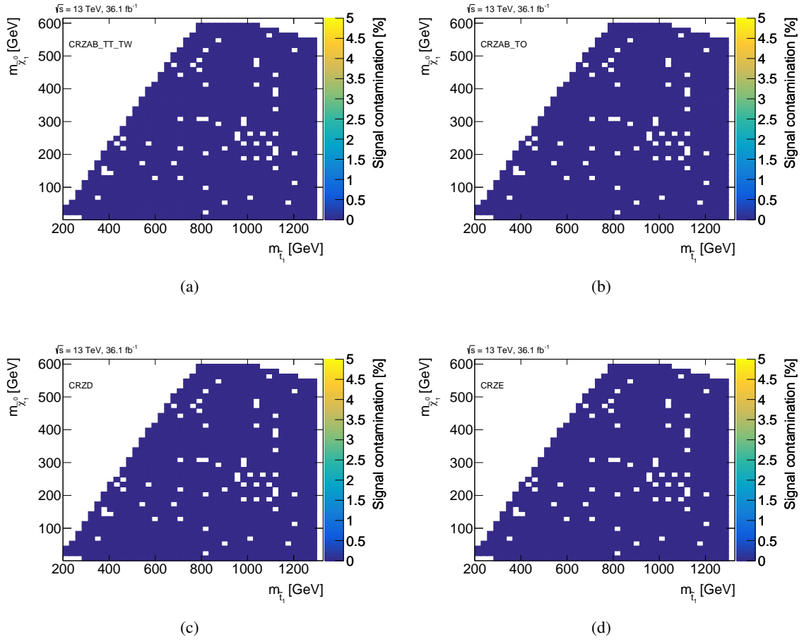
Figure B.16: Expected signal contamination for top squark pair production with \mathcal{BR}(\tilde{t}_1 \rightarrow t + \tilde{\chi}_1^0) = 100\% in the Z+jets CRs.
