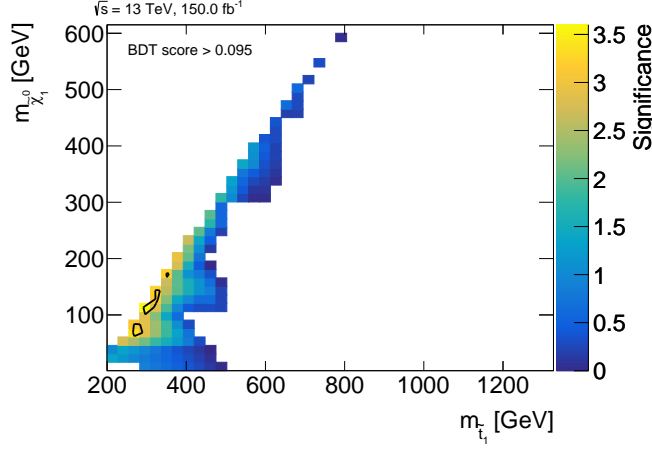
Figure 14.7: Expected significances as a function of m_{\tilde{t}_1} and m_{\tilde{\chi}_1^0} for a signal region based on the preselection summarised in Table 14.3 and a minimum requirement on the score of a BDT of BDT (SRC) score > 0.095 trained on all signal simulations with 173 \text{ GeV} \leq m_{\tilde{t}_1} - m_{\tilde{\chi}_1^0} \leq 188 \text{ GeV} . The results are obtained assuming an integrated luminosity of 150.0 \text{ fb}^{-1} corresponding to the full LHC Run 2 dataset. For the calculation of the expected significances, an uncertainty of 30% on the SM yields are assumed. The solid black line indicates the 3\sigma contour.
