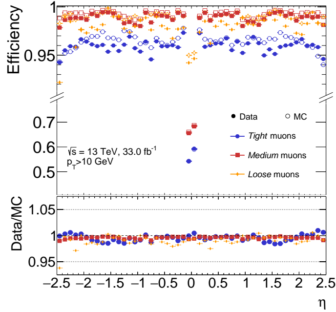
Figure 7.9: Muon reconstruction efficiencies for the Loose/Medium/Tight identification algorithms measured in Z \rightarrow \mu^+ \mu^- events of the 2016 dataset as a function of the muon pseudorapidity for muons with p_T > 10 \text{ GeV} . The prediction by the detector simulation is depicted as open circles, while filled dots indicate the observation in collision data with statistical errors. The bottom panel shows the ratio between expected and observed efficiencies, the efficiency scale factor. The errors in the bottom panel show the quadratic sum of statistical and systematic uncertainty.
