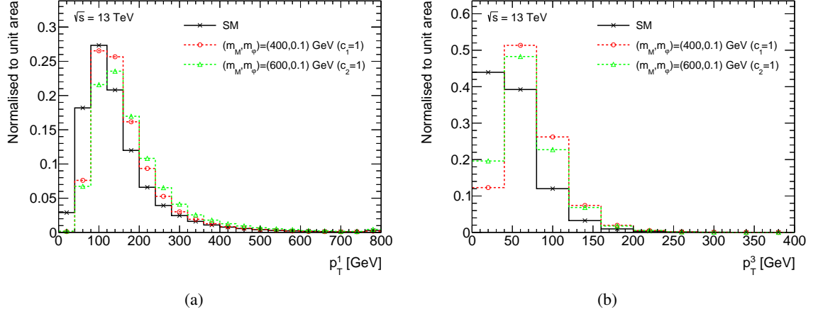
Figure 13.3: Relative distributions of the simulated jet transverse momenta p_T for the second (a) and forth (b) jet leading in p_T after applying a lepton veto as well as at least four jets and one b -jet for the same selection of signal processes shown in Figure 13.2. The distributions of transverse momenta of the other two jets, can be found in Appendix D.1.
