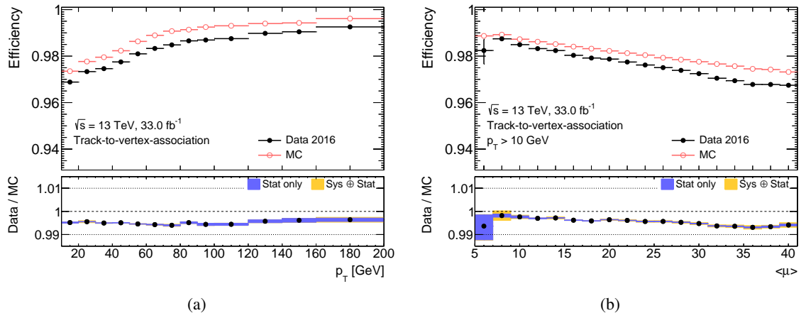
Figure 7.11: Muon track-to-vertex association efficiency measured in Z \rightarrow \mu^+ \mu^- events of the 2016 dataset as a function of the muon transverse momentum (a) and the average number of interactions per bunch crossing (b). The bottom panel shows the ratio between expected and observed efficiencies, the efficiency scale factor.
