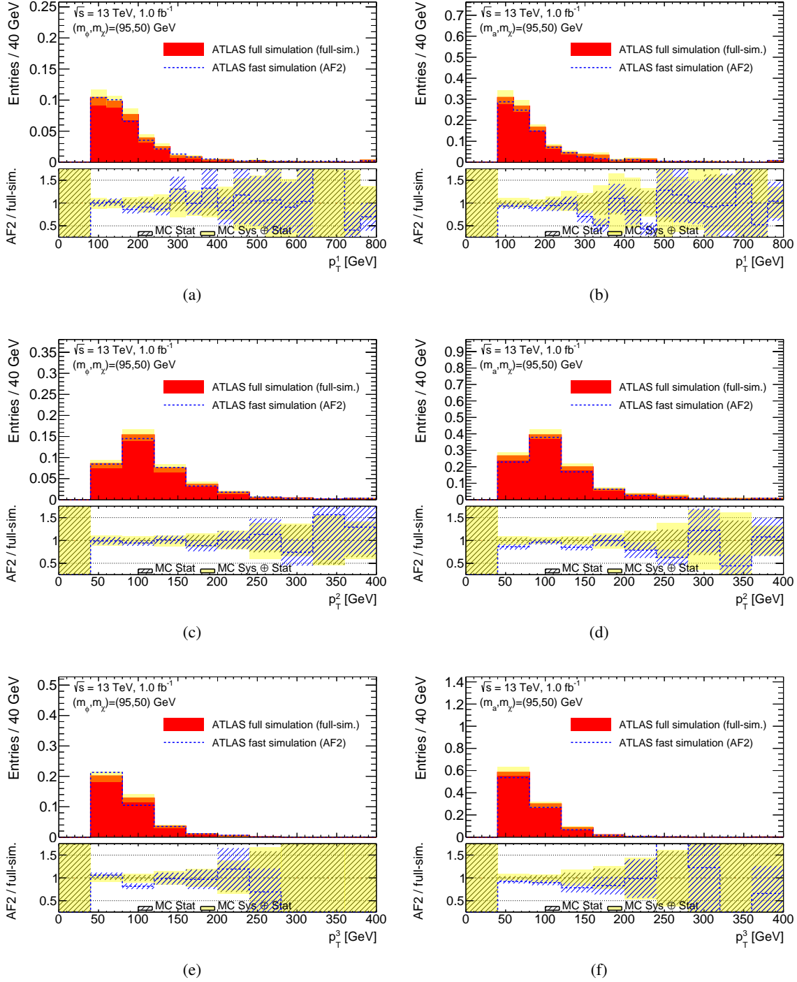
Figure C.2: Comparison between the full ATLAS detector simulation based on GEANT 4 (red) and the fast simulation framework (AF2) for WIMP pair production with m_\chi = 50 GeV and scalar (left) or pseudoscalar (right) mediator with m_{\phi/a} = 95 GeV. The hashed (yellow) bands are indicating the statistical (experimental systematic) uncertainties.
