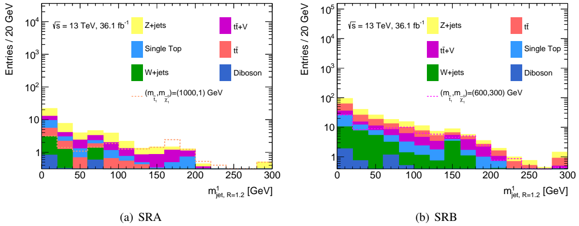
Figure 11.19: Distributions of m_{\text{jet}, R=1.2}^1 in SRA (a) and SRB (b) after applying all requirements listed in Table 11.2 but the one on m_{\text{jet}, R=1.2}^1 scaled to an integrated luminosity of 36.1 \text{ fb}^{-1} without drawing statistical or systematic uncertainty bands. In addition to the SM processes, also simulated top squark pair production with (m_{\tilde{t}_1}, m_{\tilde{\chi}_1^0}) = (1000, 1) \text{ GeV} (a) and (m_{\tilde{t}_1}, m_{\tilde{\chi}_1^0}) = (600, 300) \text{ GeV} (b) are shown, respectively. The rightmost bin includes overflow events.
