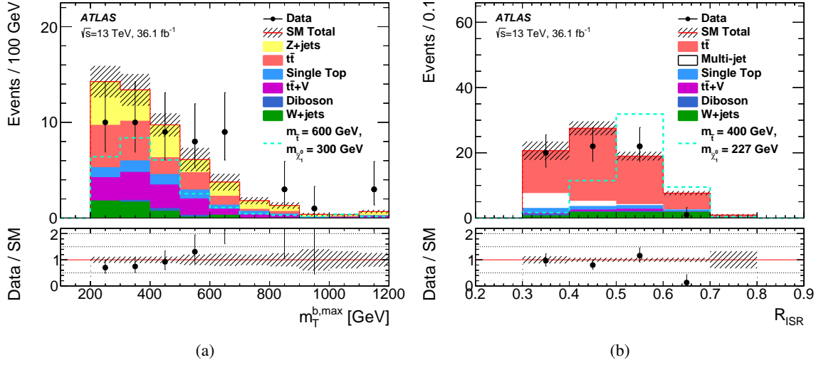
Figure 11.41: Distributions of m_T^{b,max} for SRB-TW (a) and R_{ISR} for SRC1-5 (b) after the likelihood fit is performed. The stacked histograms show the SM prediction and the hatched uncertainty band around the SM prediction shows the MC statistical and detector-related systematic uncertainties. For each variable, the distribution for a representative signal point is shown [288].
