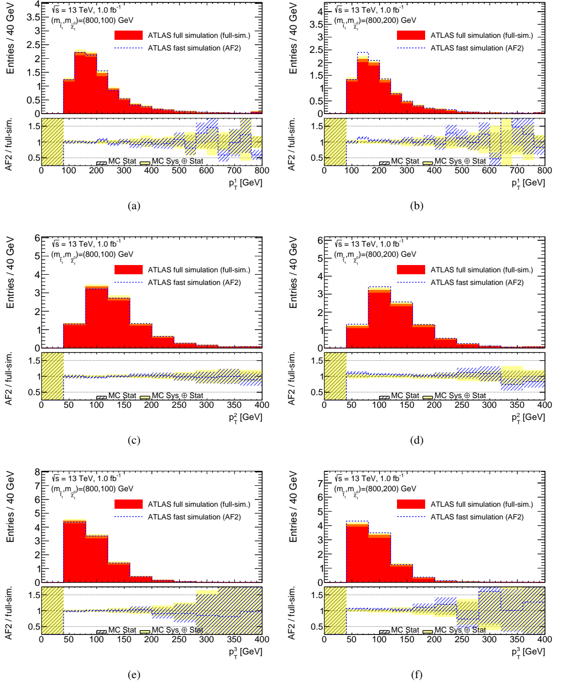
Figure B.3: Comparison between the full ATLAS detector simulation based on GEANT 4 (red) and the fast simulation framework (AF2) for top squark pair production with m_t = 800 GeV and m_{\tilde{\chi}_1^0} = 100 GeV (left) or m_{\tilde{\chi}_1^0} = 200 GeV (right), respectively. The hashed (yellow) bands are indicating the statistical (experimental systematic) uncertainties.
