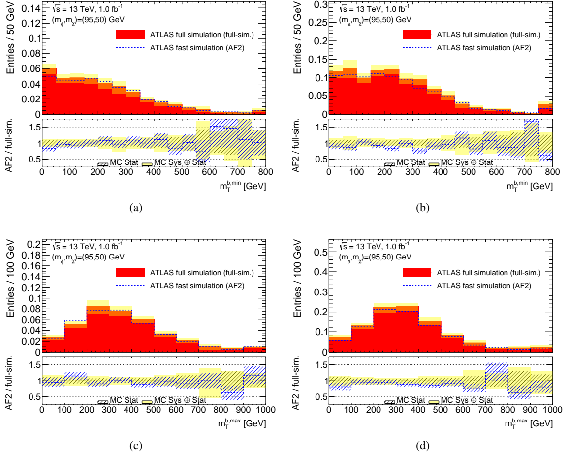
Figure C.3: Comparison between the full ATLAS detector simulation based on GEANT 4 (red) and the fast simulation framework (AF2) for WIMP pair production with m_\chi = 50 GeV and scalar (left) or pseudoscalar (right) mediator with m_{\phi/a} = 95 GeV. The hashed (yellow) bands are indicating the statistical (experimental systematic) uncertainties.
