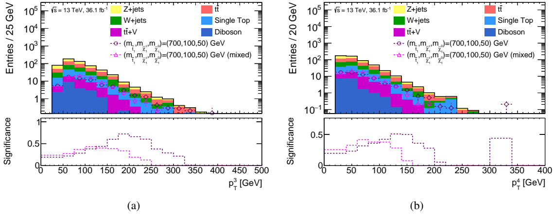
Figure 11.28: Simulated distributions of p_T^3 (a) and p_T^4 (b) after requiring the presence of at least two b -jets, m_T^{b, \min} > 200 GeV and p_T^1 > 150 GeV in addition to the basic requirements summarised in Table 11.1. The bottom panel shows the expected significance for the signal scenario with (m_{\tilde{t}_1}, m_{\tilde{\chi}_1^\pm}, m_{\tilde{\chi}_1^0}) = (700, 100, 50) GeV depending on a potential cut value on the corresponding variable.
