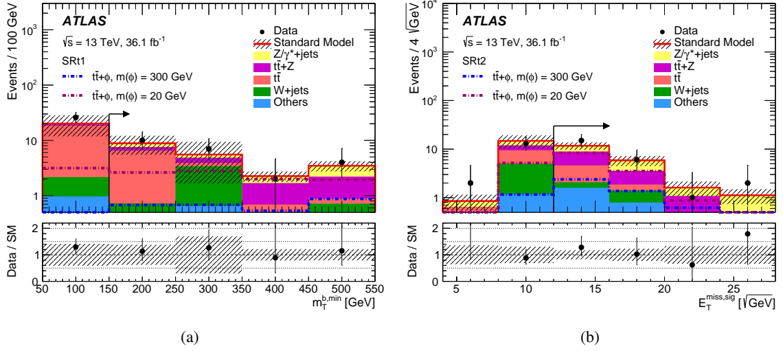
Figure 12.15: Comparison of the data with the post-fit SM prediction of the m_T^{b,min} distribution in SRt1 (a) and the E_T^{miss}/\sqrt{H_T} distribution in SRt2 (b). The last bins include overflows, where applicable. All signal region requirements except the one on the distribution shown are applied. The signal region requirement on the distribution shown is indicated by an arrow. The bottom panel shows the ratio of the data to the prediction. The uncertainty band includes all systematic and statistical uncertainties [330].
