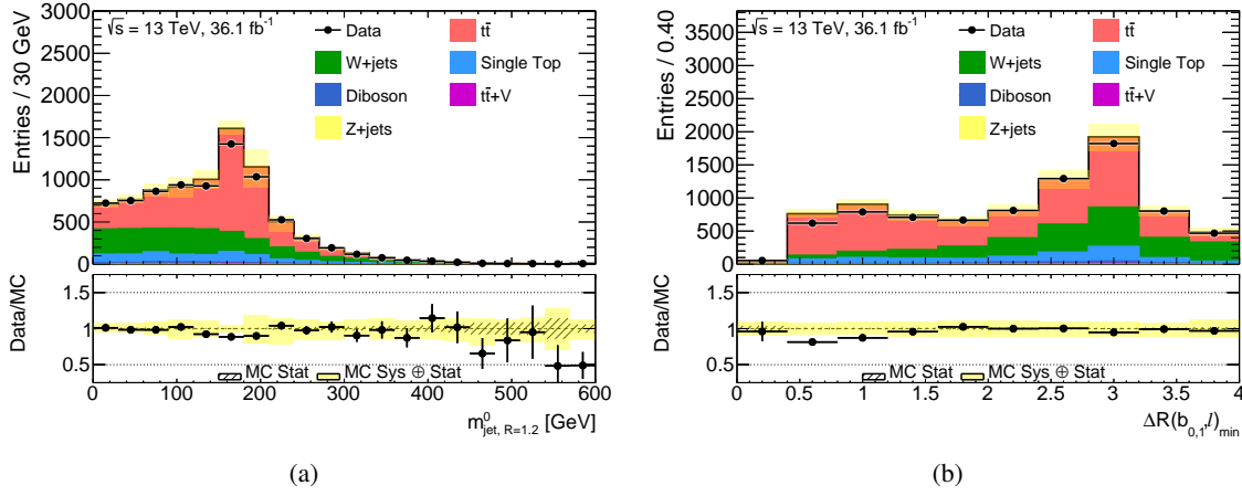
Figure 11.35: Distributions of m_{\text{jet}, R=1.2}^0 (a) and \Delta R(b_{0,1}, \ell)_{\min} (b) scaled to an integrated luminosity of 36.1 \text{ fb}^{-1} after requiring one charged lepton and all basic requirements listed in Table 11.1 except for E_{\text{T}}^{\text{miss, track}} and |\Delta\phi(E_{\text{T}}^{\text{miss}}, E_{\text{T}}^{\text{miss, track}})| . The yellow bands show the quadratic sum of the statistical and experimental systematic uncertainties.
