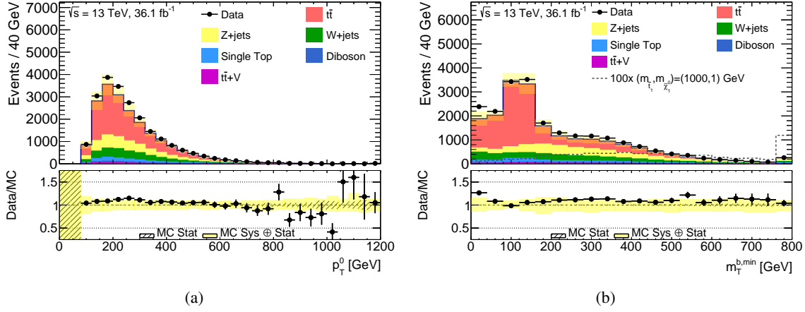
Figure 11.10: Distributions of the transverse momentum of the highest- p_T jet, p_T^0 (a), and m_T^{b,min} (b) after the common preselection summarised in Table 11.1. The stacked histograms show the SM prediction before being normalised using normalisation factors derived from a simultaneous fit (detailed in Section 11.6) to all dominant SM backgrounds. The lower panels show the ratio of data events to the total SM prediction. The rightmost bin includes overflow events. The yellow bands show the quadratic sum of the statistical and experimental systematic uncertainties.
