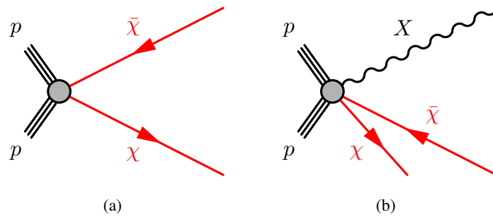
Figure 12.1: Sketch of WIMP pair production with no other SM particle (a) and with associated production of a SM particle X (b) at the LHC.
