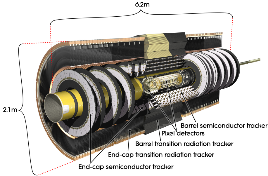
Figure 5.2: The ATLAS Inner Detector [153].
