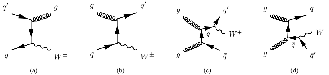
Figure 9.2: Selection of Feynman graphs for W + jets production at the LHC.
