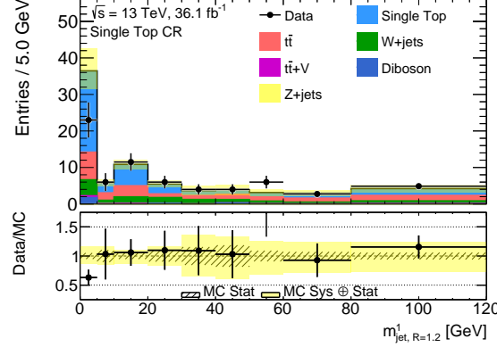
Figure 11.40: Distribution of m_{\text{jet}, R=1.2}^1 in the CR for single top quark production. The majority of the single top quark contribution satisfies m_{\text{jet}, R=1.2}^1 < 60 GeV which corresponds to the R = 1.2 reclustered jet category T0. The yellow band shows the quadratic sum of the statistical and the experimental systematic uncertainties.
