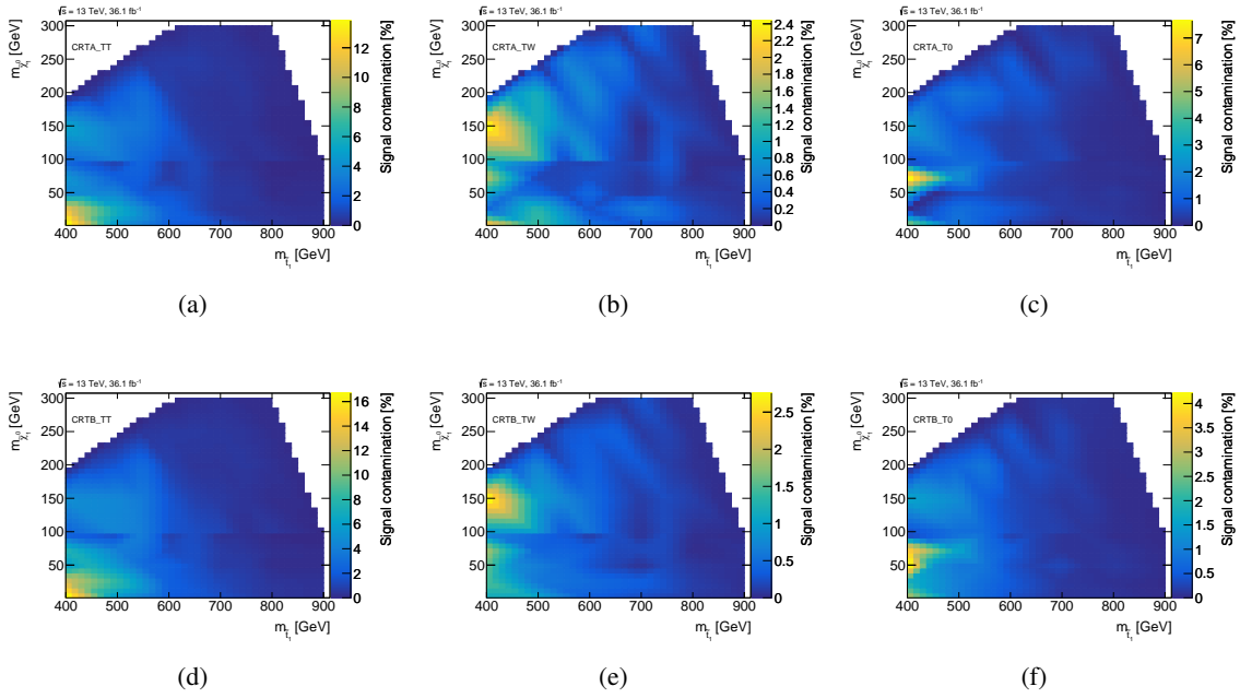
Figure B.22: Expected signal contamination for top squark pair production with \mathcal{BR}(\tilde{t}_1 \rightarrow b + \tilde{\chi}_1^+) = 100\% in the \tilde{t}\tilde{t} CRs targeting SRA and SRB.
