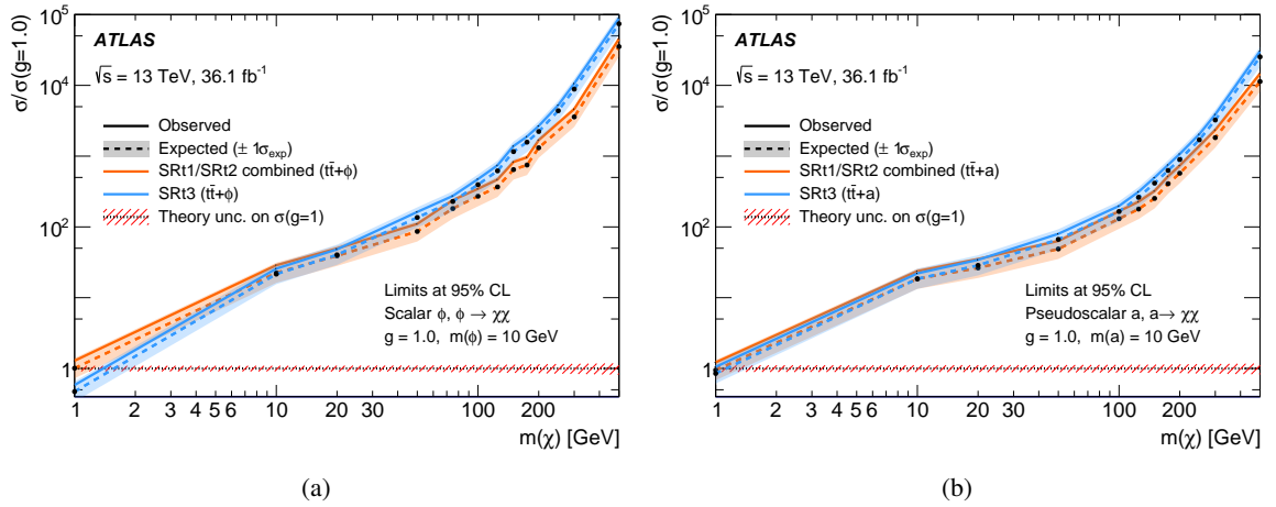
Figure 12.16: Exclusion limits for t\bar{t} + \phi (a) and t\bar{t} + a (b) models as a function of the WIMP mass for a mediator mass of 10 GeV. The limits are calculated at 95% CL and are expressed in terms of the ratio of the excluded cross section to the nominal cross section for a coupling assumption of g = g_t = g_\chi = 1 . The solid (dashed) lines show the observed (expected) exclusion limits for the different SRs according to the colour code specified in the legend. To derive the results for the fully hadronic t\bar{t} final state the region SRt1 or SRt2 providing the better expected sensitivity is used [330].
