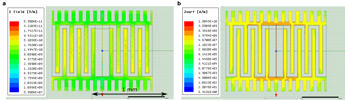
Figure 5.9 – HFSS simulation of resonator 2 on sample A. a. Electric field in logarithmic scale with 1 Joule applied in the resonator mode. b. Surficial current in logarithmic scale with 1 Joule applied in the resonator mode.
