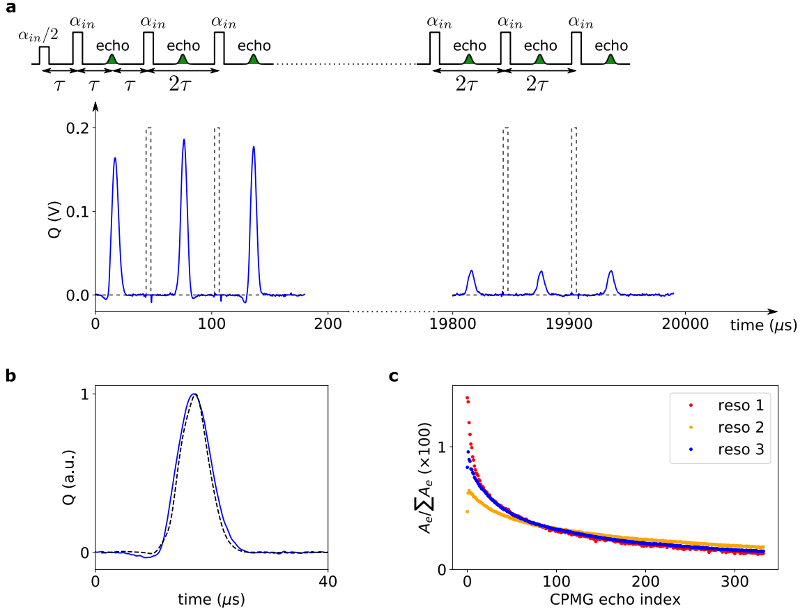
Figure 8.4 – CPMG echoes. a. Top. Sketch of a Hahn-echo sequence followed after a delay \tau by a CPMG sequence consisting in a series of N pulses of same amplitude and duration as the refocusing pulse of the Hahn-echo sequence. The CPMG pulses are spaced by 2\tau and an echo forms at time \tau after each CPMG pulse. Bottom. Hahn-echo followed by N = 332 CPMG echoes recorded at high pulse power on the Q quadrature with resonator 3 of sample A, at \varphi = 30^\circ (solid blue line). The CPMG control pulses sent by the AWG, of duration dt = 4 \mu\text{s} and separation 2\tau = 60 \mu\text{s} , are shown in a dashed grey line. The sequence is repeated every 4 s and averaged 300 times. The x -axis is cut to show only the three first and last echoes. The total sequence lasts about 20 ms. b. Hahn-echo (blue, same data as the first echo of subplot a) superposed with the CPMG averaged echo (black dashed line). The latter is computed as the weighted average of all N + 1 echoes where the weights are the normalized integral of each echo. c. Normalized integrated echo A_e / \sum A_e as a function of its index in the CPMG sequence for all three resonators. These data, measured at high pulse power, are used as the weights for the CPMG averaging in all further experiments with CPMG signal enhancement.
