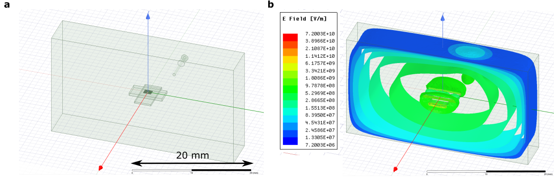
Figure 5.8 – HFSS simulation. a. Drawing in HFSS showing the rectangular metallic box (of dimensions 33 \times 19 \times 6 mm 3 ), the metallic antenna and the silicon chip which holds the CaWO 4 sample where one resonator is patterned. b. Electric field in logarithmic scale with 1 Joule applied in the box fundamental mode.
