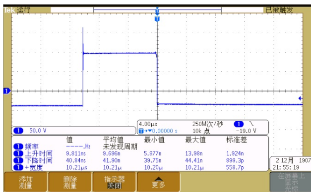
Figure 8: Parament of the pulse-forming circuit.
