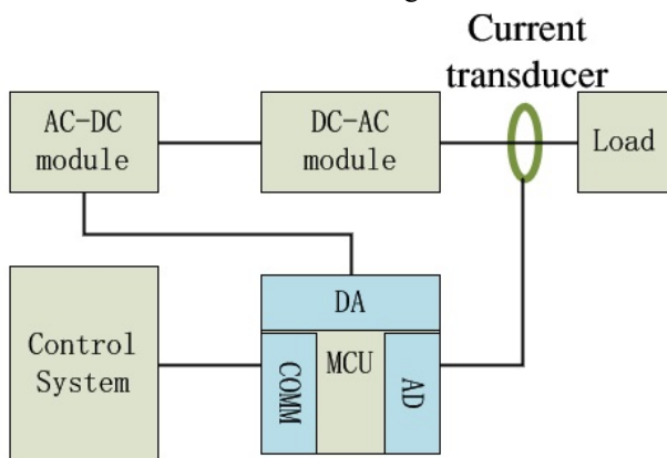
Figure 10: Conceptual of the DC-AC inverter.
