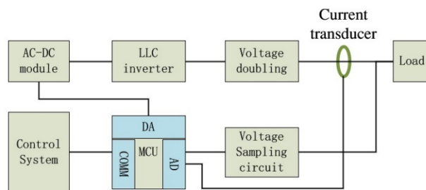
Figure 11: Conceptual of high voltage PS.
