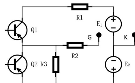
Figure 7: MOSFET coupling circuit.
