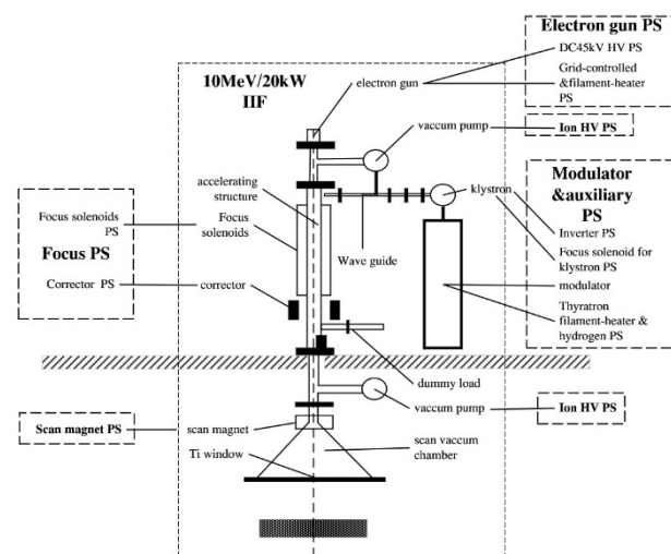
Figure 1: Power supply system of the IIF.
