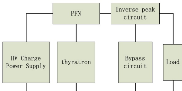
Figure 9: Linear modulator.
