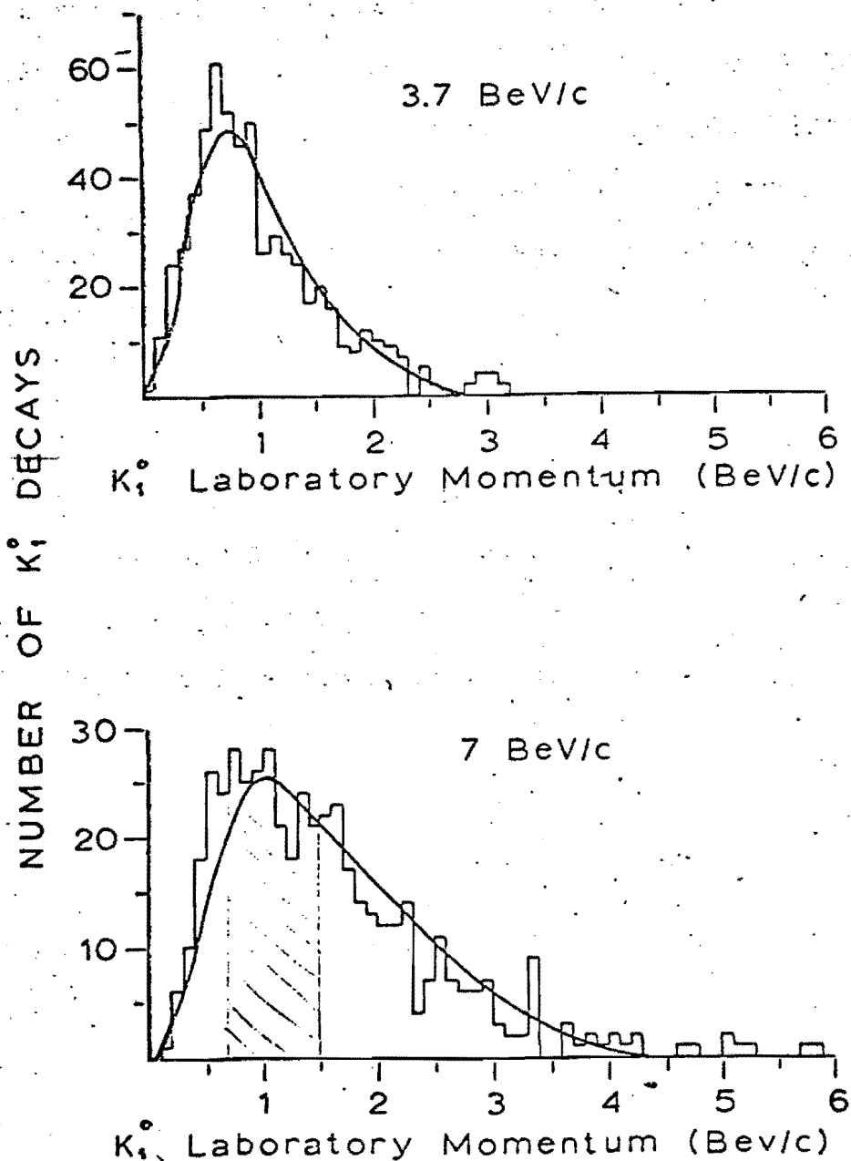
Figure 19. Laboratory momentum spectra of K_1^0 -particles produced at 3.7 and 7 BeV/c. The smooth curves represent statistical model expectations on the basis of 6-body final state for 3.7 BeV/c and 7-body final state for 7 BeV/c.
