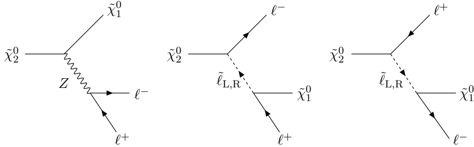
Fig. 1. Diagrams contributing to the leptonic three-body neutralino decay \tilde{\chi}_2^0 \rightarrow \tilde{\chi}_1^0 \ell^+ \ell^- .
