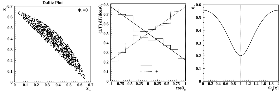
Fig. 3. Left: the Dalitz plot for the neutralino \tilde{\chi}_2^0 decay in the (x_-, x_+) Dalitz plane. Middle: the normalized lepton angle distribution (19); the solid line is for the negative charge lepton and the dotted line for the positive charge lepton. Right: the \Phi_1 dependence of the slope parameter \eta_- for the parameter set (14).
