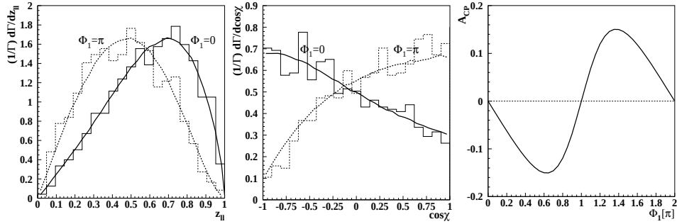
Fig. 4. The lepton invariant mass distribution (left panel) and the opening angle distribution (middle panel) in the three-body leptonic neutralino decay. The solid lines are for \Phi_1 = 0 , (when neutralinos have the same CP parities) and the dotted lines for \Phi_1 = \pi , (when neutralinos have the opposite CP parities). The right panel: the \Phi_1 dependence of the CP-odd and CPT-even asymmetry A_{CP} of the triple scalar product for the parameter set (14).
