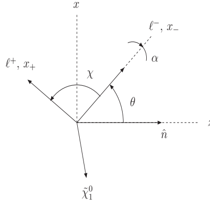
Fig. 2. Kinematic configuration of momenta and the spin vector in the neutralino \tilde{\chi}_2^0 rest frame.
