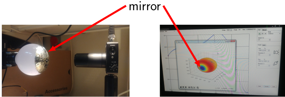
Figure 4: Far scan result. The test was performed with a mirror on the top to improve the isotropy in a backward region. Right: The scanner control interface with scan visualization.
